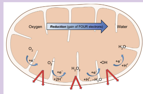
Fig 3. Oxygen is fully reduced to water by gaining four electrons (blue arrows) in the mitochondrial respiratory chain (top line). Incomplete oxygen reduction results in the production of the reactive intermediates superoxide (O 2 •− ), hydrogen peroxide (H 2 O 2 ), and hydroxyl radicals (•OH), respectively. These intermediates can go on to react with other cell constituents (red arrows) such as metal ions (e.g. Fe 2+ in haemoproteins), thiols (e.g. glutathione) or compounds in the cell nucleus (e.g. DNA).
