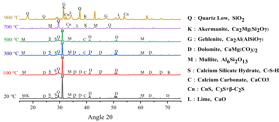
Fig. 6. XRD graphs of geopolymers (S0CA0) after exposed to elevated temperatures.
