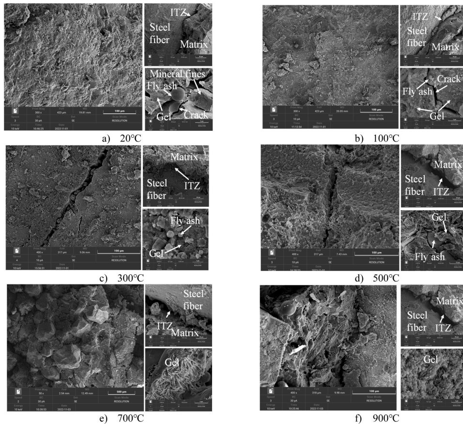
Fig. 7. SEM images of geopolymers (S2CA30) after exposed to elevated temperatures.
