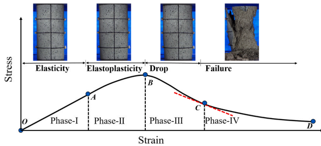
Fig. 14. Typical axial compression stress-strain curve.
