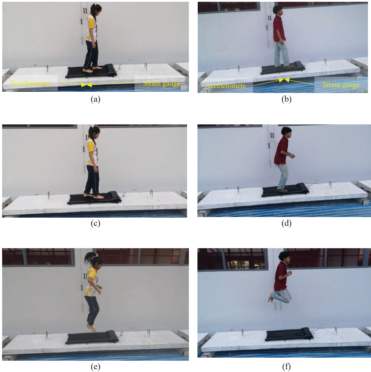
Fig. D1. Setup of human-induced vibration tests to measure vertical acceleration in 100% RCA composite metal deck slab (a) female normal walking, (b) male normal walking, (c) female brisk walking, (d) male brisk walking, (e) female jumping, and (f), male jumping.
