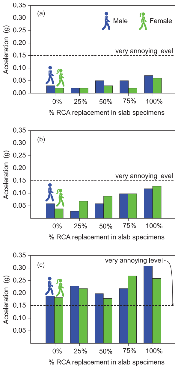
Fig 10. Maximum acceleration of slabs subjected to (a) normal walking, (b) brisk walking, and (c) jumping.
