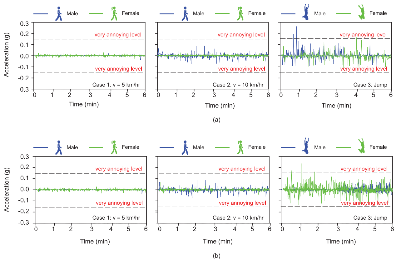
Fig. A1. Accelerations results of slab for normal walking, brisk walking, and jumping for RCA0% (a) and RCA100% (b).
