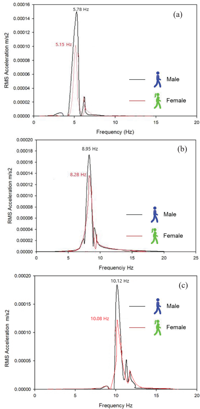
Fig 11. Frequency response of slab RCA100% slab for (a) normal walking, (b) brisk walking, and (c) jumping.
