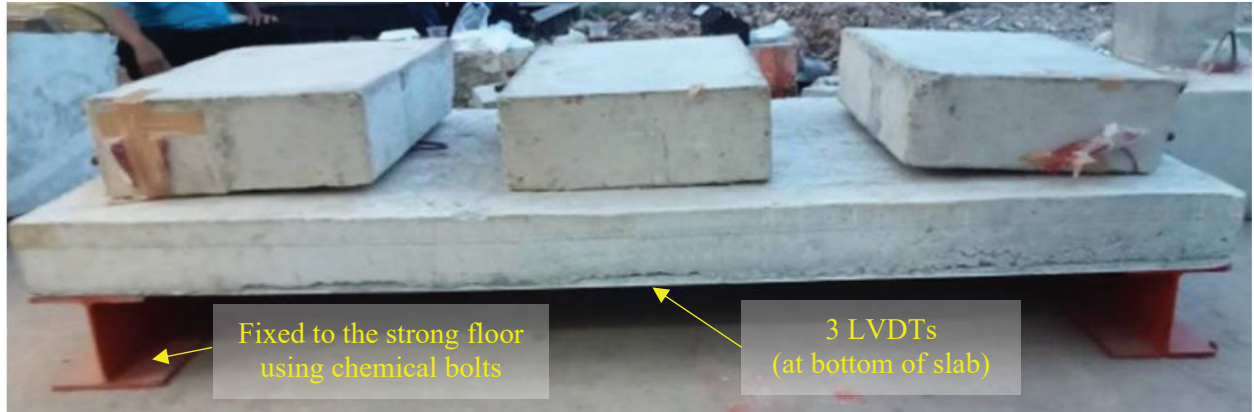
Fig 5. Typical experimental setup for sustainable loading tests.
