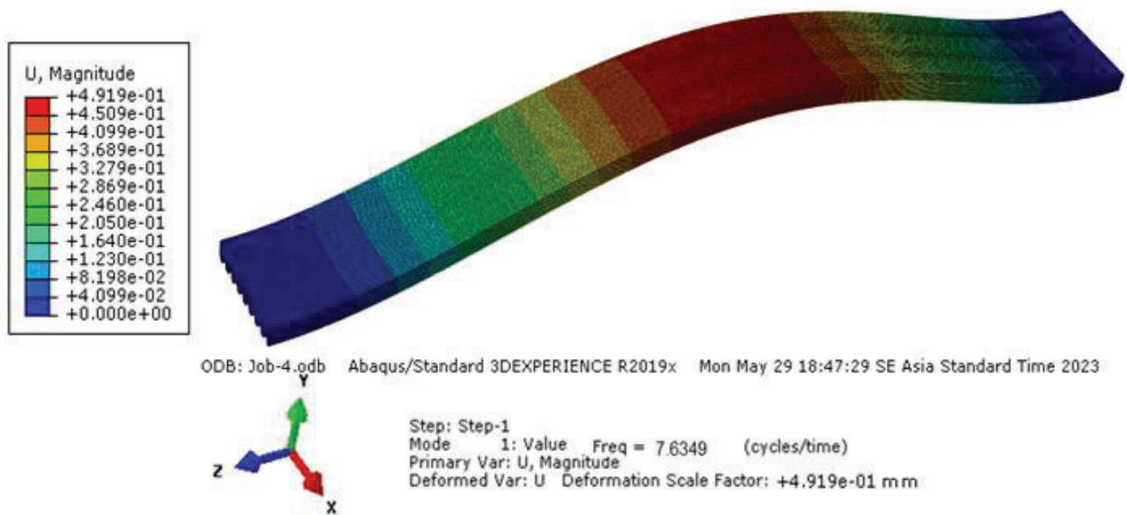
Fig. C4. Mode shape Frequency response of slab RCA100% slab for Model 4
