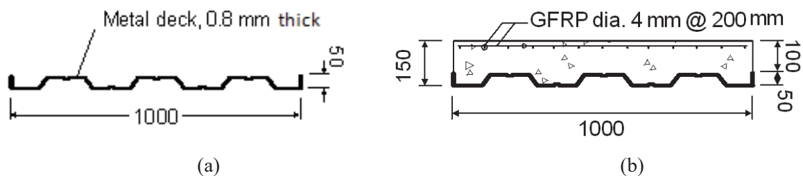
Fig 1. Schematic view of (a) metal deck, and (b) cross section of concrete slab-deck system (units: mm).
