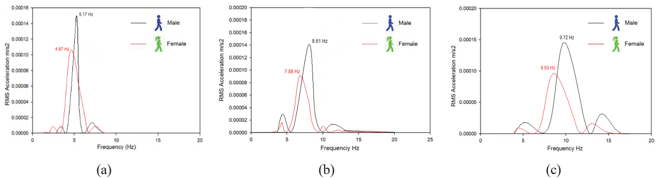
Fig. B3. Frequency response of slab RCA50% slab for (a) normal walking, (b) brisk walking, and (c) jumping.
