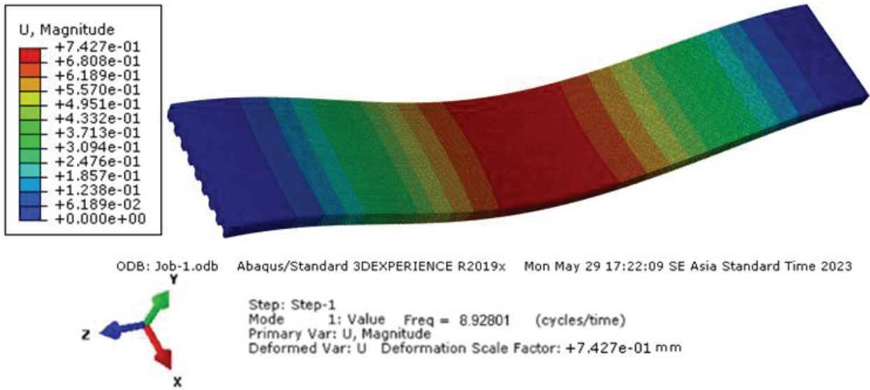
Fig. C1. Mode shape Frequency response of slab RCA100% slab for Model 1
