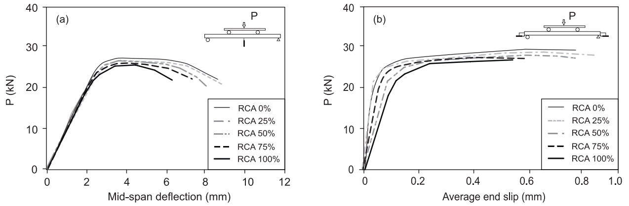
Fig 8. Results from slabs with different levels of RCA: (a) load vs mid-span deflection curves, and (b) load vs end slips.
