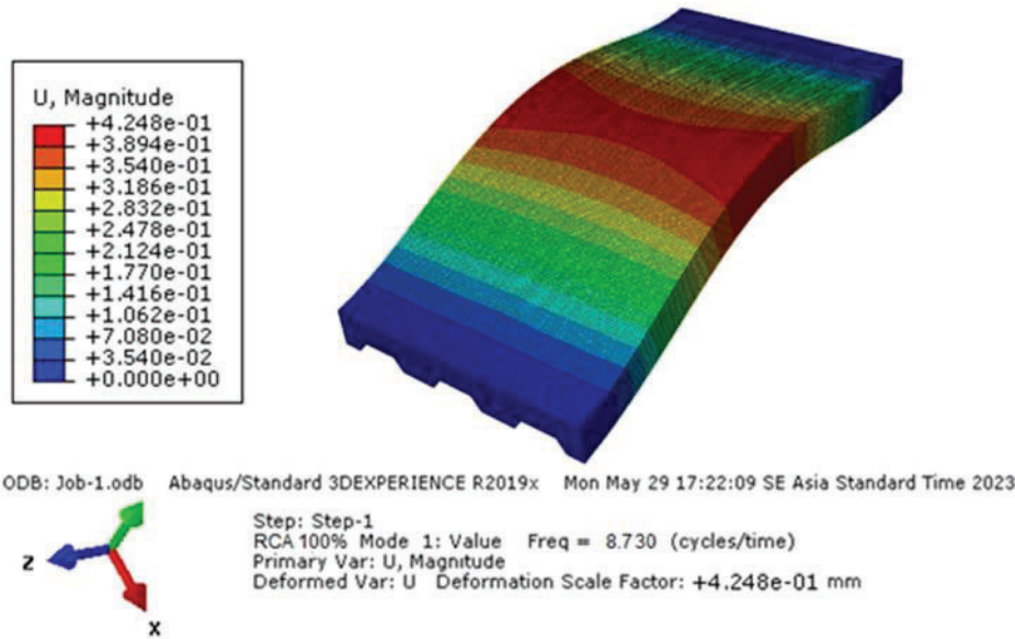
Fig 15. Modal shape of RCA100% slab with f_l=8.73 Hz.
