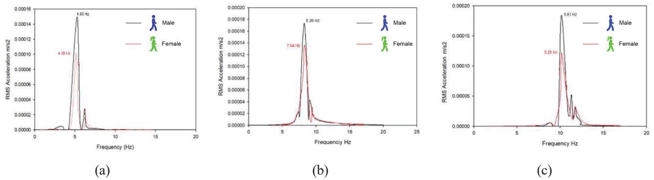
Fig. B2. Frequency response of slab RCA25% slab for (a) normal walking, (b) brisk walking, and (c) jumping.
