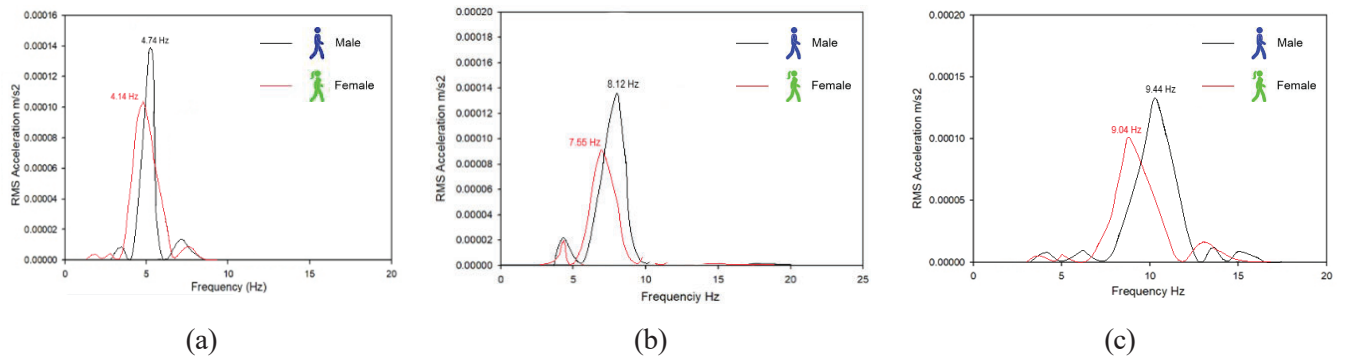
Fig. B1. Frequency response of slab RCA0% slab for (a) normal walking, (b) brisk walking, and (c) jumping.
