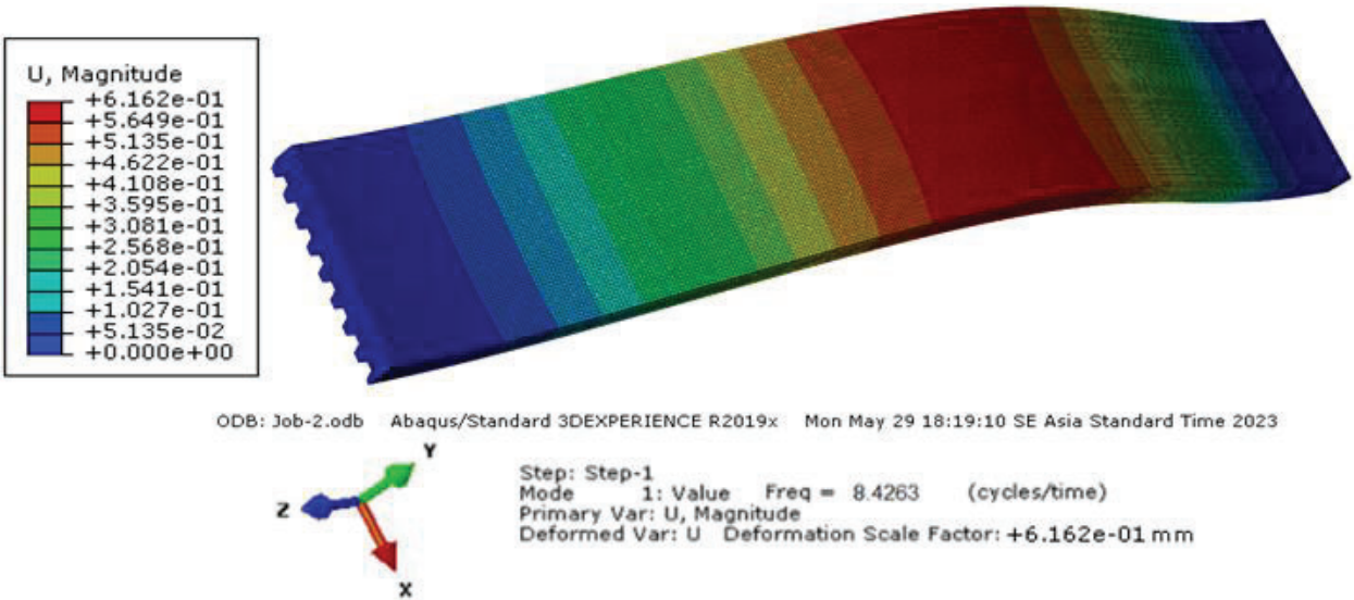
Fig. C2. Mode shape Frequency response of slab RCA100% slab for Model 2
