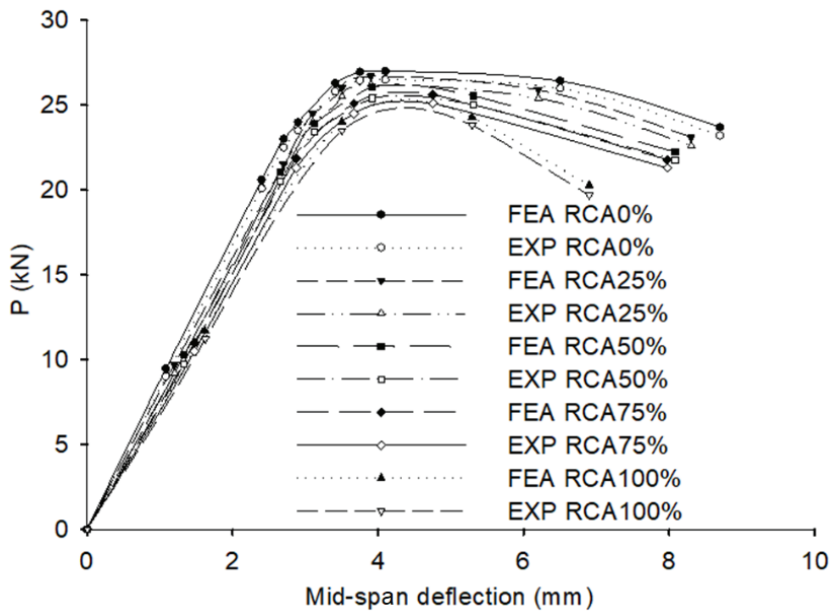
Fig 14. Comparison of experimental deflections and predicted values obtained from finite element analysis.
