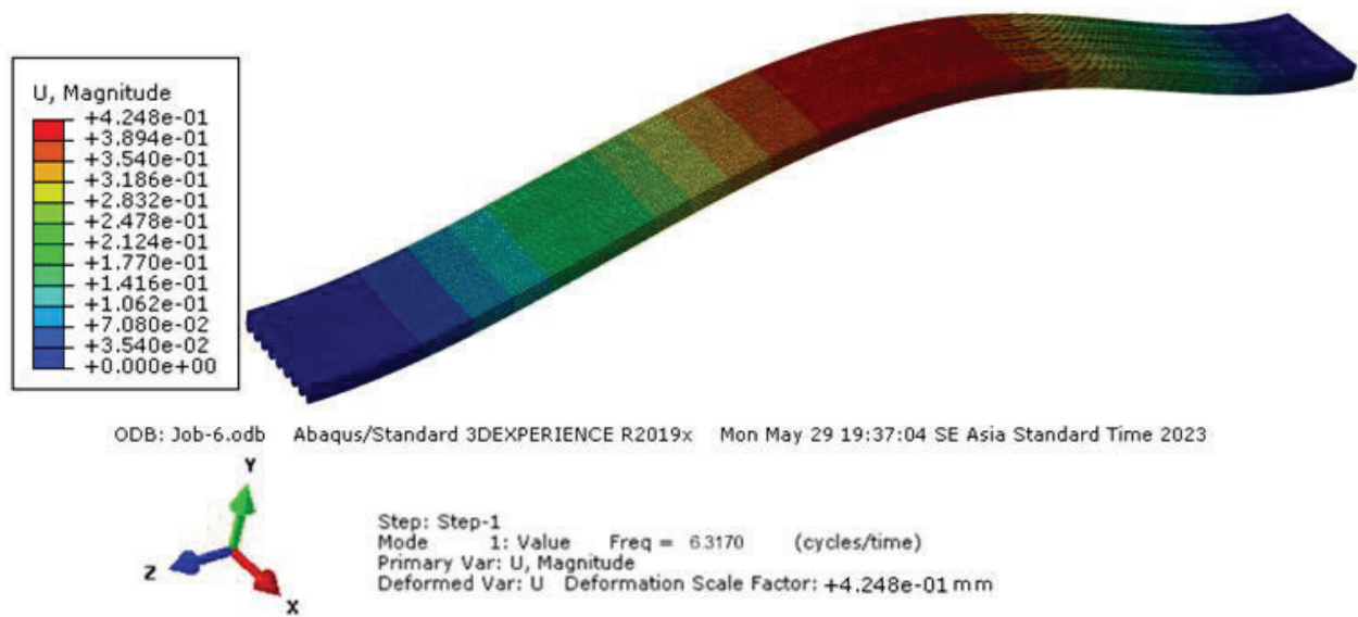
Fig. C6. Mode shape Frequency response of slab RCA100% slab for Model 6
