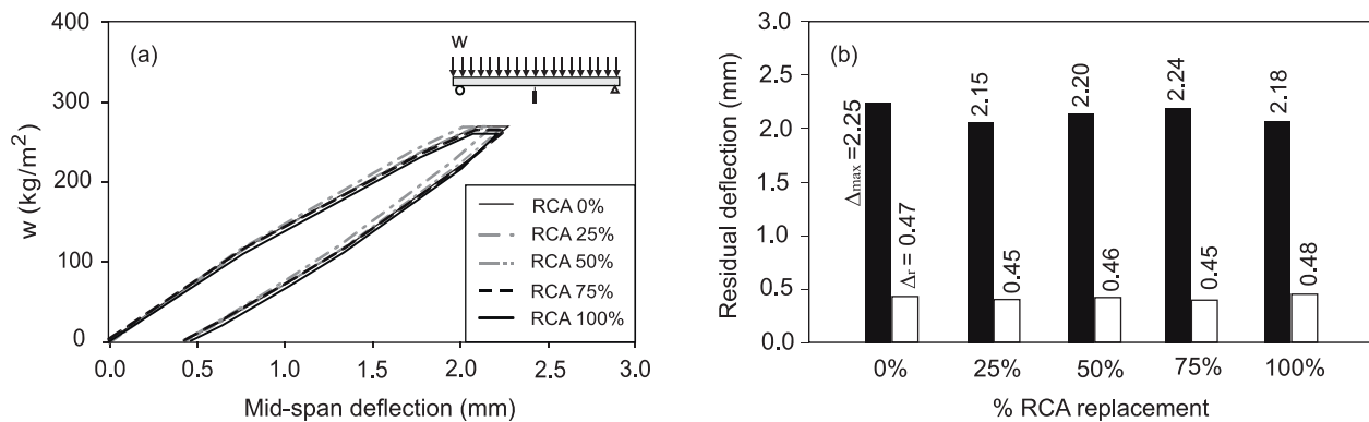
Fig 9. Results from 90 day sustained loading tests: (a) load vs mid-span deflection, and (b) mid-span residual deflection.
