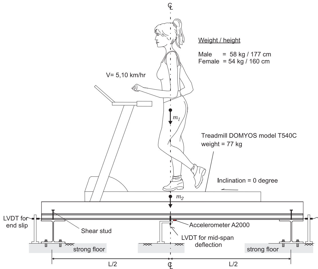
Fig 6. Setup of human-induced vibration tests and position of a treadmill on the tested slab.
