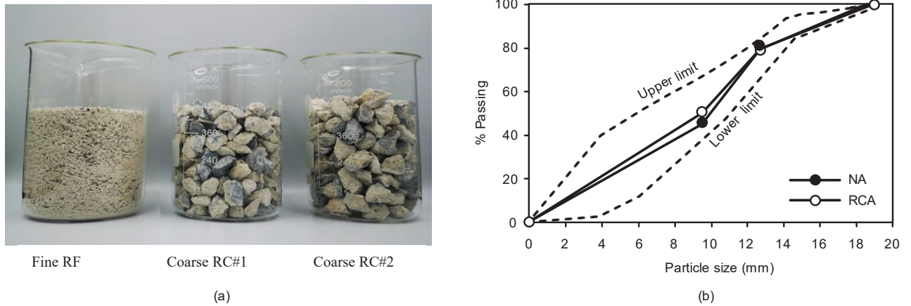
Fig 3. (a) Coarse and fine RCA, and (b) size distribution of natural aggregate and RCA
