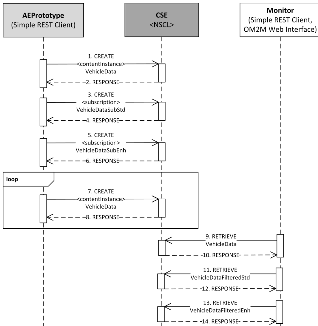
Figure 7.7: Sequence Diagram of Experiment Execution and Result Retrieve
