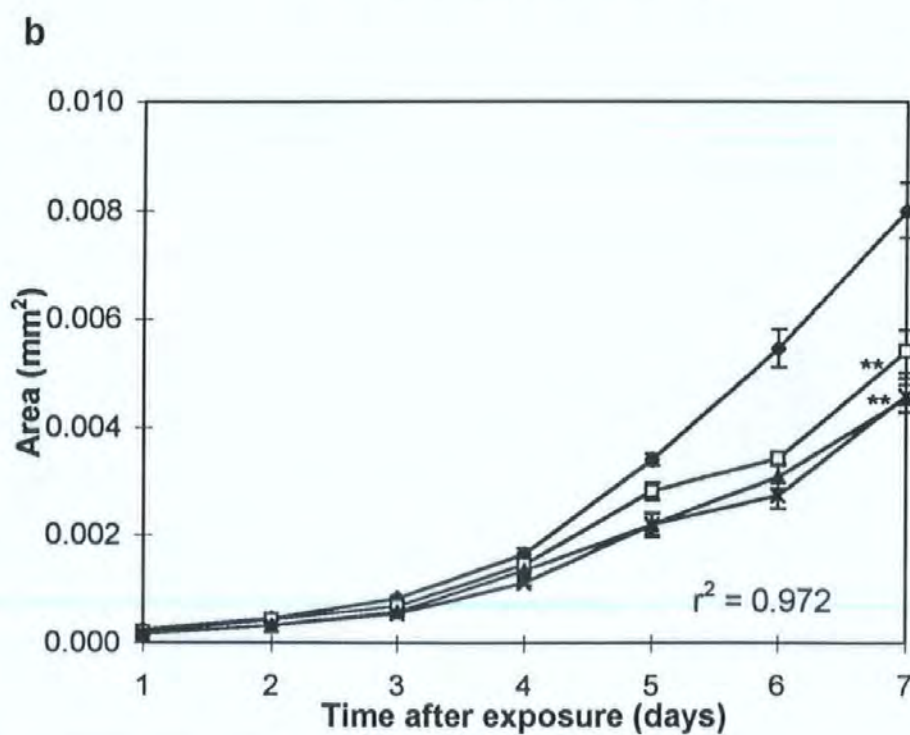
Figure 6.3 Growth of gametophytes (a) and sporophytes (b) measured as increase in area as a function of time after exposure to varying UV irradiances. Multiple regressions were performed on log transformed data, r^2 values are shown for the fitted linear models. ** indicate significant differences in the slopes compared to the control, p < 0.01 . 15 germlings were measured per replicate, mean \pm SE, n = 5 .
