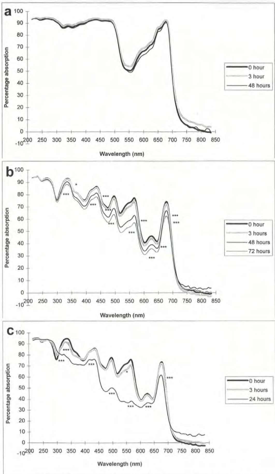
Fig. 3.5 Enteromorpha intestinalis a) and Palmaria palmata b, c). Average in vivo absorptance spectra, before, and after initial 3 h exposure to 2.6 \text{W m}^{-2} (unweighted UV-B irradiance) (a, b); and before and after initial 3 h exposure to 9.0 \text{W m}^{-2} (c). (*, **, *** significant differences between absorptance maxima before and after exposure at p < 0.05 , p < 0.01 ; p < 0.001 , respectively; n = 5 ).
