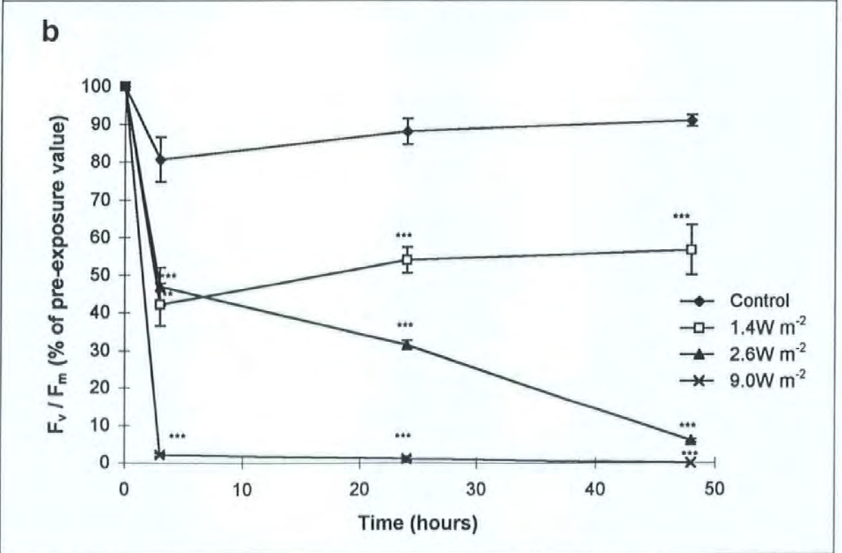
Figure 3.3 Enteromorpha intestinalis a) and Palmaria palmata b). F_v / F_m as a function of time after exposure to different UV-B irradiances; exposure time for all UV-B irradiances was 3 h; data are means \pm SE (n = 5). *** significant differences between UV-B-treated thalli and control thalli at p < 0.001 ; overall significant time-treatment interaction ( p < 0.001 ) was found for both species.
