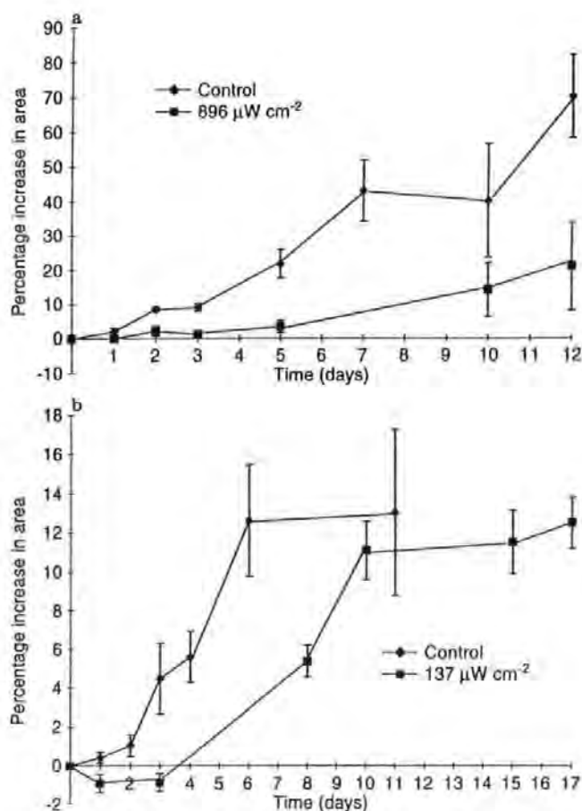
Fig. 5 Enteromorpha intestinalis (a) and Palmaria palmata (b). Growth of mature thalli calculated as percentage area increase from Day 0 measured over 12 and 17 d periods after initial 3 h exposure to 896 or 137 \mu\text{W cm}^{-2} , respectively. Data are means \pm SE ( n = 5 )
