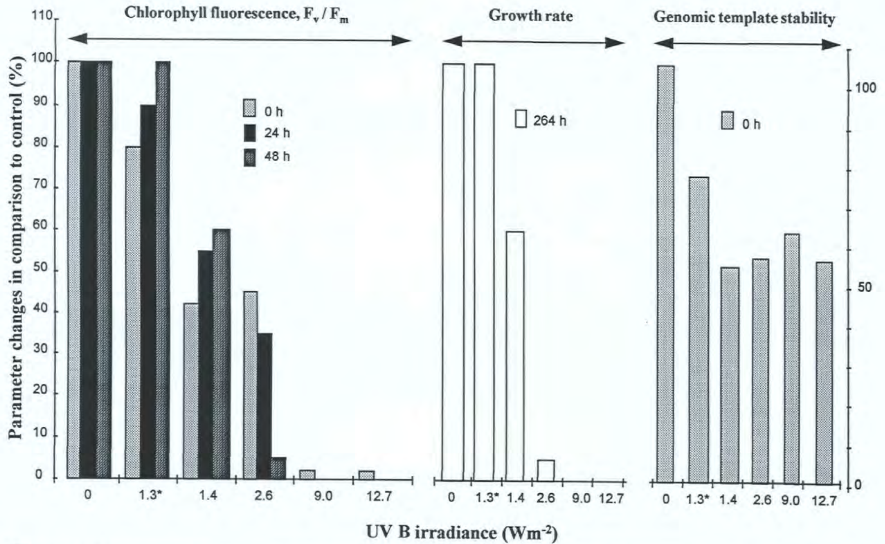
Figure 5.3. Comparison between chlorophyll fluorescence, F_v/F_m ratio, growth rate, and genomic template stability in populations of Palmaria palmata exposed to UV radiation. * indicate that the algae were irradiated with UV-A only.
