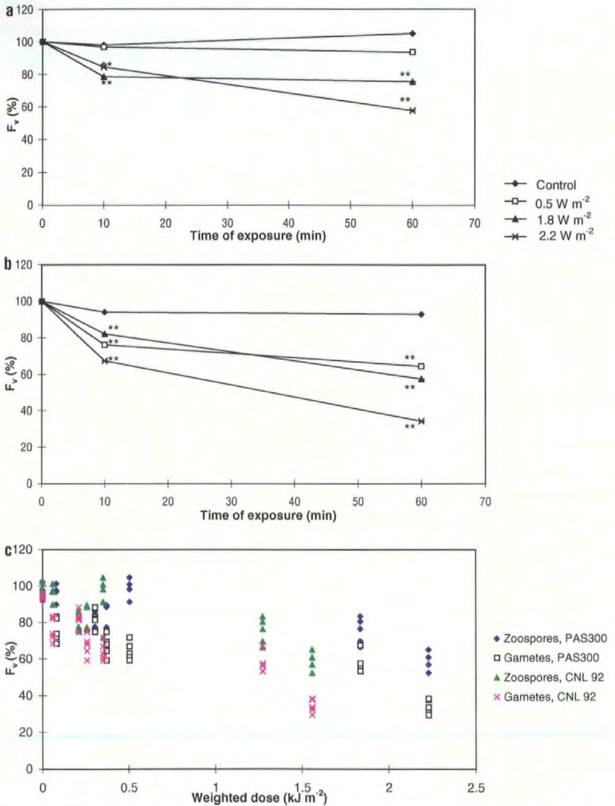
Figure 6.1. Chlorophyll fluorescence F_v (% of pre-exposure value) as a function of exposure time to varying UV-B irradiances in zoospores (a) and gametes (b) of the seaweed species E. intestinalis . Mean \pm SE ( n = 5 ), (** indicate significant differences from control levels, one-way ANOVA, p < 0.01 ). (c) F_v (%) as a function of PAS 300 weighted doses (Caldwell 1971) and CNL 92 phytoplankton weighted doses (Cullen et al. 1992). Data were derived from Fig 6.1a and b. Each point represents a replicate ( n = 5 ). Each replicate in the three panels contained 2.9 \times 10^8 cells per ml.
