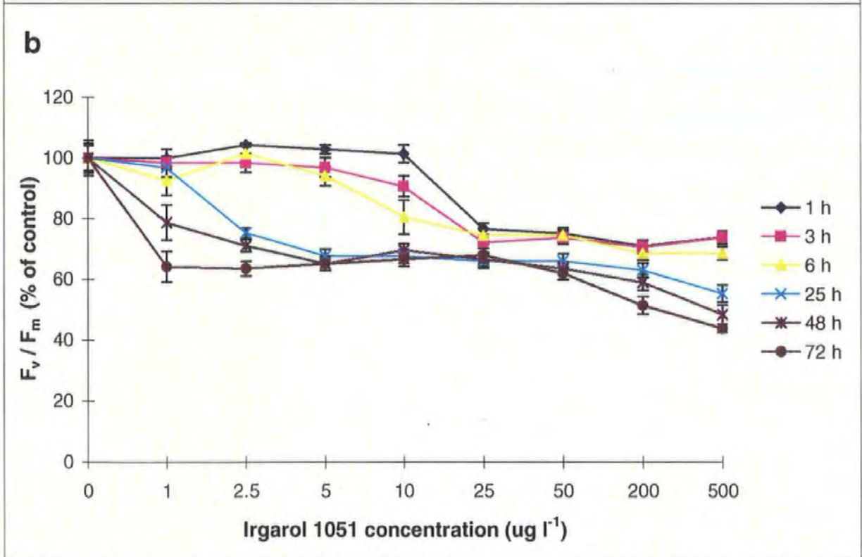
Figure 8.2. Dose-response curves for a) Palmaria palmata and b) Porphyra umbilicalis showing the effect of varying concentrations of Irgarol 1051 on F_v / F_m ratio in mature thalli incubated in Irgarol 1051 solutions at different time periods. Means \pm SE, n = 6.
