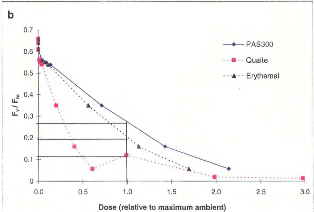
Figure 3.4. Response of F_v/F_m ratio in Palmaria palmata at increasing UV-B dose expressed as a) absolute doses of several weighting functions and b) doses relative to the maximum July dose in Plymouth for Caldwell's generalised plant response spectrum (PAS300), Quaite or the Erythemal action spectrum. Data are from Figure 3.2b.
