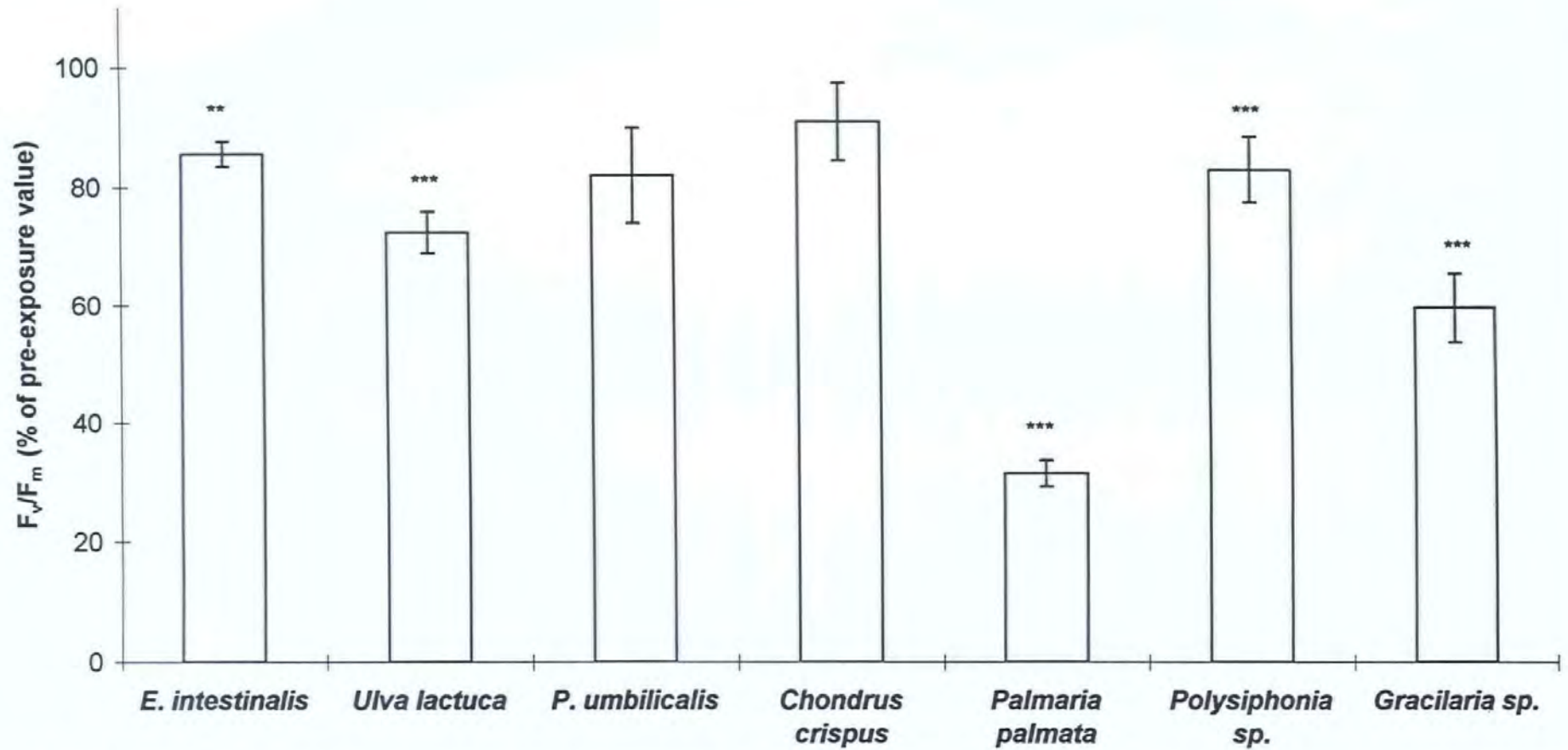
Figure 3.1. Chlorophyll fluorescence F_v/F_m ratio in several species of macroalgae from different tidal heights (Chlorophyta and Rhodophyta) following a 3 hr exposure to unweighted UV-B irradiance of 1.7 \text{ W m}^{-2} . Means \pm SE, n = 5 . **, ***; p < 0.01 , p < 0.0001
