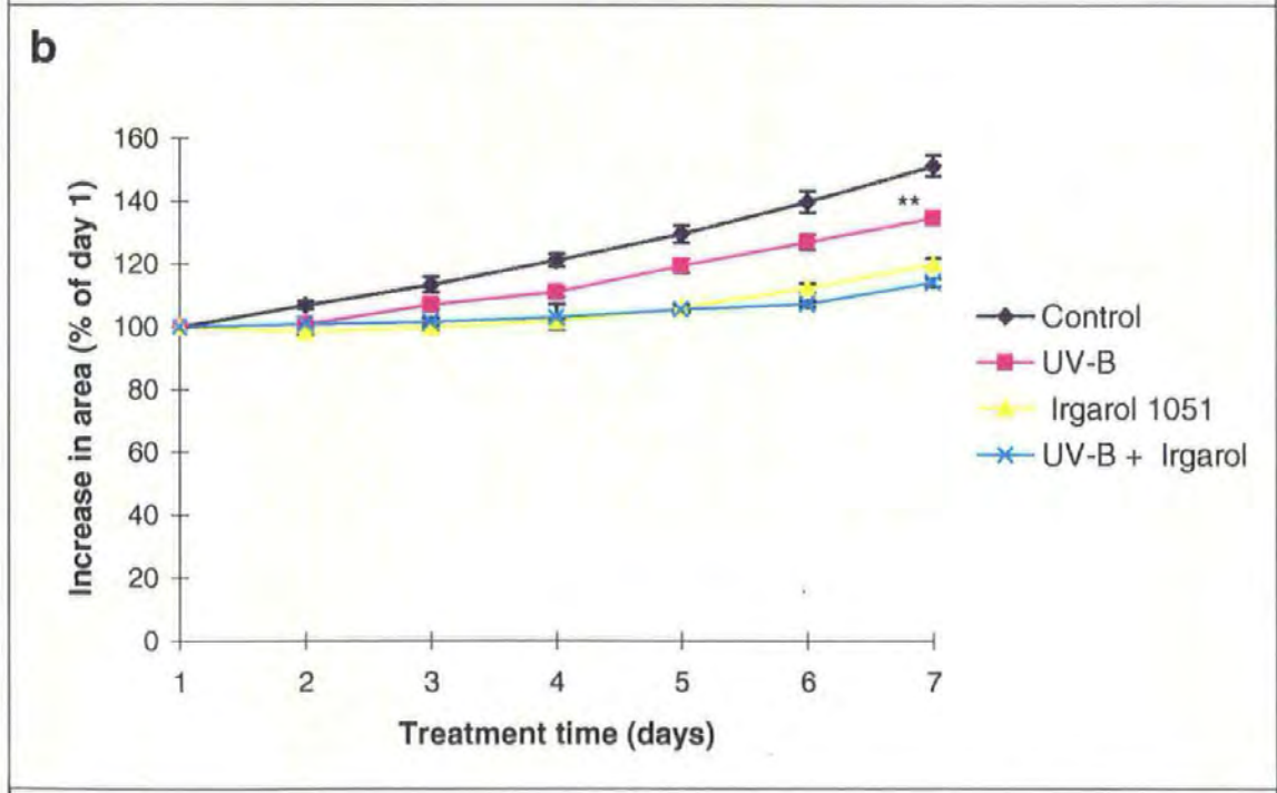
Figure 8.5. Increase in thallus area in a) Palmaria palmata and b) Porphyra umbilicalis as a function of treatment time to UV-B and/or Irgarol 1051 exposure. For both species a UV-B irradiance of 2.1 \text{ W m}^{-2} was applied on day 0 in these treatment groups (50 min exposure for P. palmata and a 6 hour exposure for P. umbilicalis respectively). Irgarol 1051 ( 5 \mu\text{g l}^{-1} ) was applied throughout the treatment period. Means \pm SE, n = 9. *, ** indicate significant different slopes in all treatment groups compared to non-treated controls. Data was calculated as % increase in area and differences in slopes and intercepts were tested in multiple regression analysis, p < 0.05 , p < 0.01 .
