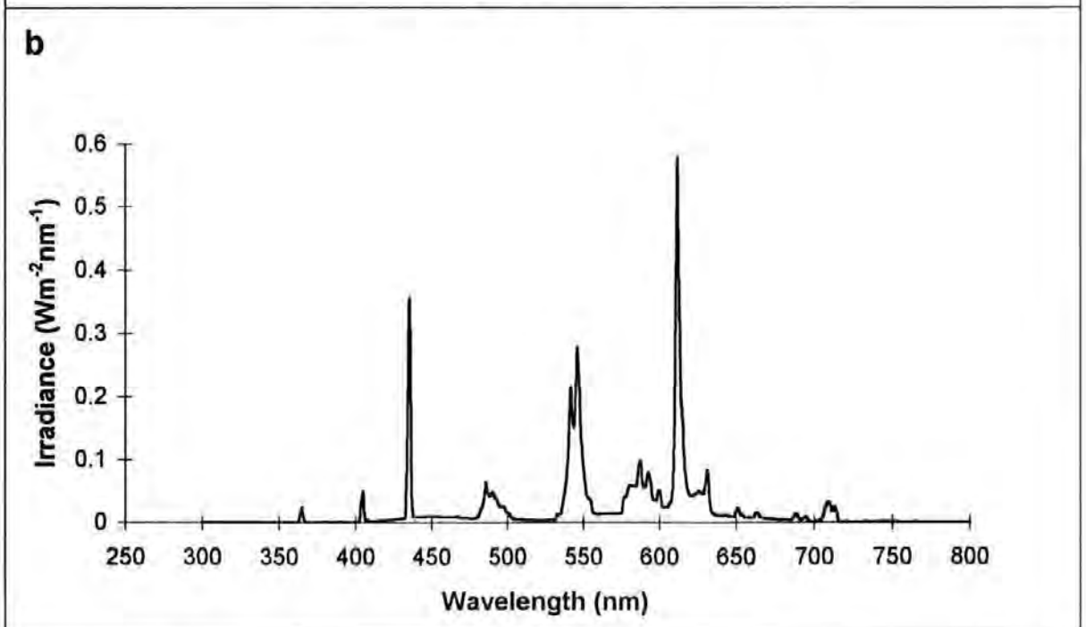
Figure 2.1 a) Emission spectra of UV-B and UV-A tubes used in the different experiments throughout this thesis. UV-B tubes (Philips TL' 20W/12 RS) and UV-A tubes (Philips 1609 15 W) were covered with 35 \mu\text{m} cellulose diacetate foil to filter out UV-C, or UV-B tubes were fitted with Mylar 125 D. b) Emission of fluorescence tubes, Phillips TLD 32W/83 HF, used as background Photosynthetically Active Radiation. Since varying UV and PAR irradiances were used throughout this work, the total irradiance shown on the figure should be regarded as an example.
