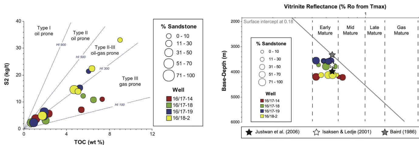
Figure 14. Thermal maturity depth plot showing early-mid mature oil generation window based on vitrinite reflectance values converted from Rock-Eval T_{\max} compared with similar maturity/depth values recorded by Baird (1986), Justwan et al. (2006) and Isaksen and Ledje (2001).
