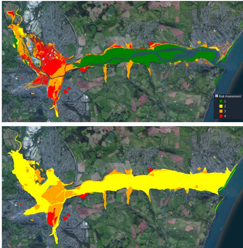
Figure 8. Risk Assessment: No mitigation options (up) vs All mitigations (down). Mid-term conditions: 2050 yr, Tr 50 yrs. Scale: Low (green), Moderate (yellow), Medium (orange) and High (red) risk.
