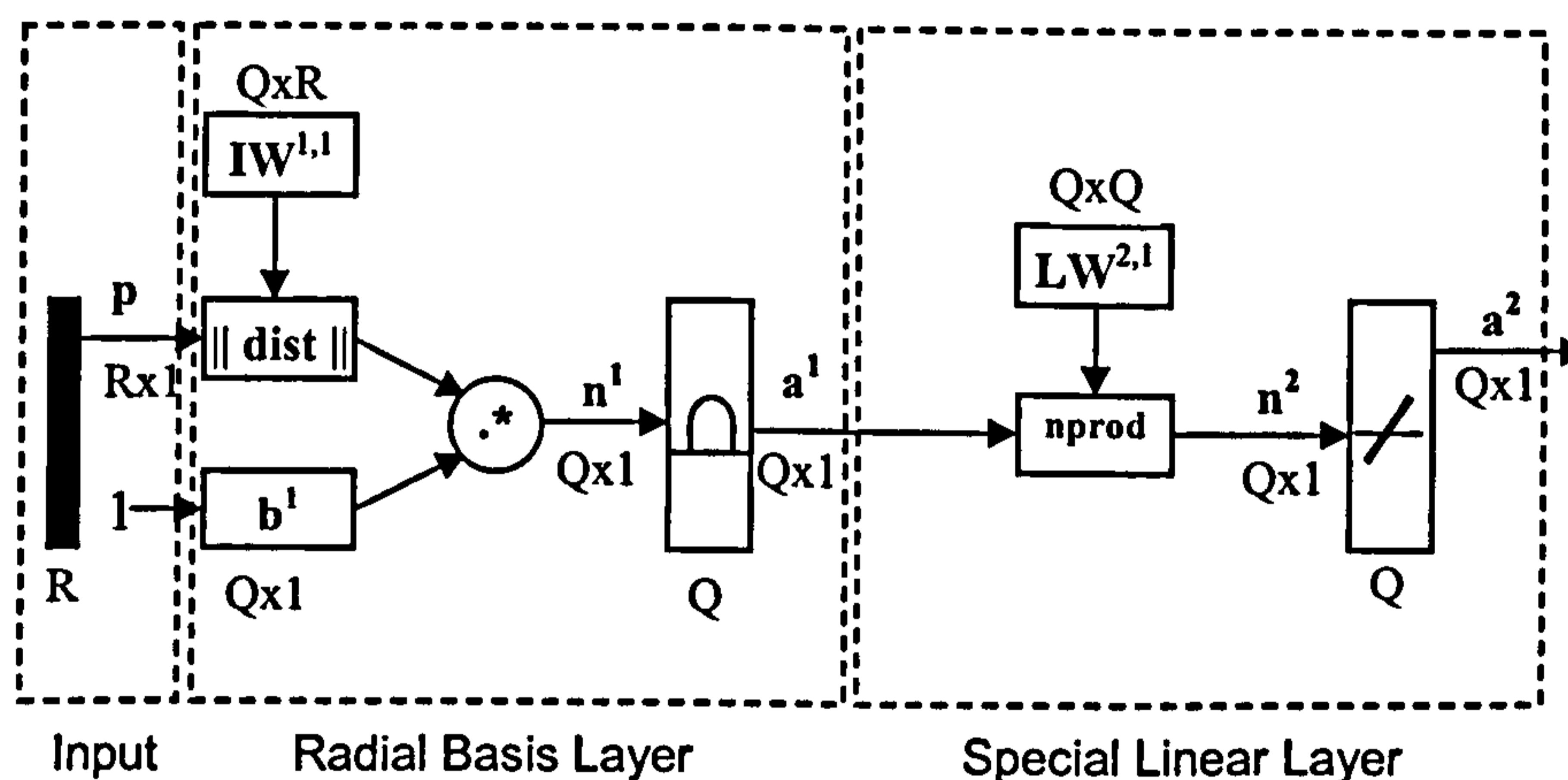
Figure 9 Generalised Regression Network
