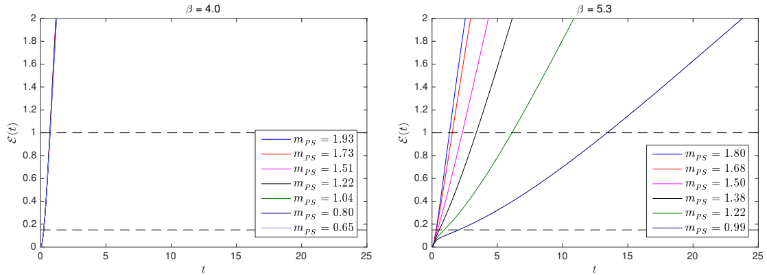
Figure 8. Determination of the t_0 observable for two different bare couplings. The left panel at \beta = 4.0 is in the strong coupling region (Region I), while the right panel at \beta = 5.3 is in the weak coupling region (Region II). The observable has a negligible quark-mass dependence in Region I, but a very strong quark-mass dependence in Region II. The dashed horizontal lines are the reference values \mathcal{E}_{\text{ref}} = 1 and \mathcal{E}_{\text{ref}} = 0.15 . The quark mass dependence in the two regions is not influenced by the choice of the reference value.
