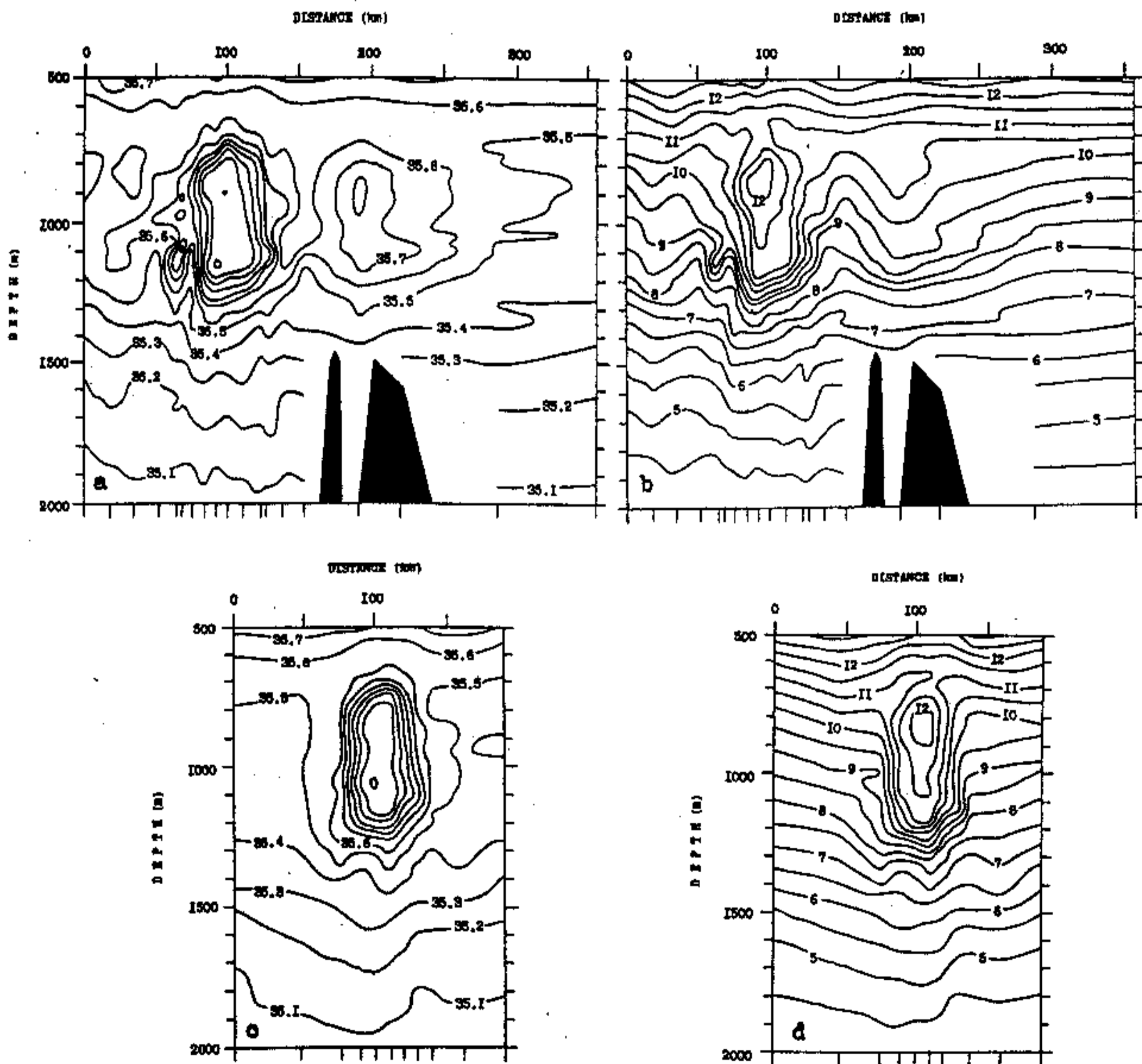
Figure 5 Salinity and temperature cross sections for the major (a,b) and minor (c,d) axes of Meddy "Irving". Location of CTD stations is shown by ticks at the bottom.
