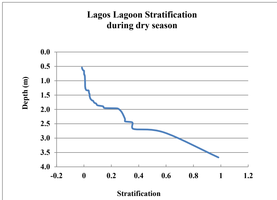
Figure 6.21: Stratification of the lagoon during the dry season exhibiting stratified mixing
