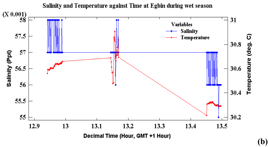
Figure 6.13: Salinity and Temperature variations against Time of observation at Egbin. (a) Salinity and temperature behaviour during the dry season, (b) Reaction of salinity and temperature during the wet season
