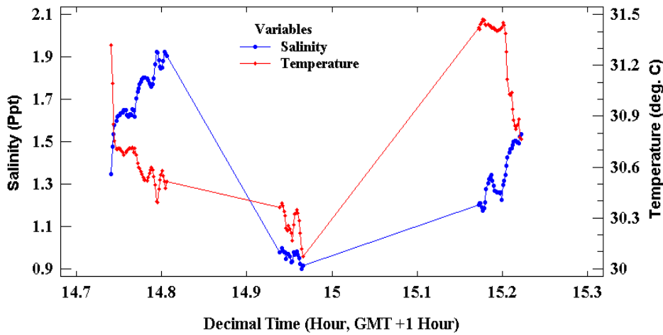
Figure 6.12: Salinity and Temperature variations against Time of observation at Five Cowries. The Lagoon has equal water mass was found to be the same at about 9:06am and 9:30am; 2:45pm and 3:12pm during the dry and wet season respectively (a) Salinity and temperature behaviour during the dry season, (b) Reaction of salinity and temperature during the wet season
