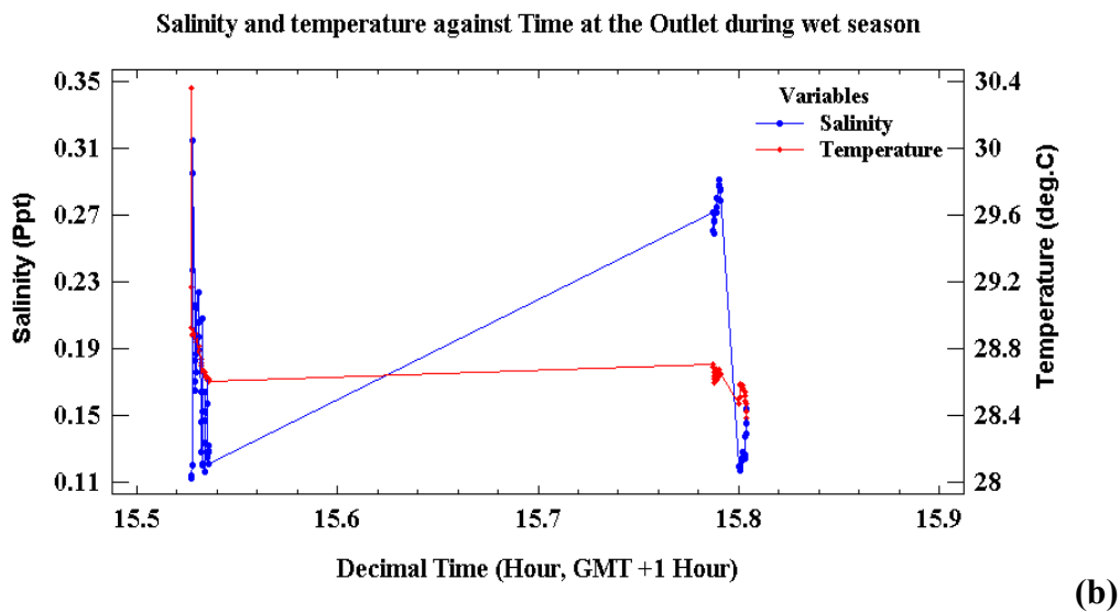
Figure 6.11: Salinity and Temperature variations against Time of observation at the outlet. (a) Salinity and temperature behaviour during the dry season, (b) Reaction of salinity and temperature during the wet season
