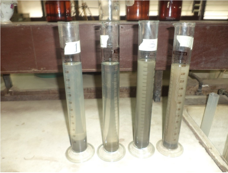
Figure showing the Hindered experiment, the tube contain sediment suspension that settles at different rate depending on the size of the particle. The experiment was carried out at the laboratory of the Department of Civil & Environmental Engineering, Faculty of Engineering, University of Lagos
