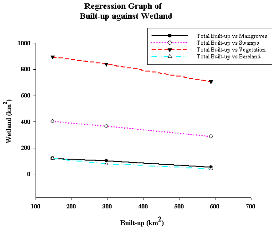
Figure 4.20: Regression graph showing correlation relationship of built-up area against mangroves, swamps, vegetation and bare-land
