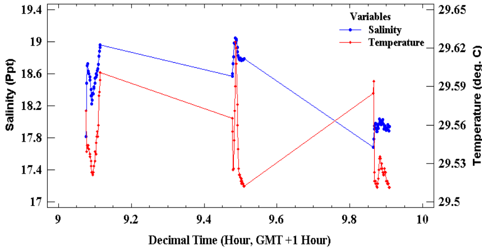
Salinity and temperature against Time at Five-Cowries during wet season
