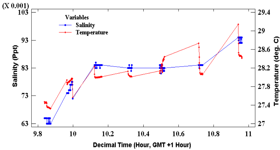
Figure 6.14: Salinity and Temperature variations against Time of observation at the inlet. (a) Salinity and temperature behaviour during the dry season, (b) Reaction of salinity and temperature during the wet season
