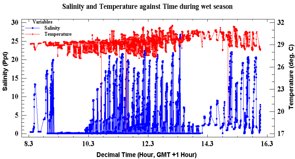
Figure 6.16: Salinity and Temperature variations against Time of observation on the entire case study area on the Lagoon during dry and wet season. (a) The general behaviour of salinity and temperature during dry season, (b) the reaction of salinity and temperature during wet season
