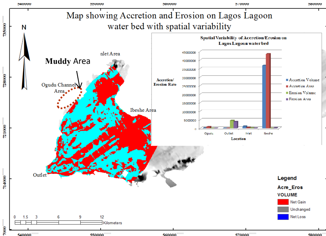
Figure 5.18: Spatial variability of sediment Accretion and Erosion on Lagos Lagoon water based on 2008 and 2014 repeated bathymetric data
