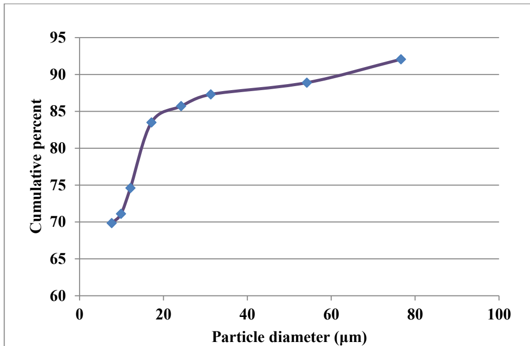
Figure 6-A5: Andreasen empirical test on the sample data at Ijede (554950mE, 722533mN)
