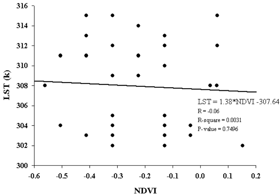
Figure 4.34: LST – NDVI correlation along south - north transect at the western region of the Lagoon ecosystem in 2002. Note the gradual change of the slope from negative to positive proceeding from the south
