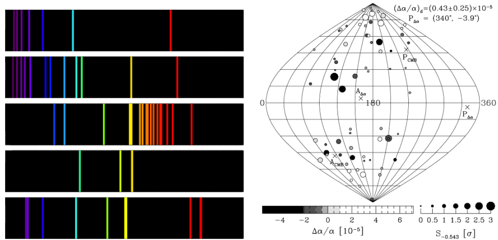
(a) Sample absorption spectra of elements H, He, Ne, Na, and Hg (from top) (b) Galactic distribution of \Delta\alpha/\alpha as shown in (Murphy et al. 2003)
