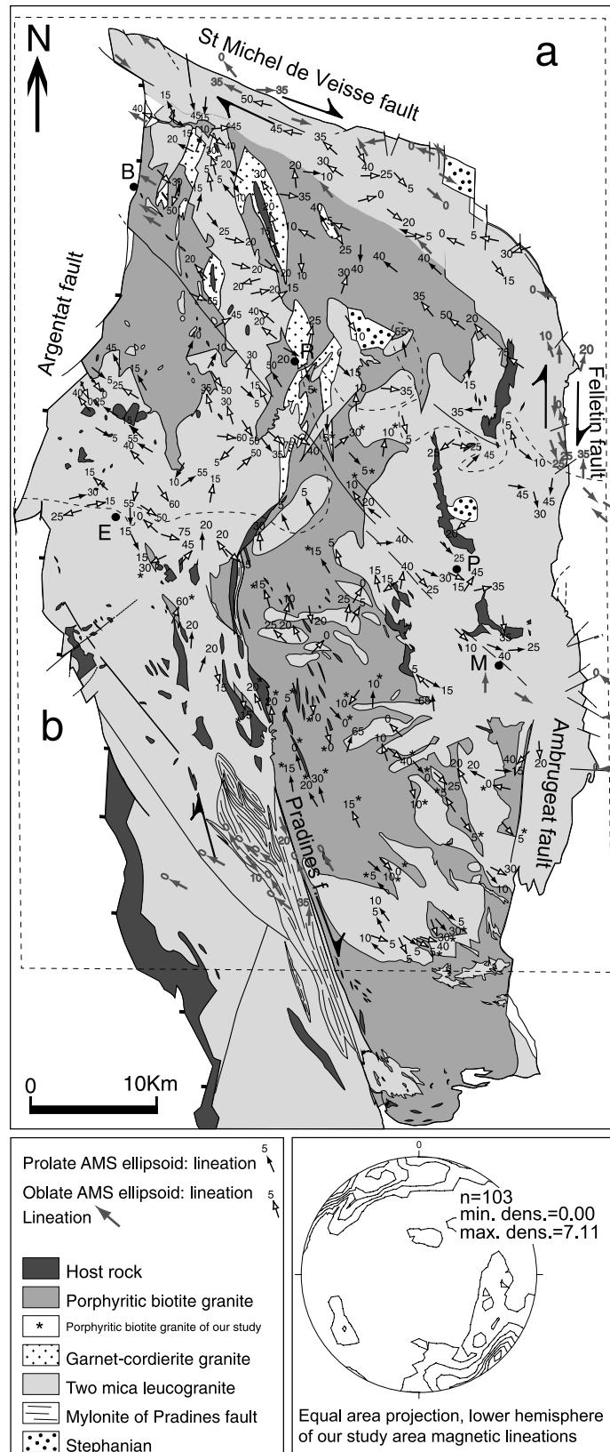
Fig. 8. Magnetic lineations of the Milllevaches massif: (a) AMS data from Jover (1986), (b) AMS data from our study area. M: Milllevaches; P: Peyrelevalde; E: Eymoutiers; R: Roy ere-de-Vassivi eres; B: Bourganeuf.
