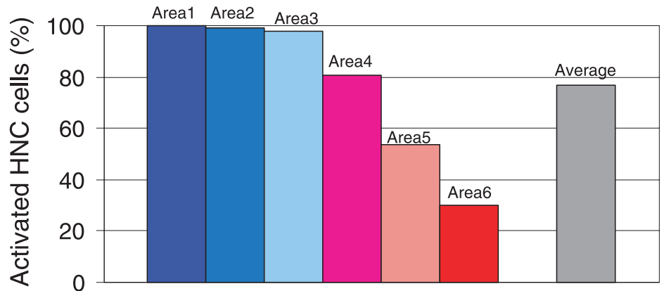
FIG. 10. Pattern-completion abilities of a Hebbian neuronal circuit (HNC). The bars show the cumulative portion of an HNC (% of HNC cells per area) that a learnt stimulus presented to Area 1 successfully reactivates over the 50 steps following stimulation, averaged across 32 different 'auditory' patterns. These data are calculated by integrating (in time) the curves shown in Fig. 9. The rightmost column is the average of the six area-specific values.
