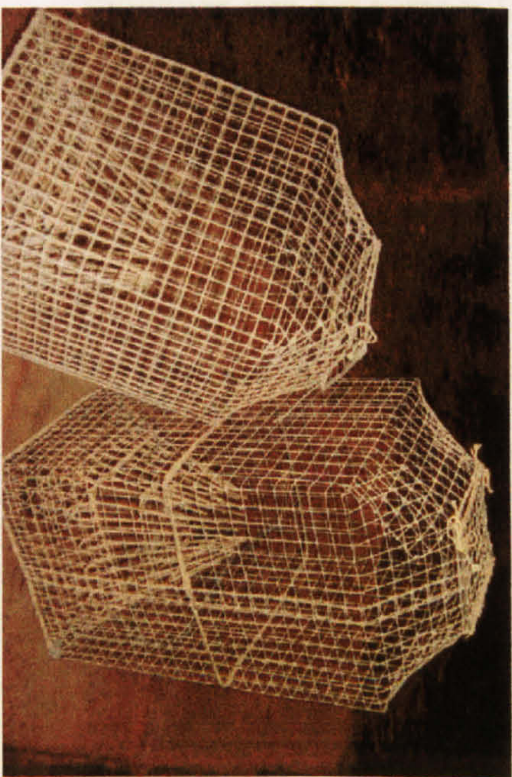
Plate 3.8 Octopus traps
