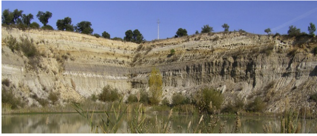
Fig. 8 The V.Atela-E outcrop, with the base at the transition of the LG unit to the US unit. Almost all of the local thickness of the US unit is exposed here (ca. 18 m). The Atela 2 sample was collected at ~2.5 m below the cliff top.
