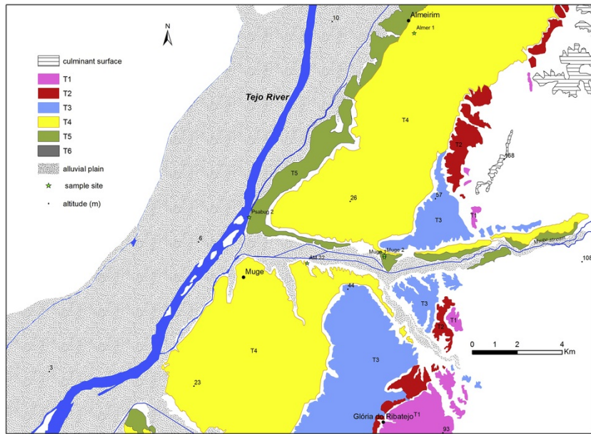
Fig. 16 Map of the Tejo terrace staircase in the Muge area, downstream of Alpiarça. Stratigraphic location of the samples collected for luminescence dating: AM-22 (T4, base of the US unit); PSabug-2 (T5 top); Muge-1 and Muge-2 (T5 top); Almer-1 (Carregueira Formation; aeolian cover sands, not mapped in this figure).
