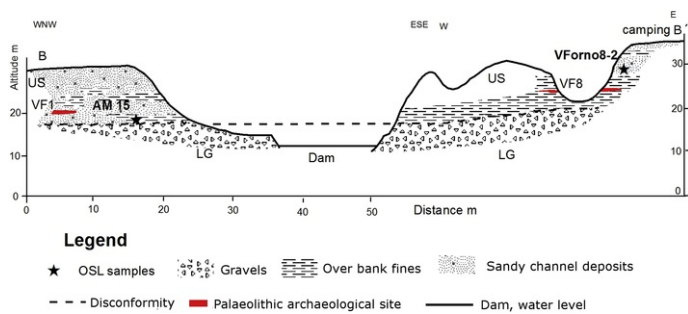
Fig. 6 Stratigraphic cross section B - B'. This section shows that the US unit is dominated by sand channel facies in the west and rich in flood-plain clayish silts in the east. The topographic position of sample AM 15 is at near distance from the cross section (see Fig. 4), in the west side of the Vale do Forno streamlet.
