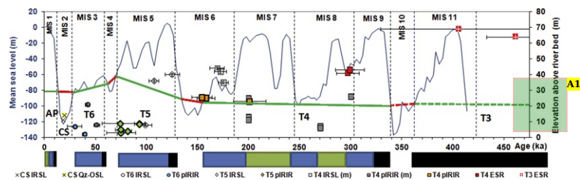
Fig. 17 Burial ages of samples collected from Middle to Late Pleistocene sedimentary units of the Tejo reach IV, plotted according to the respective elevation a.r.b. (right axis). Horizontal bars indicate the dominant lithologies for the fluvial deposits (black - gravels; blue - sands; green - silty clays) and the probable age range of each sedimentary unit. For this reach, the periods of aggradation are represented by green line segments and the periods of river downcutting are represented by red line segments that cross the sea-level curve (scaled benthic isotopes from V19-30, after Cutler et al., 2003), testifying a dominant sedimentary control by glacio-eustasy. T3, T4, T5 and T6 - terraces; CS - Carregueira Formation (aeolian sands); AP - Alluvial plain deposits. MIS
