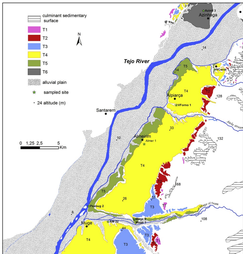
Fig. 3 Terrace staircase of the River Tejo reach IV. The T6 terrace is only visible near Azinhaga village, whilst T5 is buried by modern alluvium downstream of Muge. Note the asymmetric development of the terraces between the two sides of Tejo valley downstream of Chamusca. Terraces are very scarce on the west side of the river valley.
