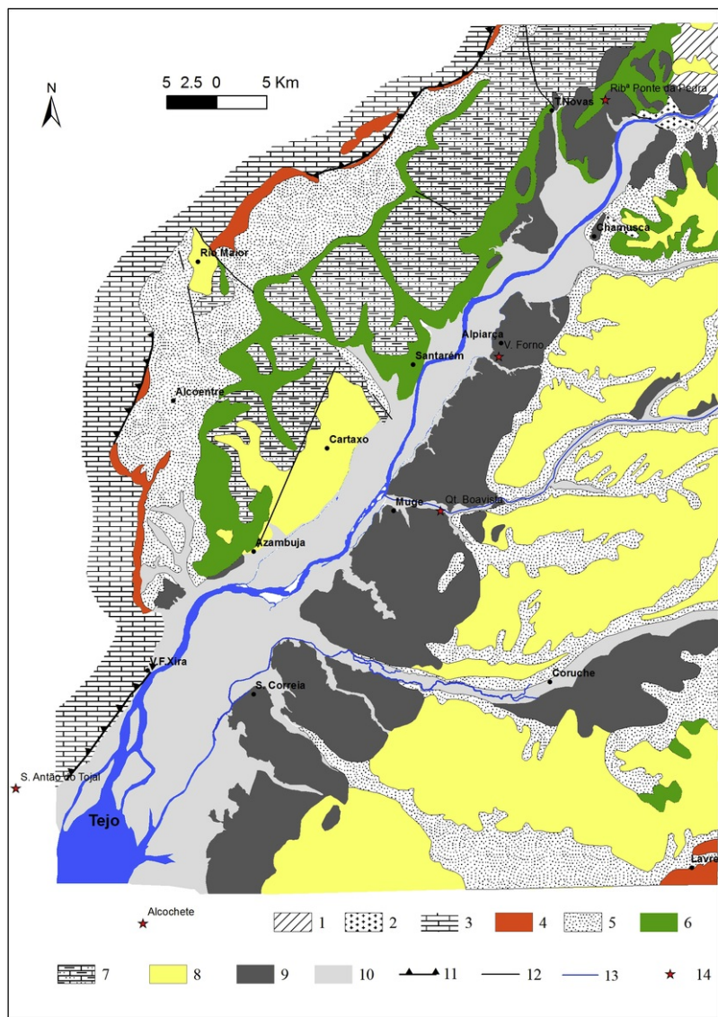
Fig. 2 Simplified geological map of the region (adapted from the Carta Geológica de Portugal, 1/500,000, Oliveira et al., 1992 and Barbosa, 1995). 1 - metasediments of the Hesperian Massif; 2 - granites of the Hesperian Massif; 3 - limestones and sandstones (Mesozoic); 4 - sandstones and conglomerates (Paleogene); 5 - sands (Lower Miocene); 6 - silts and clays (Miocene); 7 - limestones, silts and clays (Miocene); 8 - gravels and sands (Pliocene); 9 - gravels of fluvial terraces (Pleistocene); 10 - modern alluvium: mud, silt and sand (Holocene); 11 - thrust fault; 12 - fault; 13 - stream; 14 - archaeological site.
