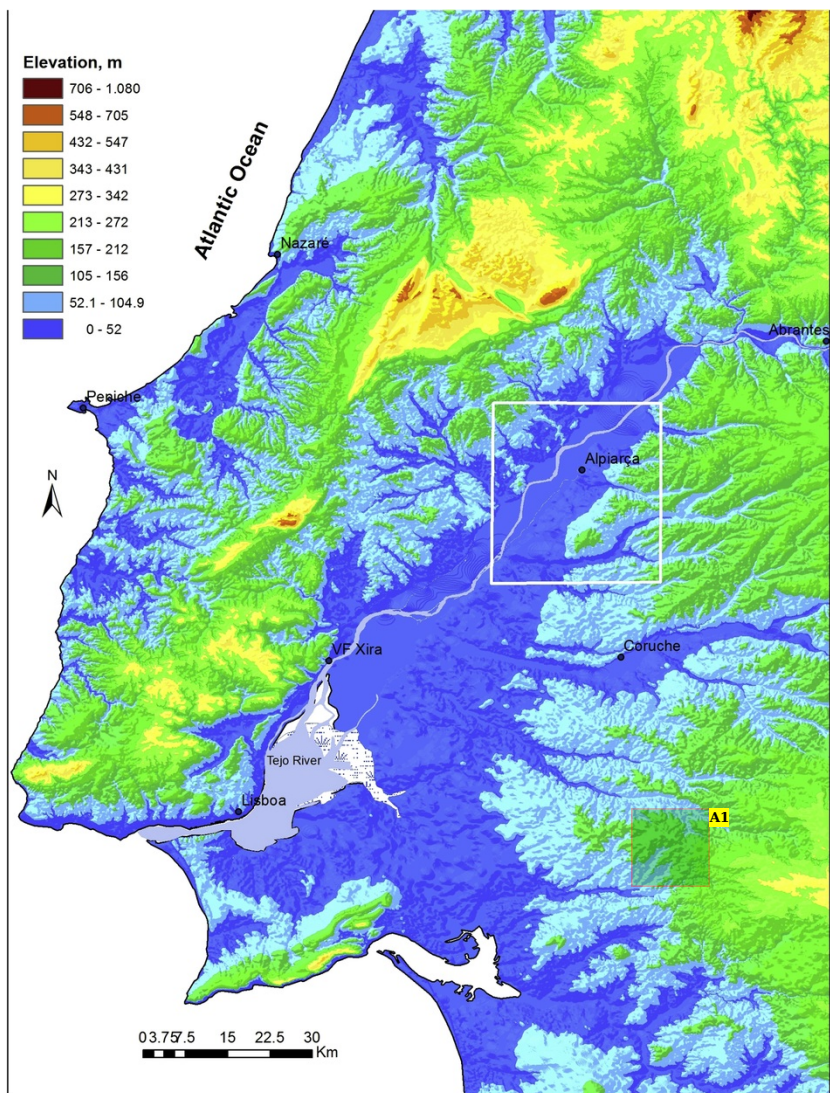
Fig. 1 Location of the study area in the Lower Tejo (central Portugal). Hypsometry and digital elevation model obtained from SRTM data.
