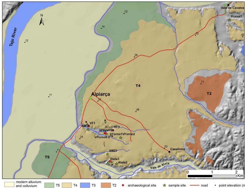
Fig. 4 Map of the Alpiarça area, comprising the River Tejo tributary valleys of Vale do Forno and Vale de Atela. Location of the sites and cross sections (A - A' and B - B'). It is deduced from the contour lines that the interfluvies between the Vale do Forno and Vale de Atela is developed in eroded (dissected) uppermost T4 deposits.
