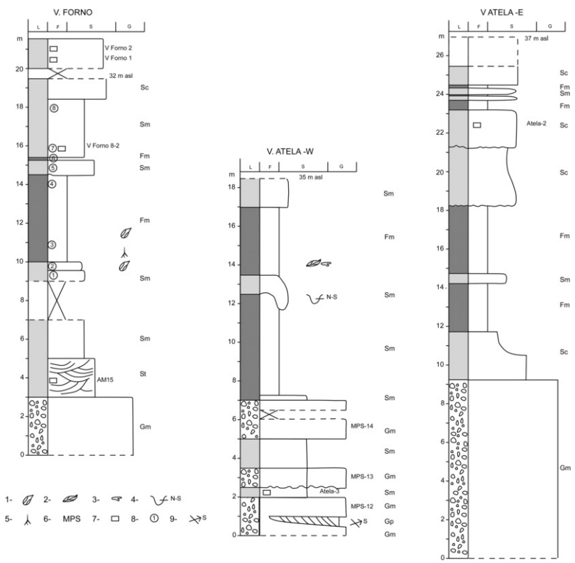
Fig. 7 Stratigraphic logs of the sections at V. Furno (the VF8 site), V. Atela-W and V. Atela-E (see Fig. 4 for location). Most of the samples for luminescence dating are from here (AM 15, VForno 8-2, VForno 8-7, VForno 1, VForno 2, Atela 2, Atela 3 and Atela 4). 1 - archaeological level; 2 - vegetal macro remains; 3 - coal fragment; 4 - channel geometry; 5 - fossil roots; 6 - Maximum pebble size (mean diameter of the larger 10 clasts per level); 7 - sample for luminescence dating; 8 - sample for sedimentology; 9 - paleocurrent derived from planar cross-bedding.
