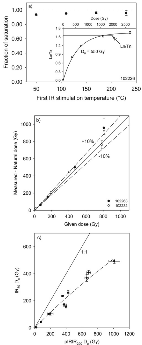
Fig. 15 a) First IR stimulation plateau for sample 102226. The natural signals are expressed as a fraction of the saturation level of the dose response curve. Three aliquots were measured per temperature and error bars represent one standard error. The inset shows the sensitivity corrected natural pIRIR290 signal (horizontal solid line) interpolated on the dose response curve for one aliquot measured using a first IR stimulation temperature of 50 °C. b) Results of the dose recovery measurements. At least three aliquots were measured per data point and error bars represent one standard error. c) IR 50 De values plotted as a function of the pIRIR290 De values for samples for which the pIRIR290 De is \leq 2 \times D_0 (see Table 4); error bars represent one standard error. The dashed line is the best fit through the data points.
