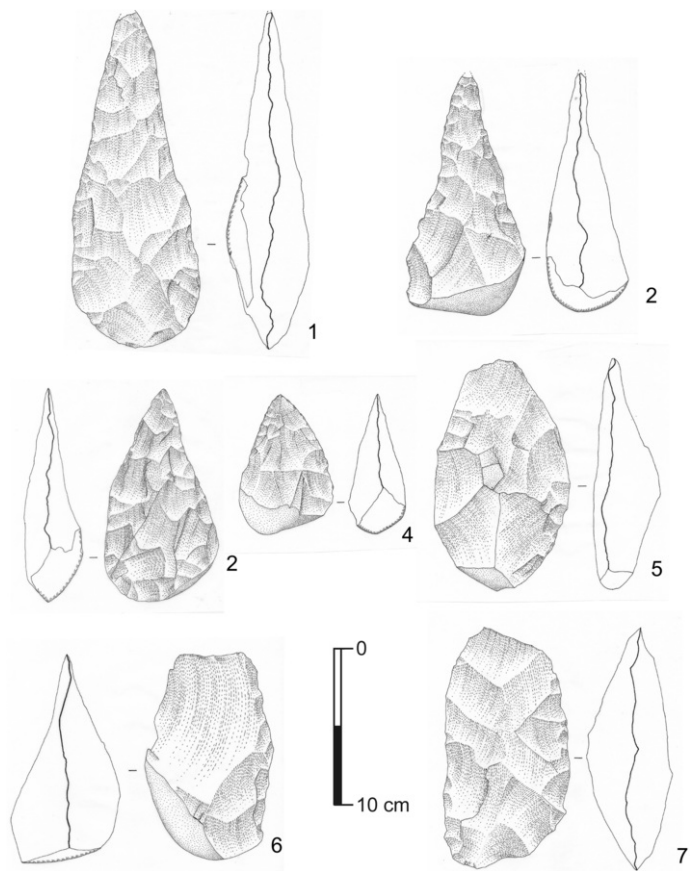
Fig. 13 The final Achdeulian industry of VF3 site (Milharós site). Bifacial tools. 1 to 5 - Bifaces (Micoquian, lanceolate, ovalar); 6 and 7 - Bifaces with distal cutting edge.
