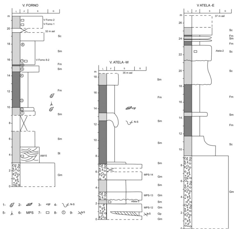
Fig. 7 Stratigraphic logs of the sections at V. Forno (the VF8 site), V. Atela-W and V. Atela-E (see Fig. 4 for location). Most of the samples for luminescence dating are from here (AM 15, VForno 8-2, VForno 8-7, VForno 1, VForno 2, Atela 2, Atela 3 and Atela 4). 1 - archaeological level; 2 - vegetal macro remains; 3 - coal fragment; 4 - channel geometry; 5 - fossil roots; 6 - Maximum pebble size (mean diameter of the larger 10 clasts per level); 7 - sample for luminescence dating; 8 - sample for sedimentology; 9 - paleocurrent derived from planar cross-bedding.
