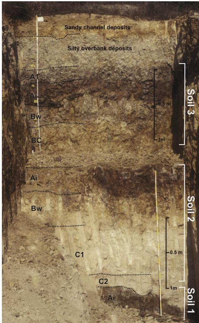
Fig. 9 Paleosols developed in the overbank deposits of the T4 terrace US unit, at the AL1 site (... at the AL1 site (see Fig. 4 for location)).
