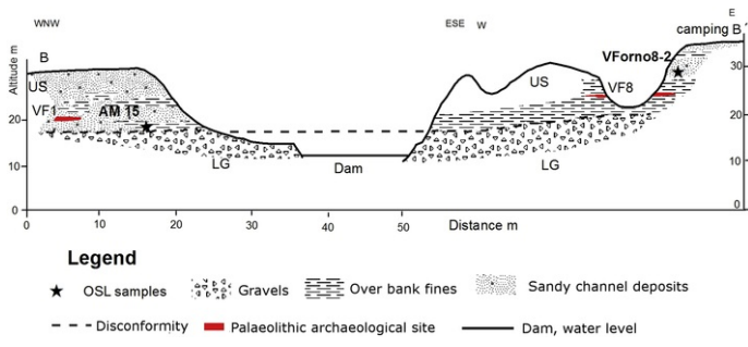
Fig. 6 Stratigraphic cross section B - B'. This section shows that the US unit is dominated by sand channel facies in the west and rich in flood-plain clayish silts in the east. The topographic position of sample AM 15 is at near distance from the cross section (see Fig. 4), in the west side of the Vale do Furno streamlet.
