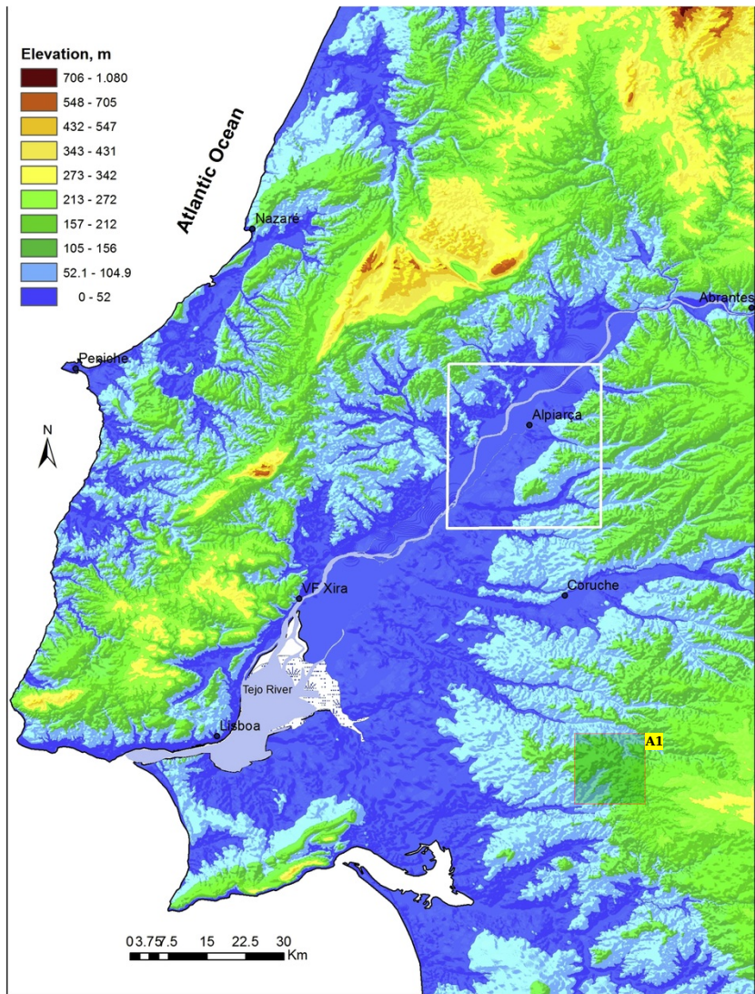
Fig. 1 Location of the study area in the Lower Tejo (central Portugal). Hypsometry and digital elevation model obtained from SRTM data.
