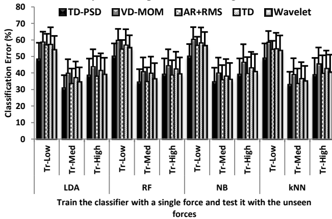
Fig. 6 Classification errors of nine amputees when training the classifier with one force and performing the testing with unseen force levels ( Experimental Scheme 2 ). Standard deviation is shown with error bars. Tr denotes training with a specific force.
