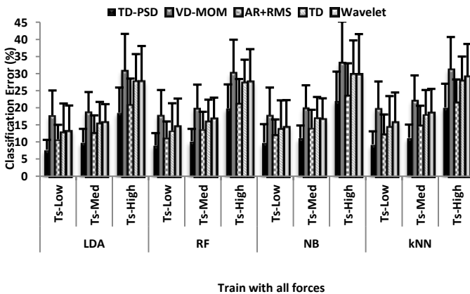
Fig. 7 Classification errors for nine amputees when training with all force levels and testing the classifier with each level of the three forces ( Experimental Scheme-3 ). Standard deviation is shown with error bars. Ts denotes testing with a specific force.
