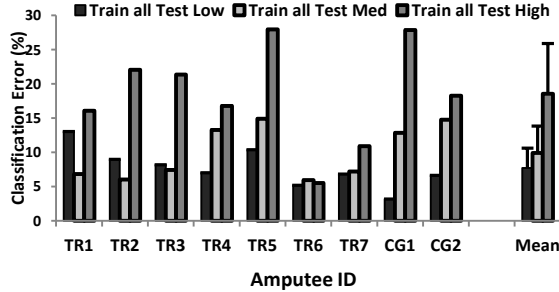
Fig. 8 The results the experimental Scheme3 for nine amputees when training with all forces with TD-PSD and LDA classifier for nine amputees. The mean of all amputees is shown and error bars represent standard deviation.
