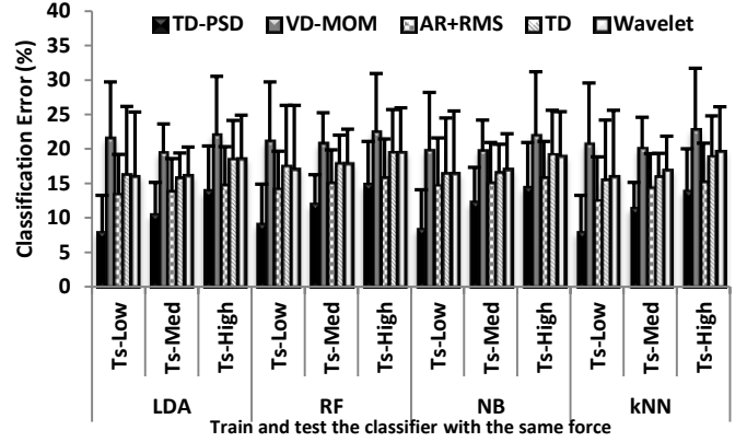
Fig. 5 Average classification errors for nine amputees when training and testing the classifiers with the same force level ( Experimental Scheme 1 ) with five feature sets and four classifiers (LDA, RF, NB and kNN). Standard deviations are shown with error bars. T_s denotes testing with a specific force.
