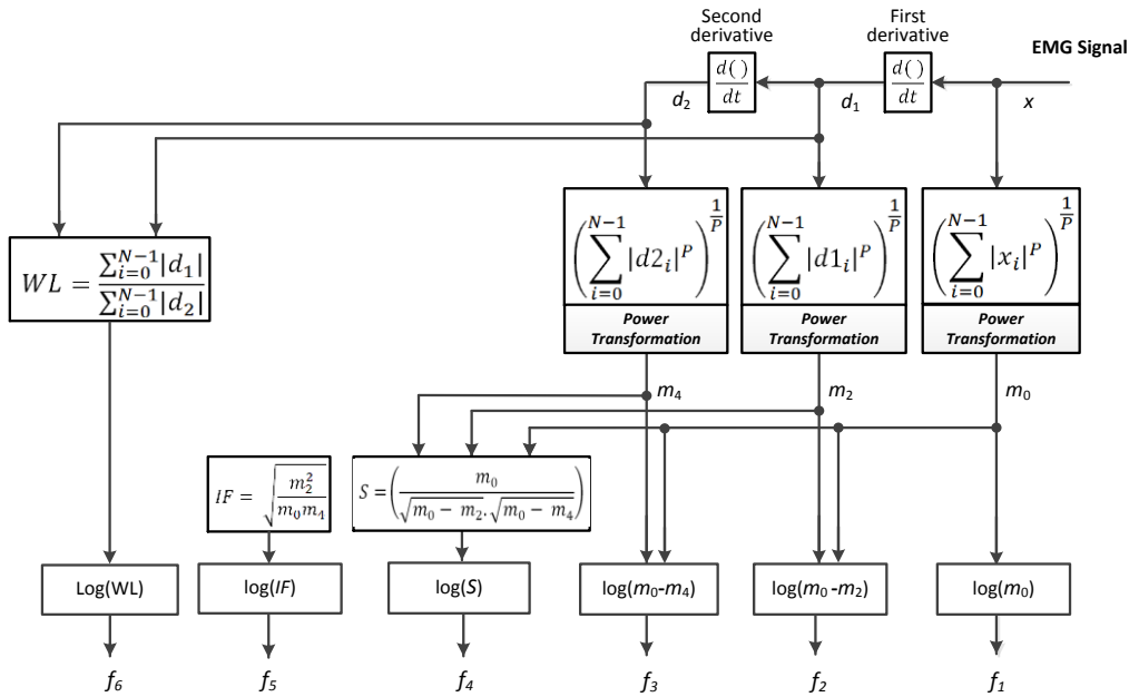
Fig. 1. Block diagram of the proposed feature extraction process.
