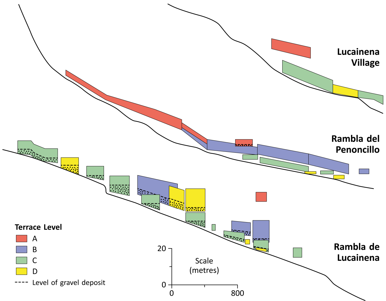
Fig. 10. Long-profiles for the terrace sequences in the Lucainena headwater tributaries and the Rambla de Lucainena (Box 3, Fig. 6). Terrace A >300-400 ka; Terrace B > 200 ka; Terrace C >78 ka; Terrace D 32.5±3.4 ka to 10ka; from Whitfield and Harvey (2012).
