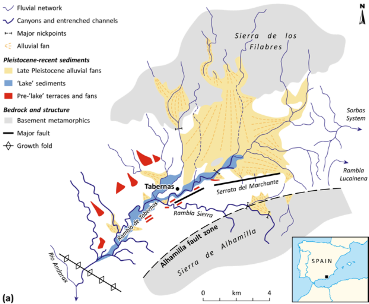
Fig. 7. Alluvial fan and related geomorphology from the Tabernas Basin (Box 1, Fig. 6). (a) plan view showing coupled west of basin and buffered east of basin. (b) relationship between buffering alluvial fans and incised terrace sequence from the west of the basin. Modified from Harvey et al., 2014. L1-L4 refer to the levels of Geach et al., (2015).
