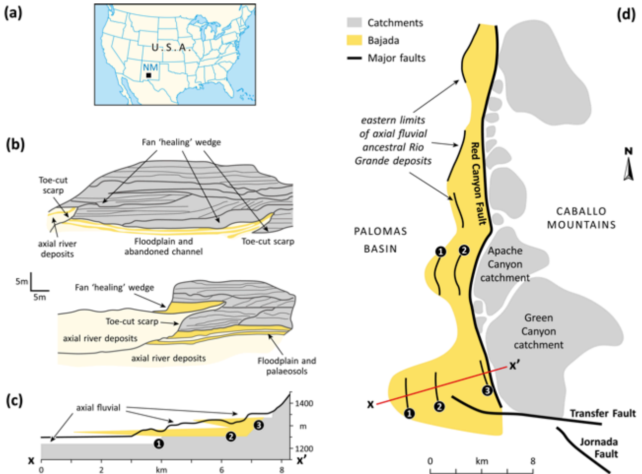
Fig. 5. Examples of the impact of lateral toe-cutting on Quaternary alluvial fan and fluvial archive stratigraphy in New Mexico. Diagrams modified from Leeder and Mack (2001). (a) General location (b) Stratigraphy through the fluvial archives based on field observations from the Palomas Basin. Note presence of toe-cut scarps and prograding alluvial fan 'healing wedge' stratigraphy. (c) distribution of intercalated river and alluvial fan deposits along the Palomas Basin in section and in planform (d). Note location of section X to X' along a transfer fault – see discussion as to significance of this.
