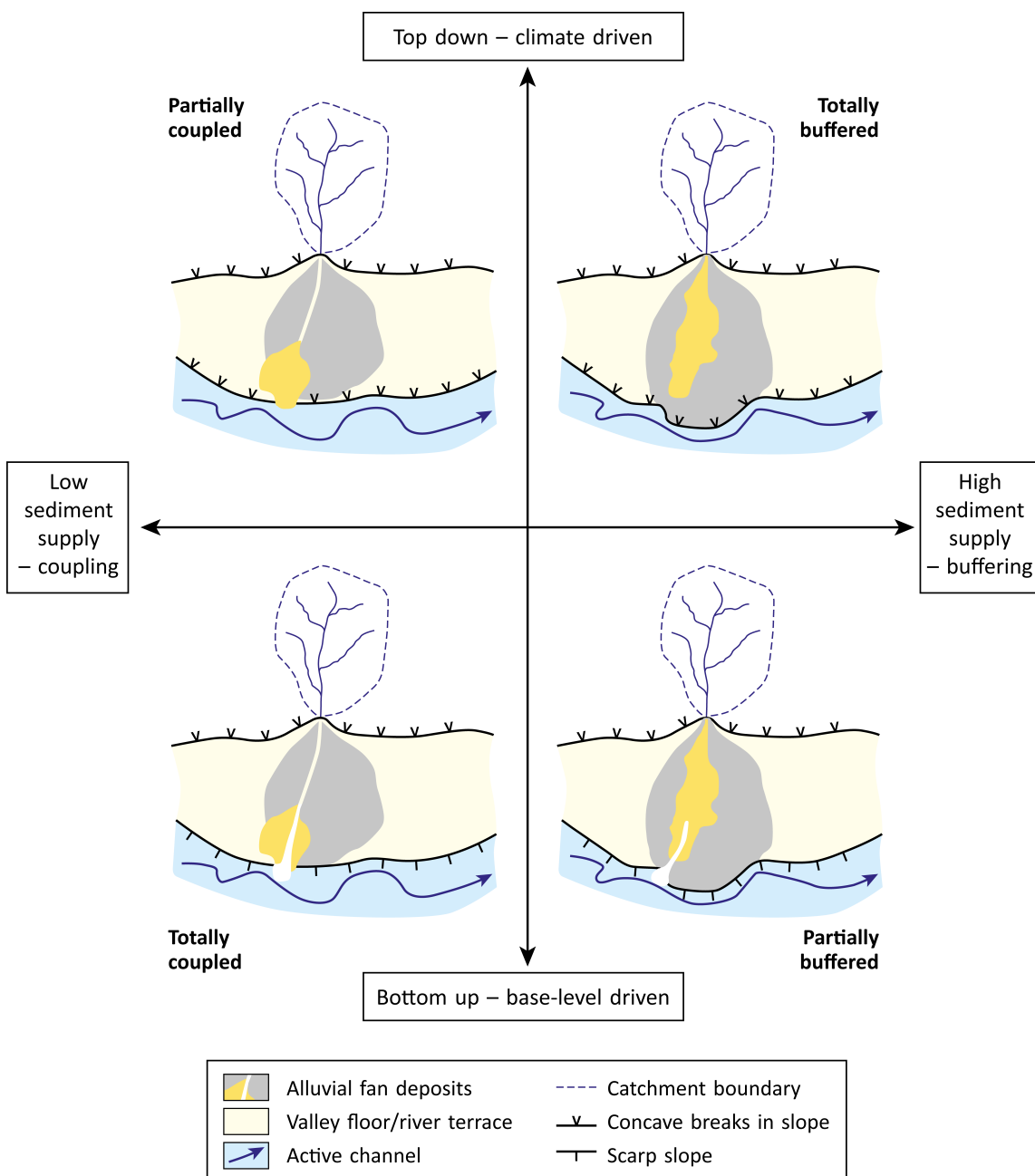
Fig.3. A conceptual model, taken from a summary of the published literature and new data used within this article, to describe behaviour of a simple alluvial fan in a tributary setting adjacent to a main river under different spatial controls (top down versus bottom up) and varying sediment supplies to the alluvial fan. The axes of the model demonstrate the key drivers which may act as top down controls on sediment and water discharge to the alluvial fan (most commonly climate driven) and bottom up base-level lowering (main river behaviour) which most commonly would be main river incision, although foreshortening of alluvial fans through main river lateral toe-cutting can have similar effects. The horizontal axis represents the direction of change in sediment supply to the alluvial fan in the form of increasing sediment supply, which ultimately can lead to the alluvial fan displacing and buffering the river from slope processes or facilitating incision in cases of sediment supply reduction. Generally within this kind of setting enhanced coupling is encouraged by main river incision (or lateral toe cutting) and also by reduction in sediment supply that promotes trenching on the alluvial fan. In the case of toe cutting the connection is most likely to be made on the upstream side of the main river flow direction.
