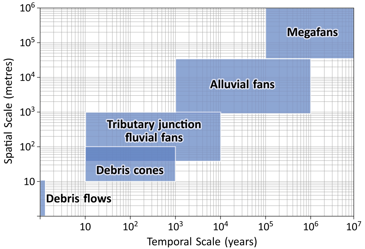
Fig. 1 The spatial and temporal scales typical of typical slope processes and landforms that commonly interact with river terrace records.
