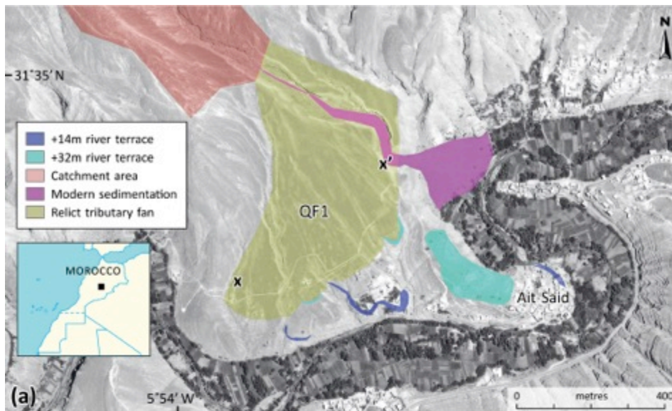
Fig. 13. (a) Location of the Ait Said tributary alluvial fan (QF1) in the River Dades Catchment. (a) relationship of alluvial fan and river terrace deposits. Darker area of image is the Holocene flood plain of the River Dades. Images courtesy of Google Earth Professional 2016. (b) field image of the tributary alluvial fan and terraces. Note steepness of alluvial fan surface ( 6^\circ ) compared to modern river. X – X' indicates position of cross-section, blue arrows indicate line of trench through alluvial fan. (c) cross-profile through the alluvial fan showing insipient incision and alluvial fan head trench (RHS) and (d) modern alluvial fan trench profile and relict alluvial fan surface (QF1) taken up the mid-fan line. Field survey undertaken using a Trupulse™ 360° laser range finder.
