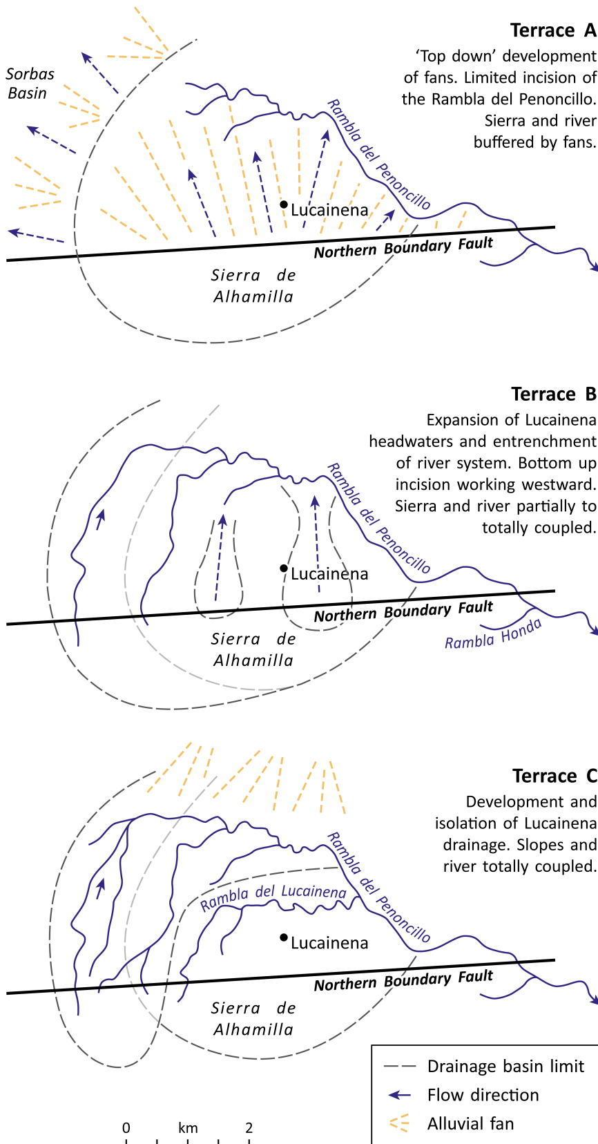
Fig. 12. River capture acting as a bottom up coupling mechanism for the alluvial fan and river system in the headwaters of the Rambla Lucainena and Rambla del Penoncillo (Box 3, Fig. 6), and demonstrating the time transgressive nature in the landscape from east to west.
