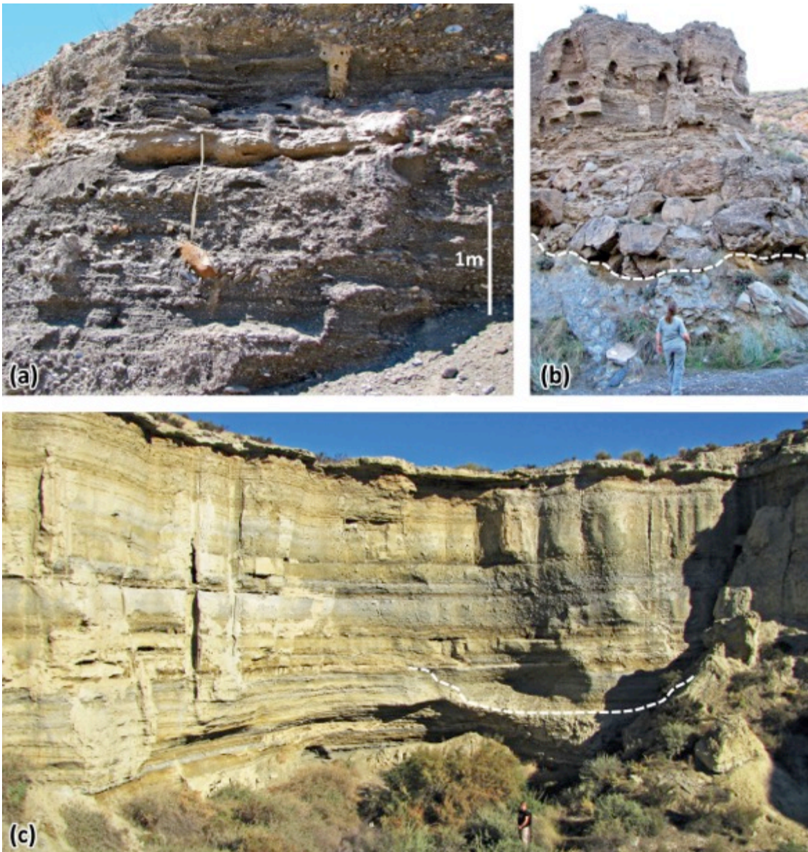
Fig. 8. Field images from Tabernas. (a) Level 2 alluvial fan deposits displaying evidence of tractional flow and sheetform geometries suggesting unconfined flows (section oblique to flow which is to the left). (b) Level 3 coarse terrace deposits from Rambla Sierra (Fig. 7a) lying unconformably on Neogene basin deposits within the Rambla Sierra (southwest portion of the Tabernas Basin) which at this time is buffered by an alluvial fan at its mouth from the more central basin locations. Dashed line indicates base of terrace. (c) palustrine – lacustrine sediments of Level 3 in the basin centre. Note the lack of fine sediments. Dashed line picks out erosive channel within the Level 3 sediments. The coarsest material observed in the section is medium to coarse sand. Note person in foreground for scale.
