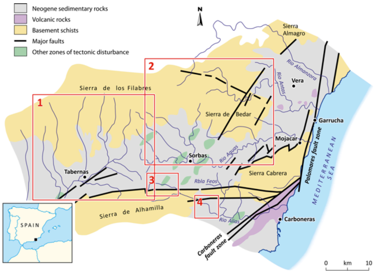
Fig. 6. Location map for SE Spain case studies. Figs. 7 and 8 (Box 1); Fig. 9 (Box 2); Figs 10 and 12 (Box 3) and Fig. 11 (Box 4). Inset image courtesy of Google Earth Professional 2016.
