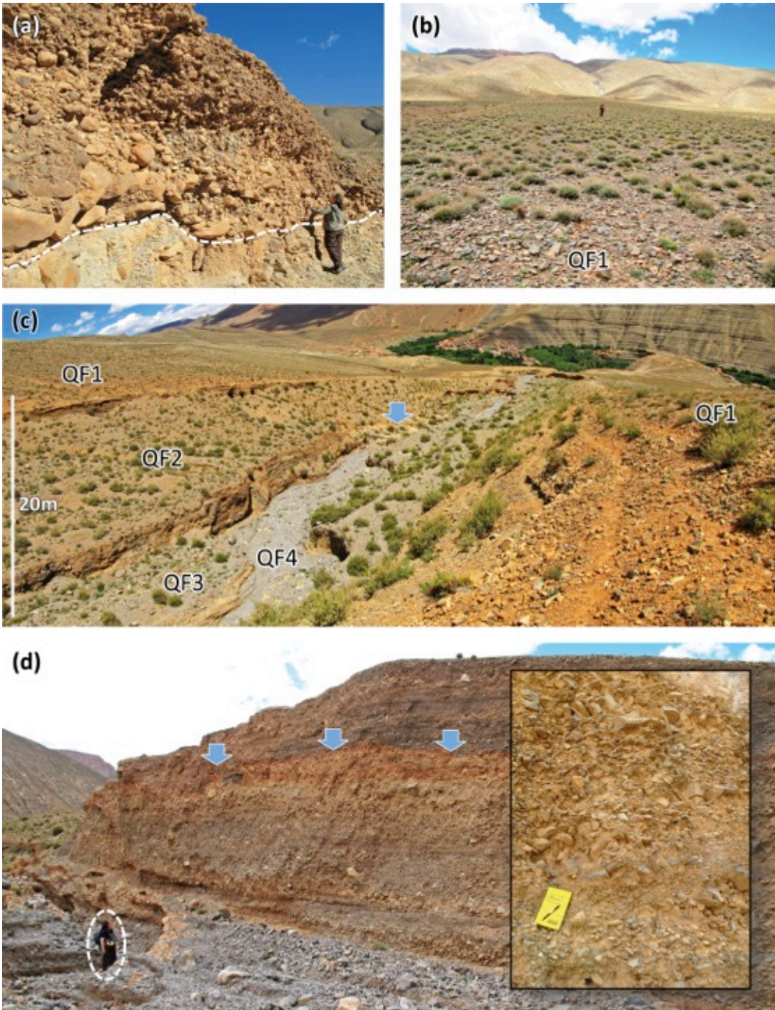
Fig. 14. Field images from the Dades study area of the Quaternary landform and associated sediments. (a) river terrace level at Ait Said (base 32m above modern river level). Note well rounded cobbles and clast supported nature of the deposits. Provenance is the same as the tributary junction alluvial fan (predominantly limestone). (b) Pleistocene alluvial fan surface (QF1) looking up alluvial fan to apex. Note lack of meso-micro relief. (c) view looking down alluvial fan trench from QF1 apex. Note inset levels in the alluvial fan (QF2, 3 and 4). Approximately 20m thickness of sediments are locally present although basement geology is evident (arrowed). (d) Note laterally unconfined nature of flows and indication of episodic deposition during alluvial fan building (palaesol arrowed). Inset shows detail of sedimentology – poorly sorted angular to subangular limestone fragments suggestive of debris flow deposition. Person circled for scale.
