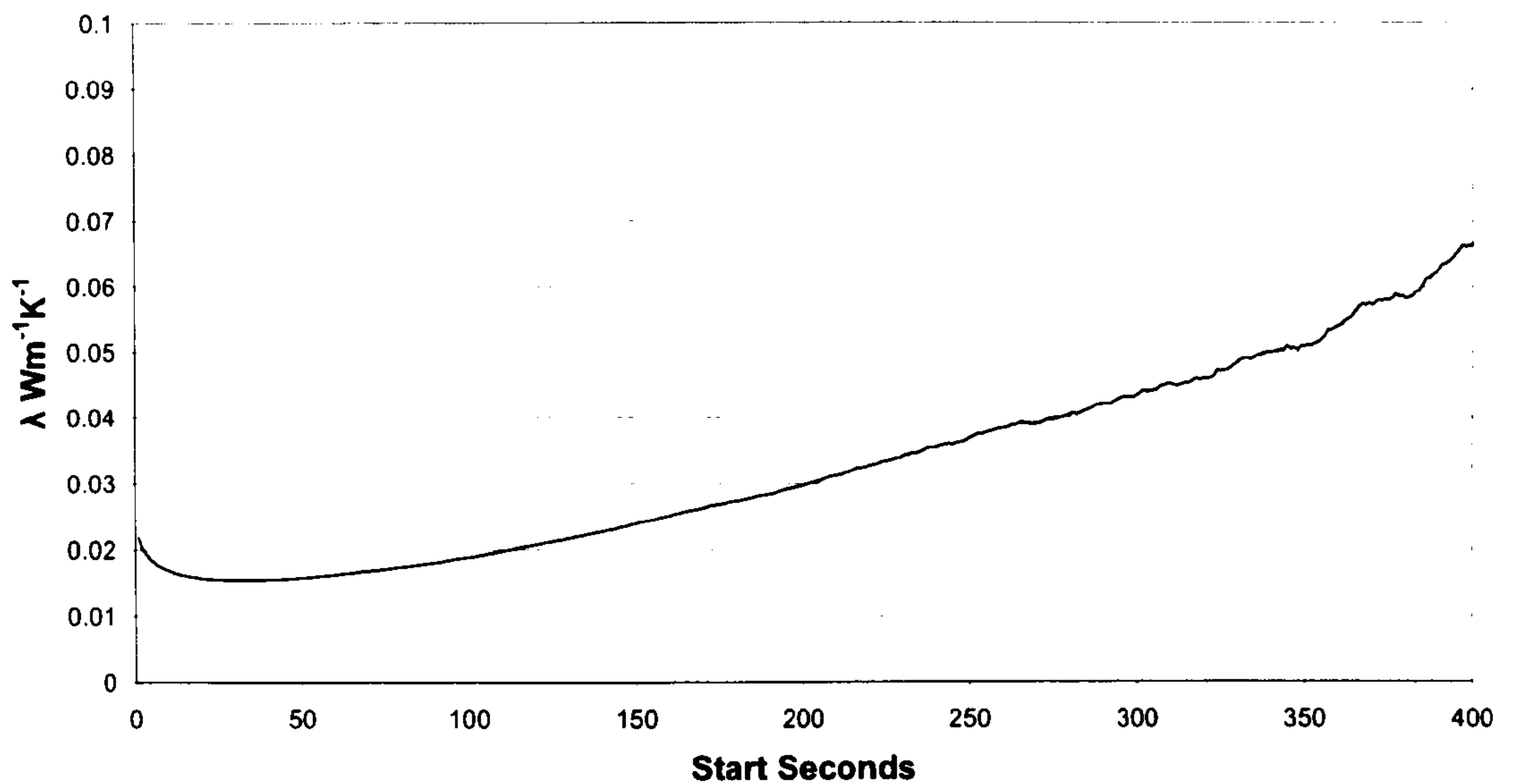
Chart 61: Thermal conductivity 100s results for a phenolic foam sample
