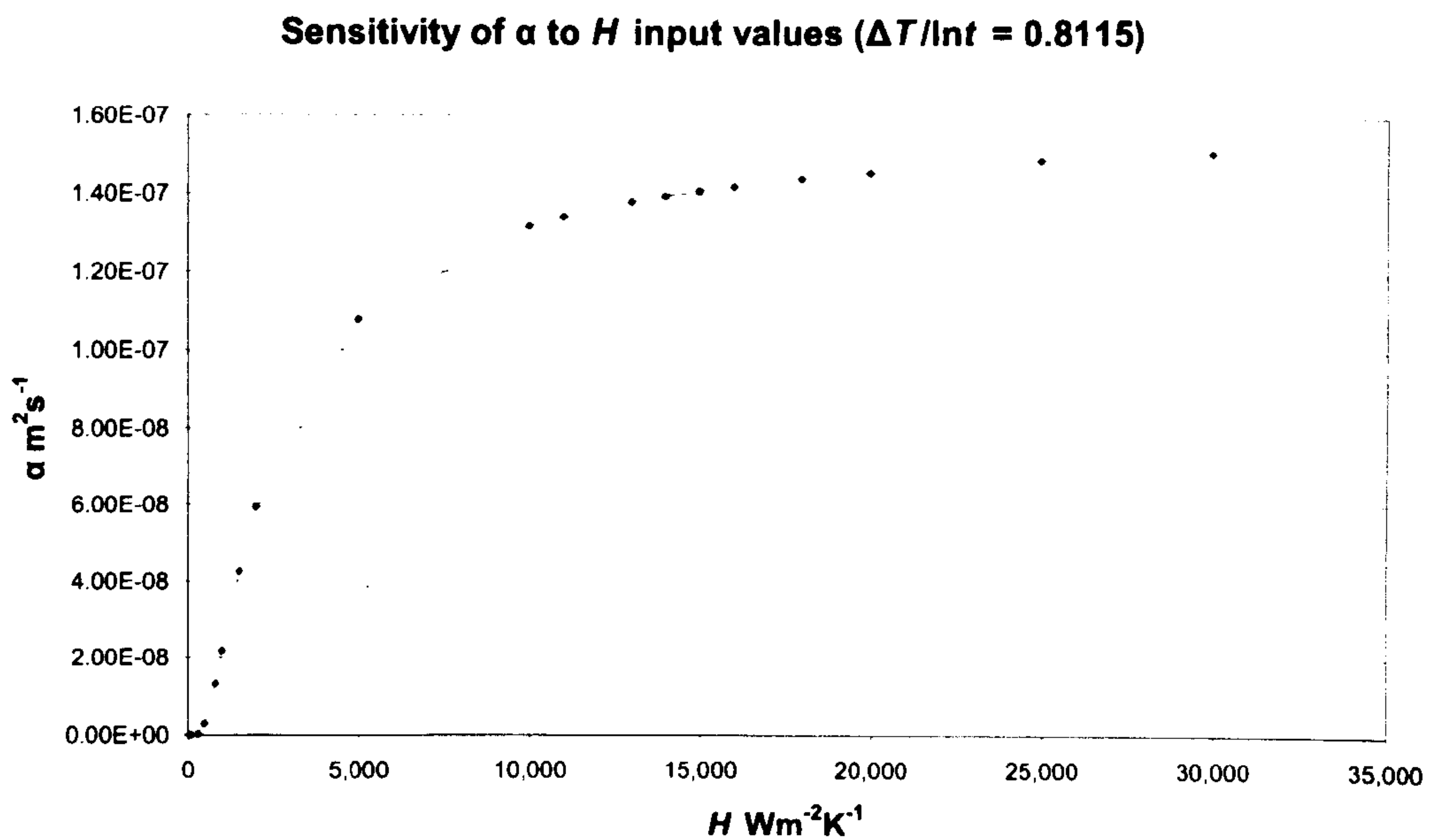
Chart 2: Thermal diffusivity by contact resistance estimates, larger H
