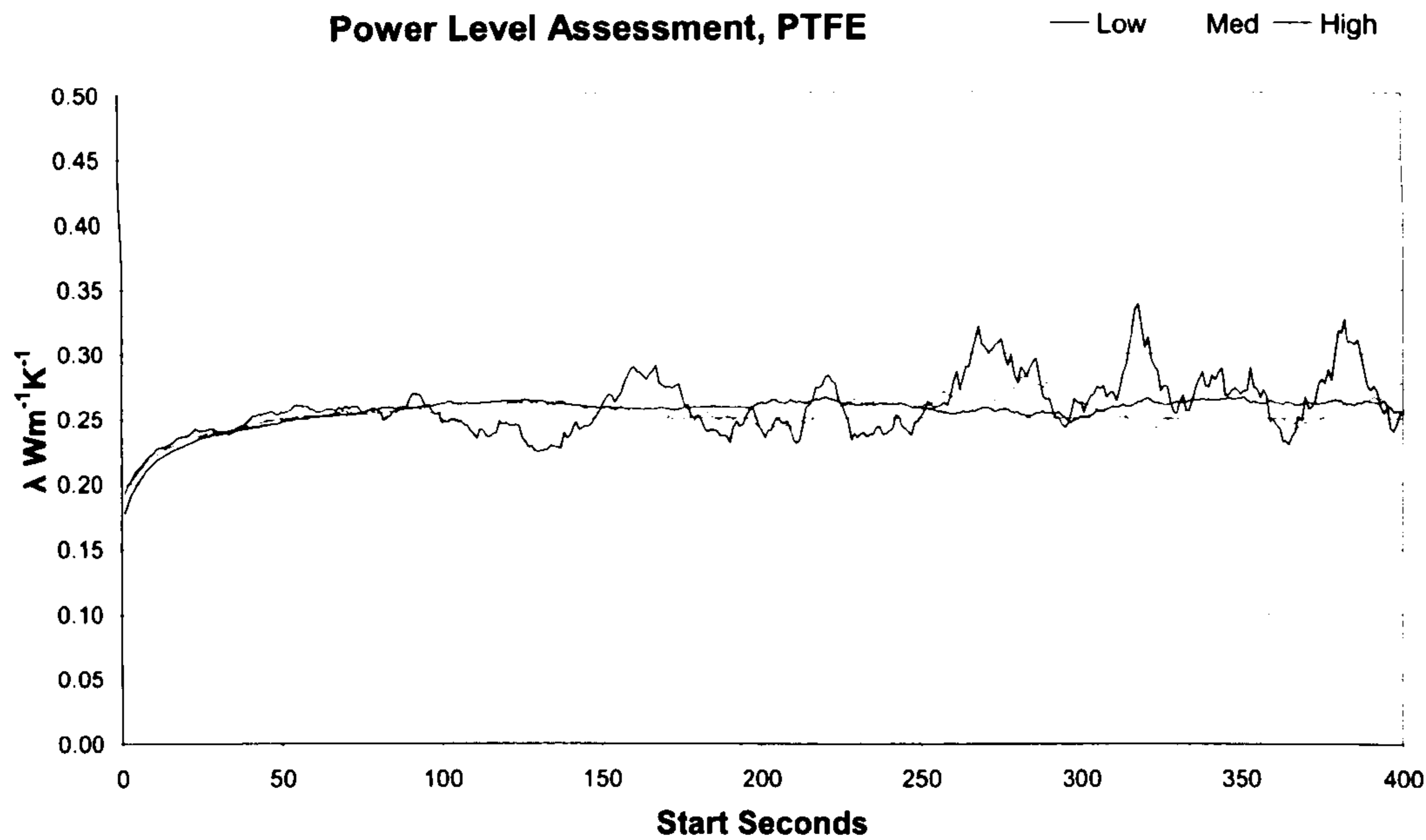
Chart 24: Thermal conductivity, PTFE at three power levels, 100s windows
