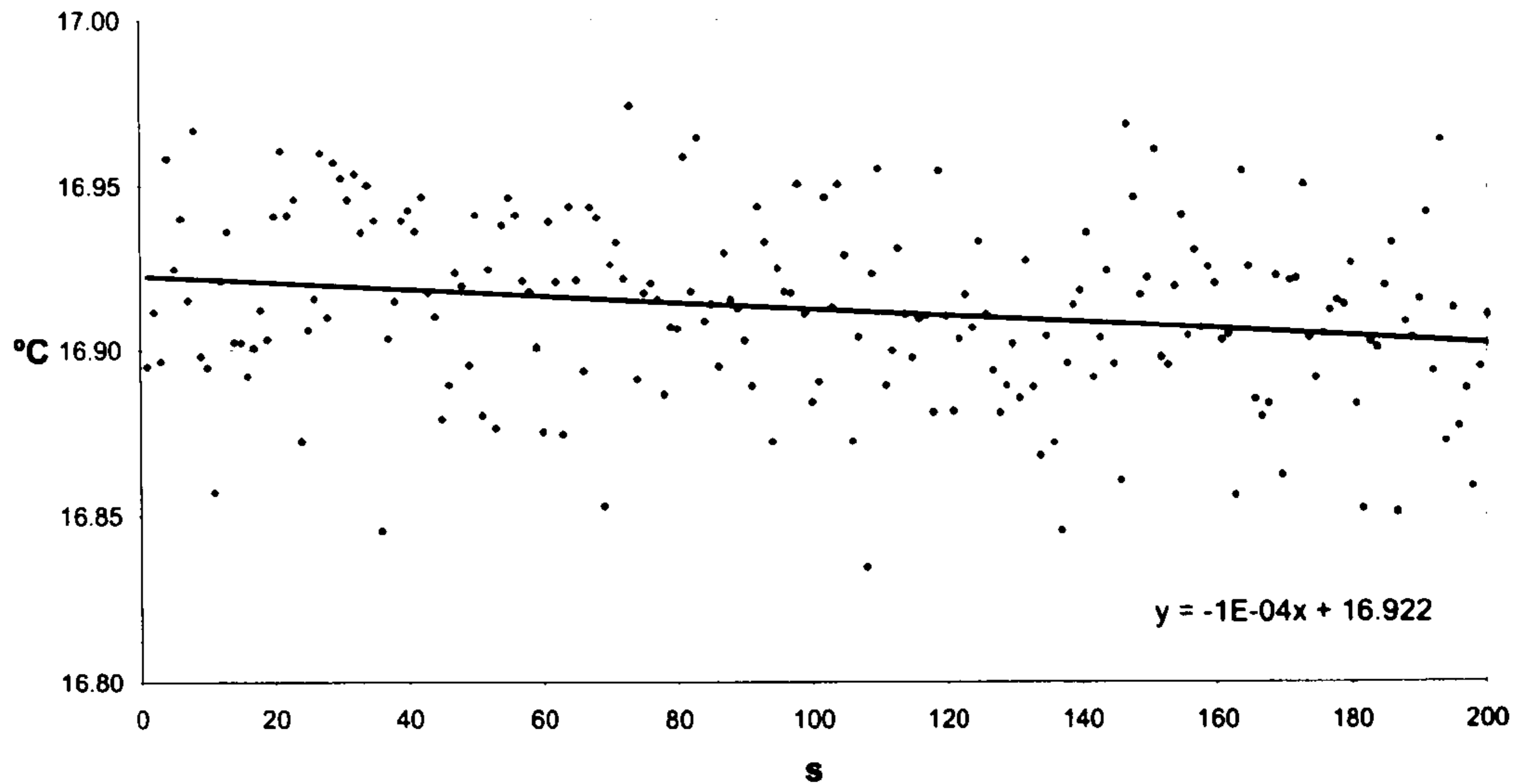
Chart 19: Temperature equilibrium from 500s after probe insertion
