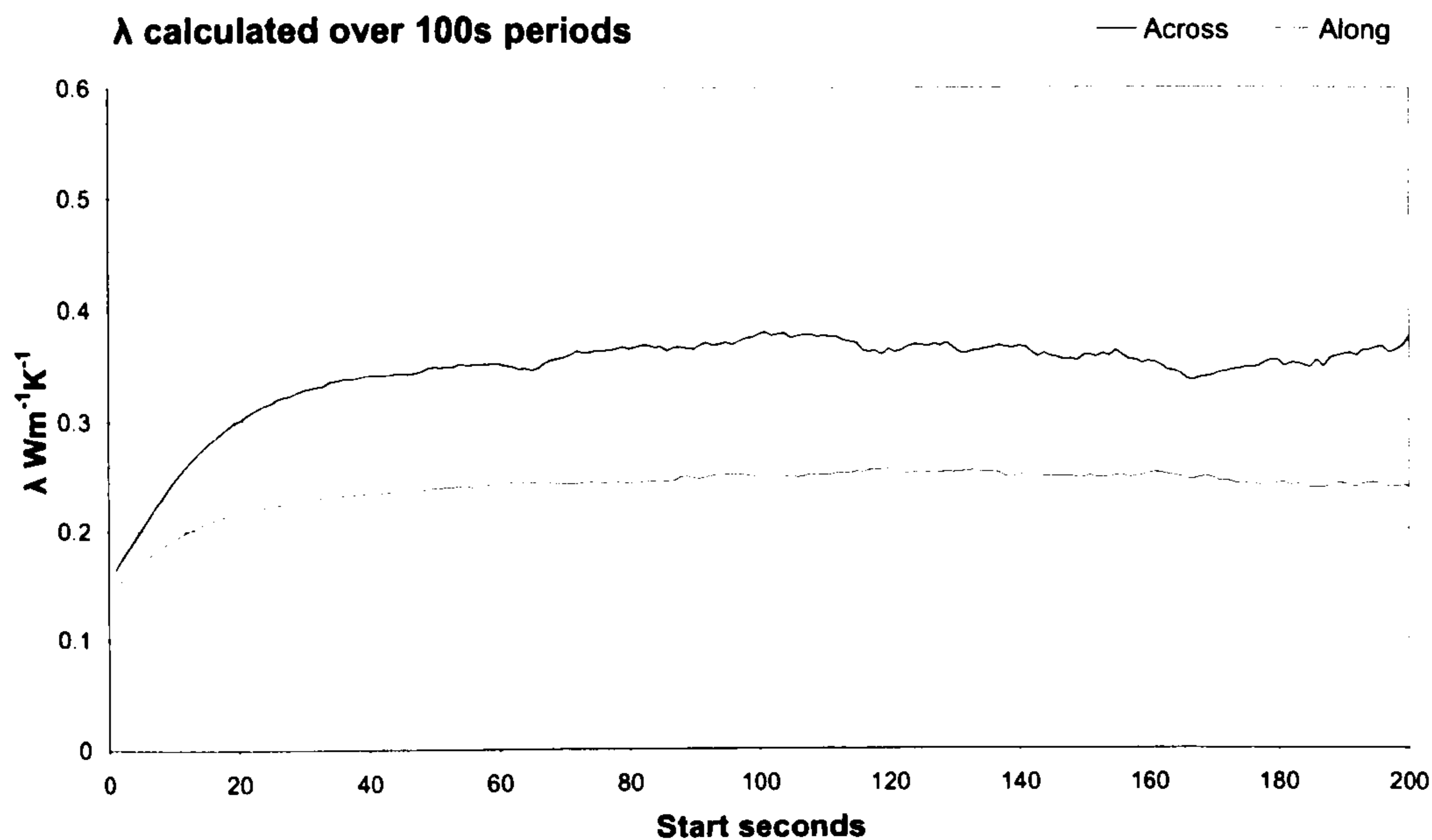
Chart 22: Thermal conductivity, oak, measured across and along the grain
