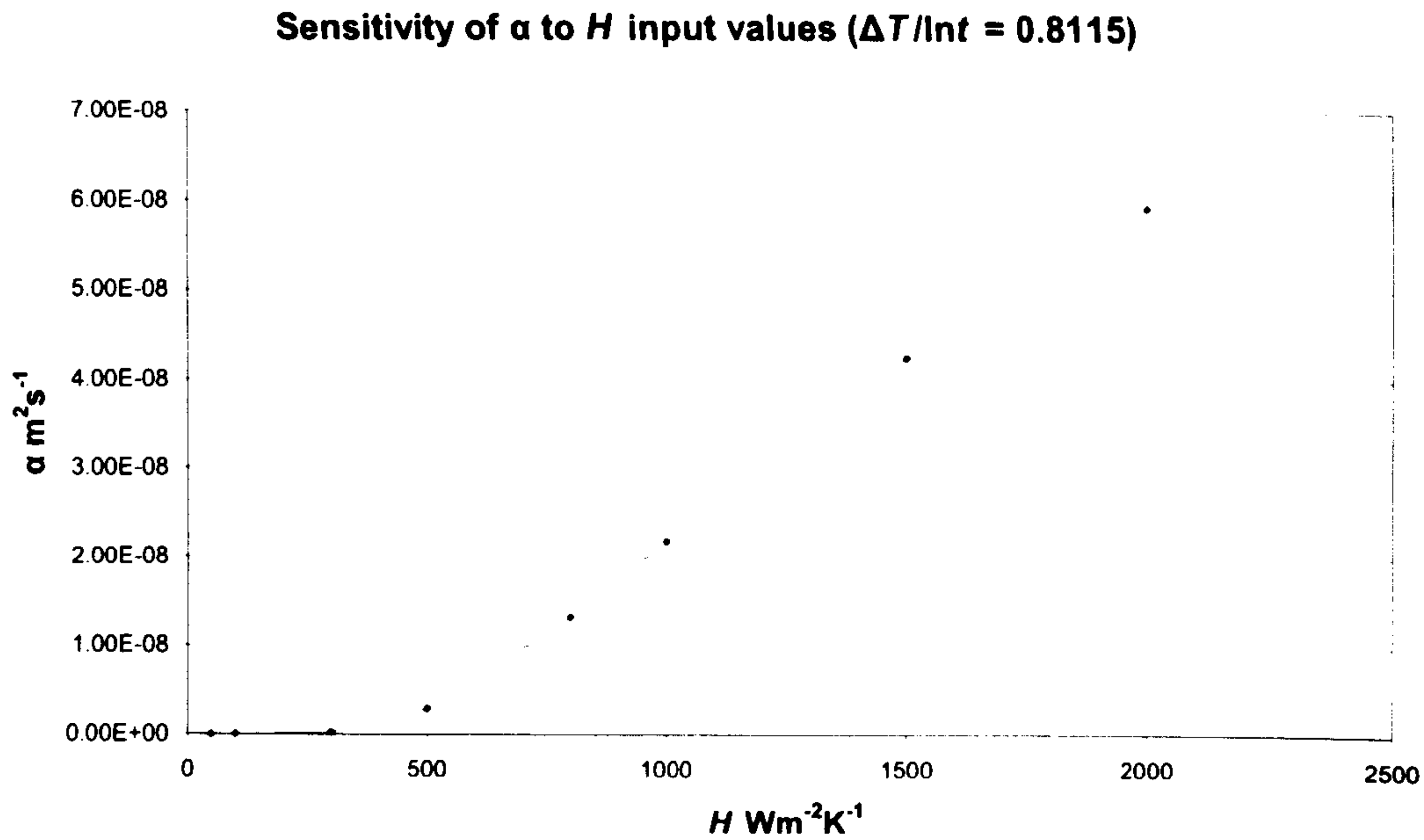
Chart 1: Thermal diffusivity by contact resistance estimates, smaller H
