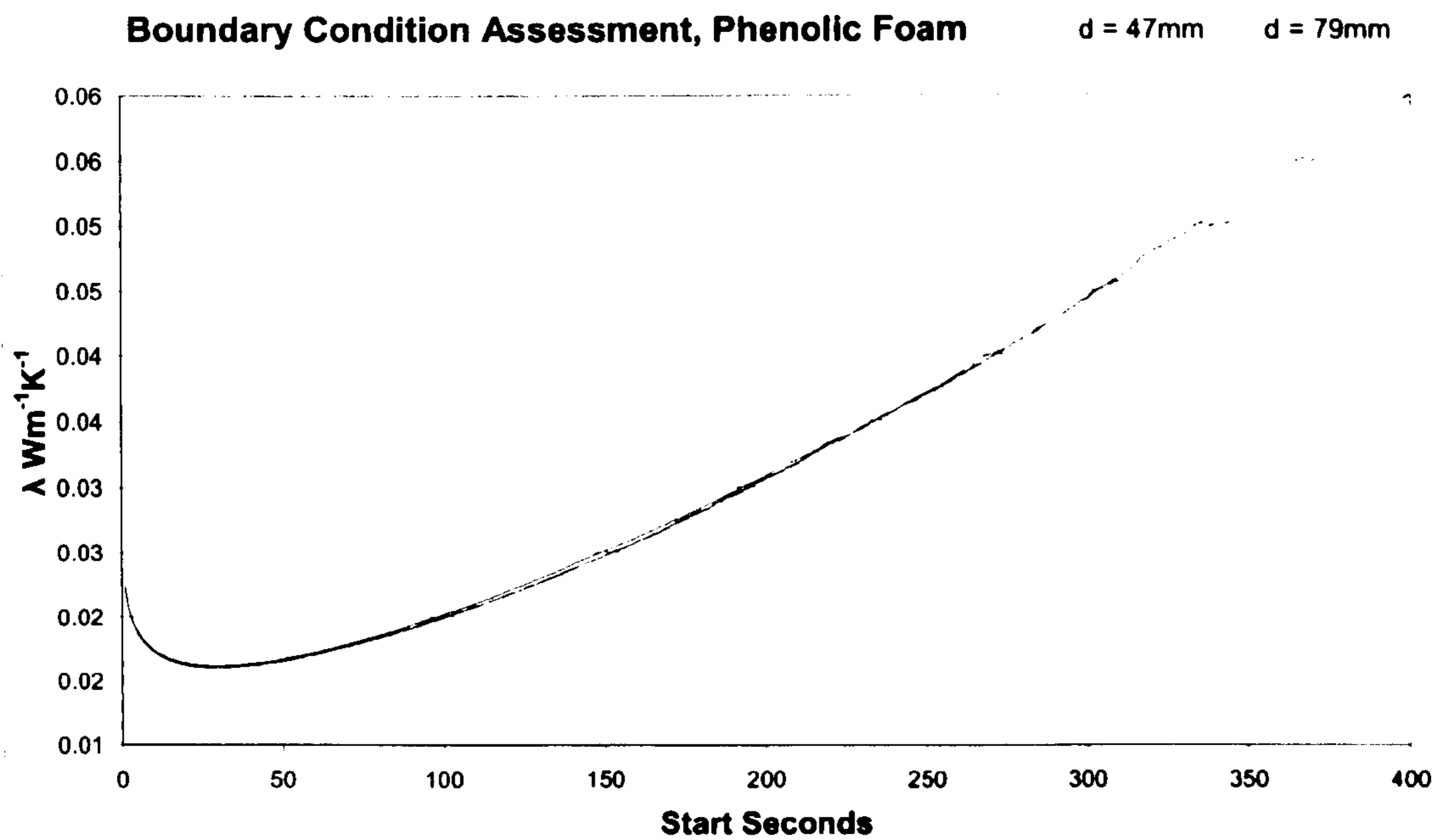
Chart 32: Thermal conductivity, phenolic foam at two thicknesses
