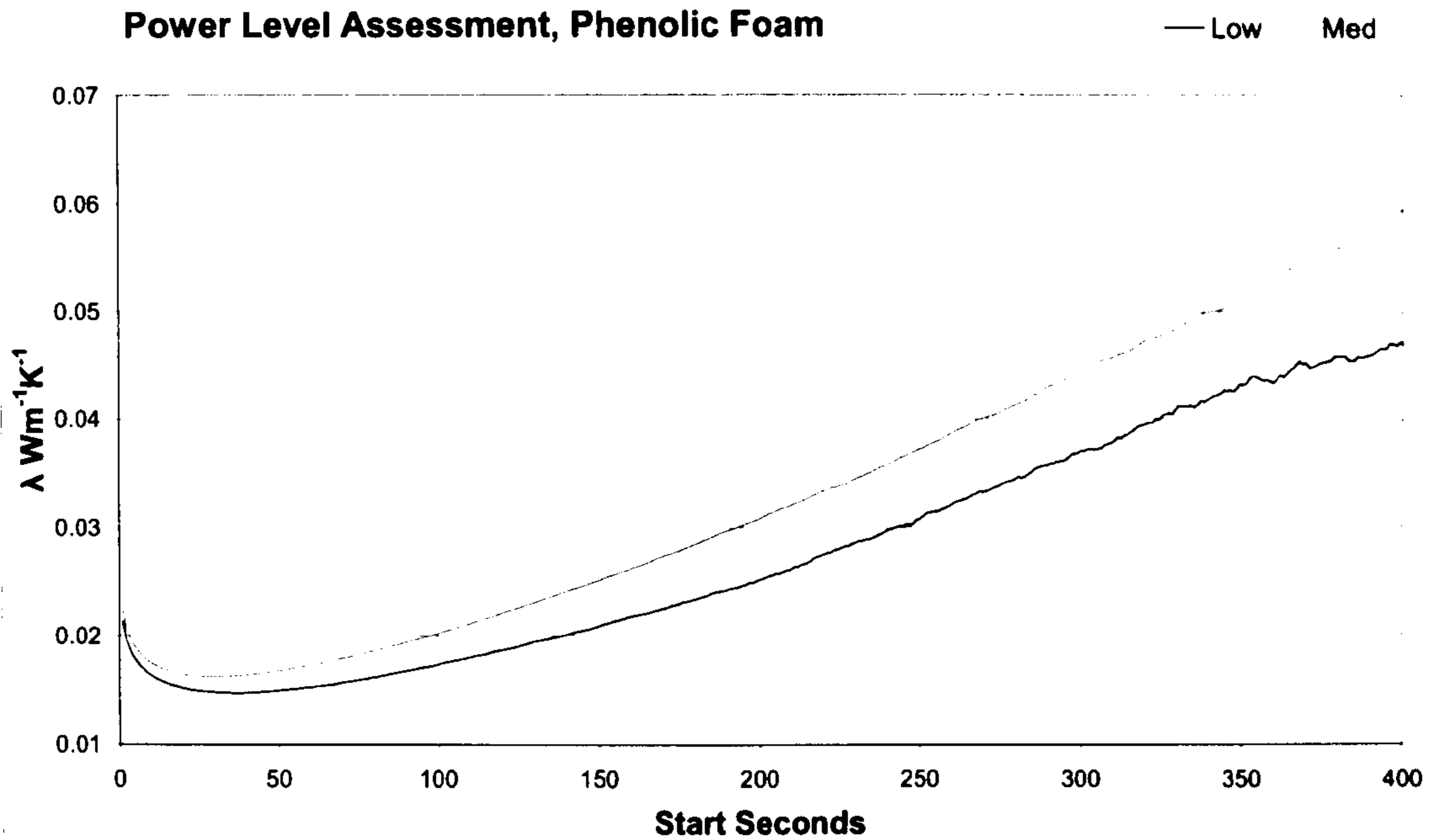
Chart 25: Thermal conductivity, phenolic foam at two power levels, 100s windows
