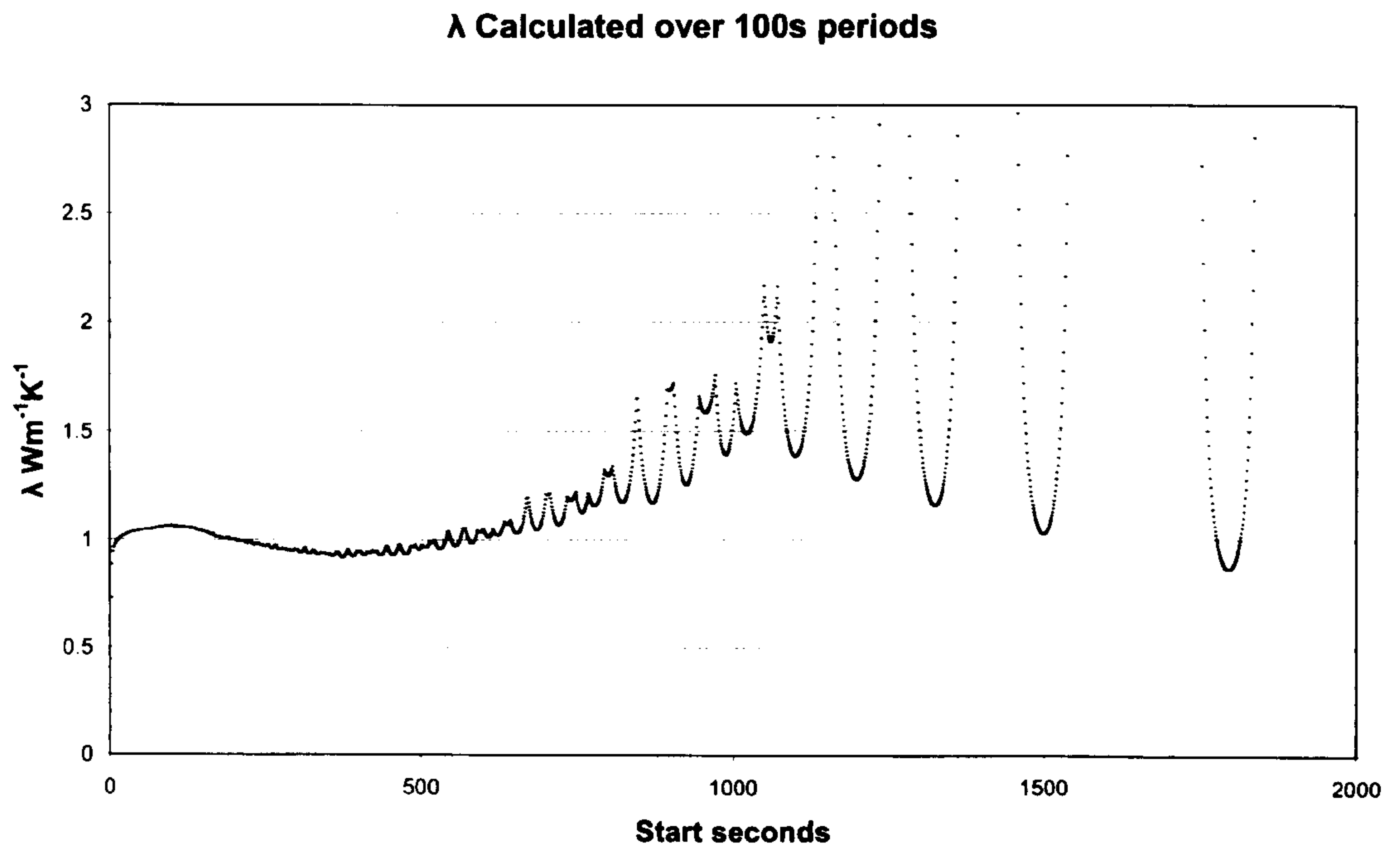
Chart 58: Voltra 100s results for 1.0 \text{ Wm}^{-1}\text{K}^{-1} , 100 \text{ kJm}^{-3}\text{K}^{-1}
