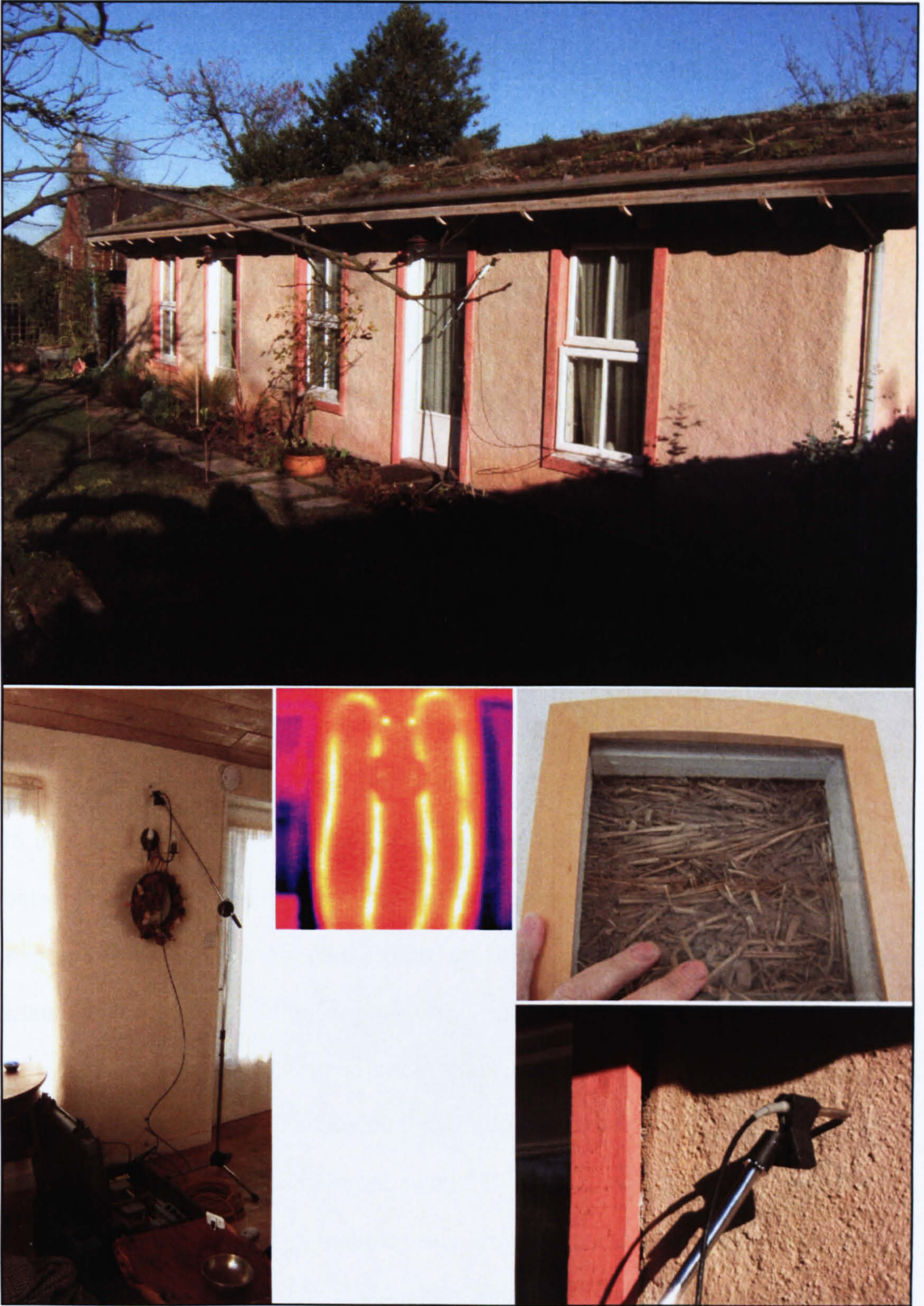
Figure 25: Clay straw studio, Scottish Borders
