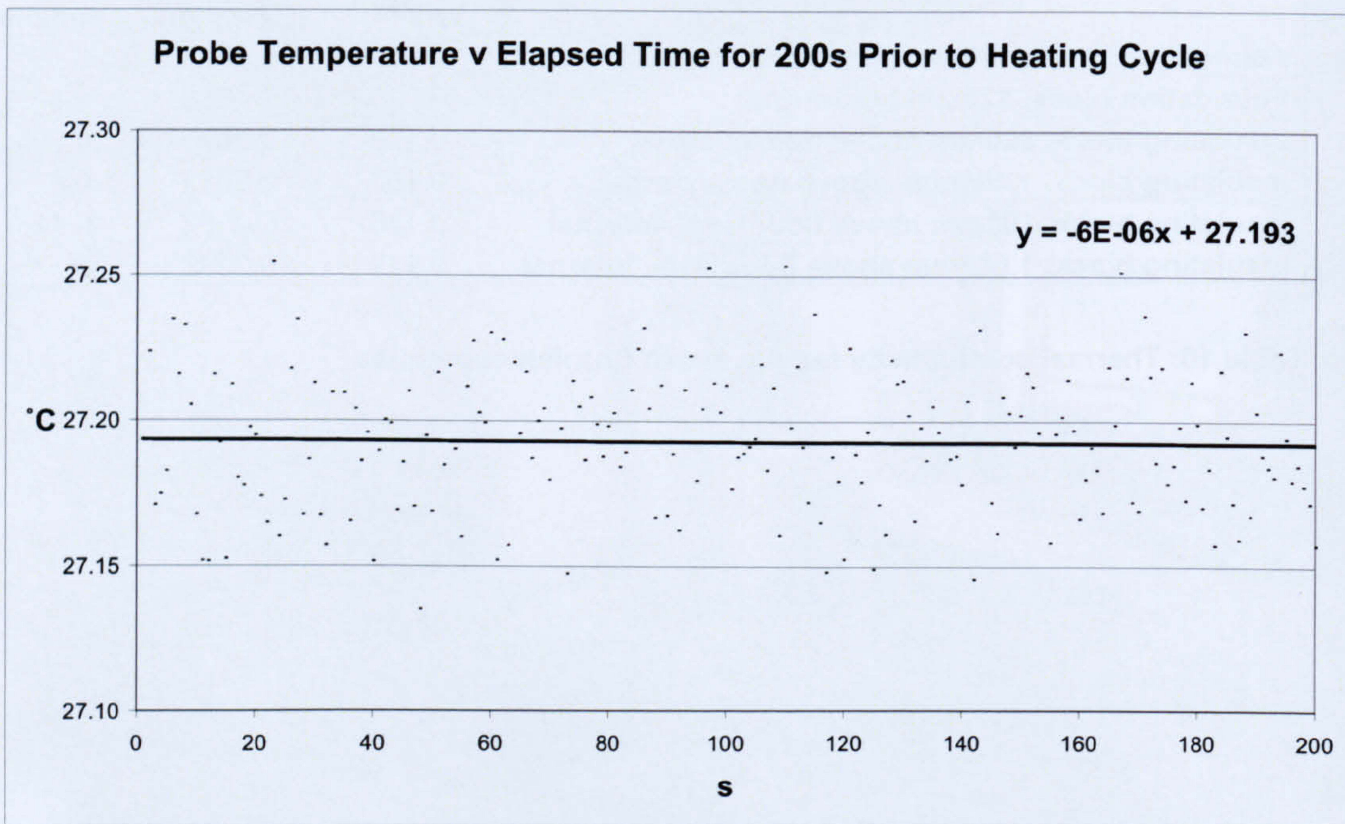
Chart 48: Temperature stability prior to the measurement in chart 56
