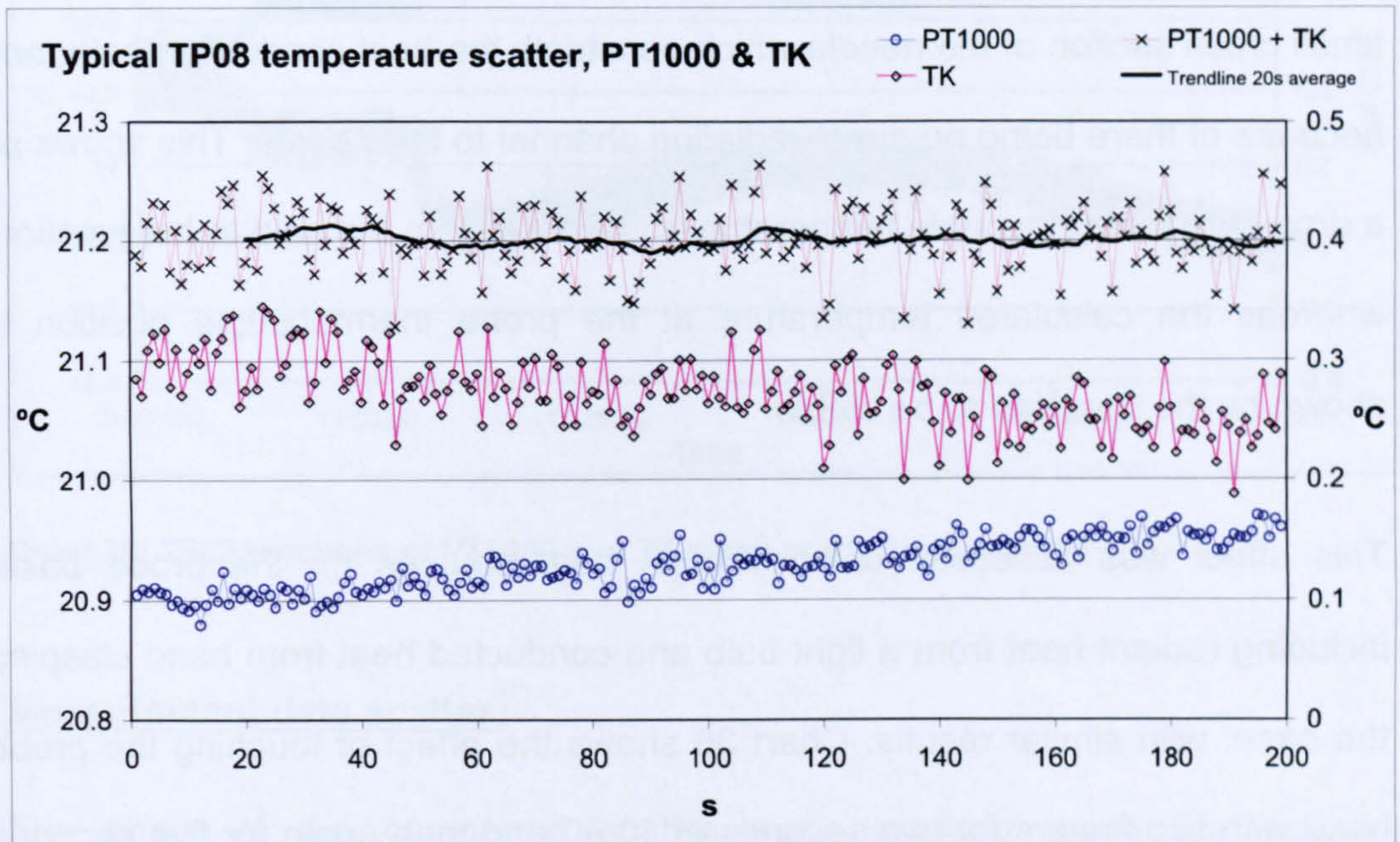
Chart 37: Data scatter in TP08 temperature measurements
