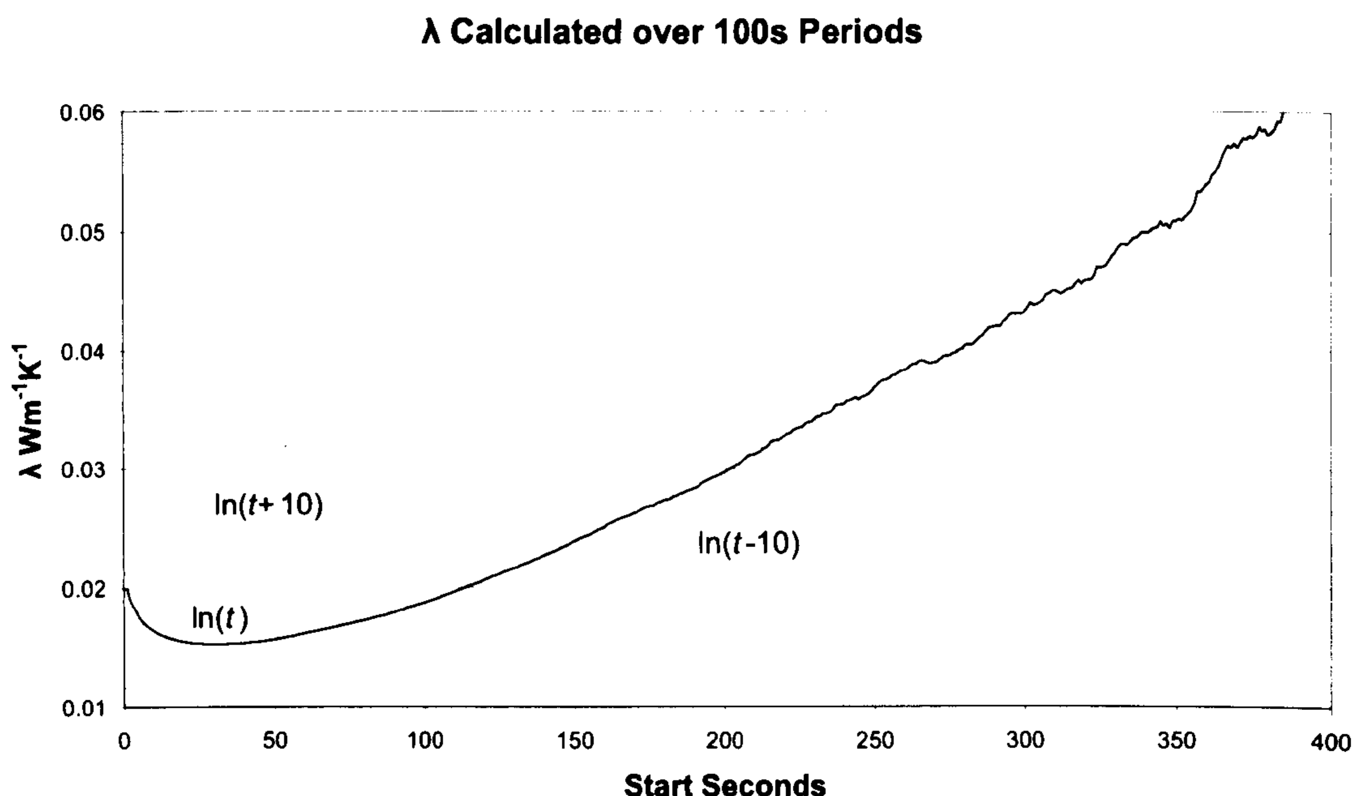
Chart 8: \lambda for phenolic foam over 100s intervals, t offset by \pm 10 s
