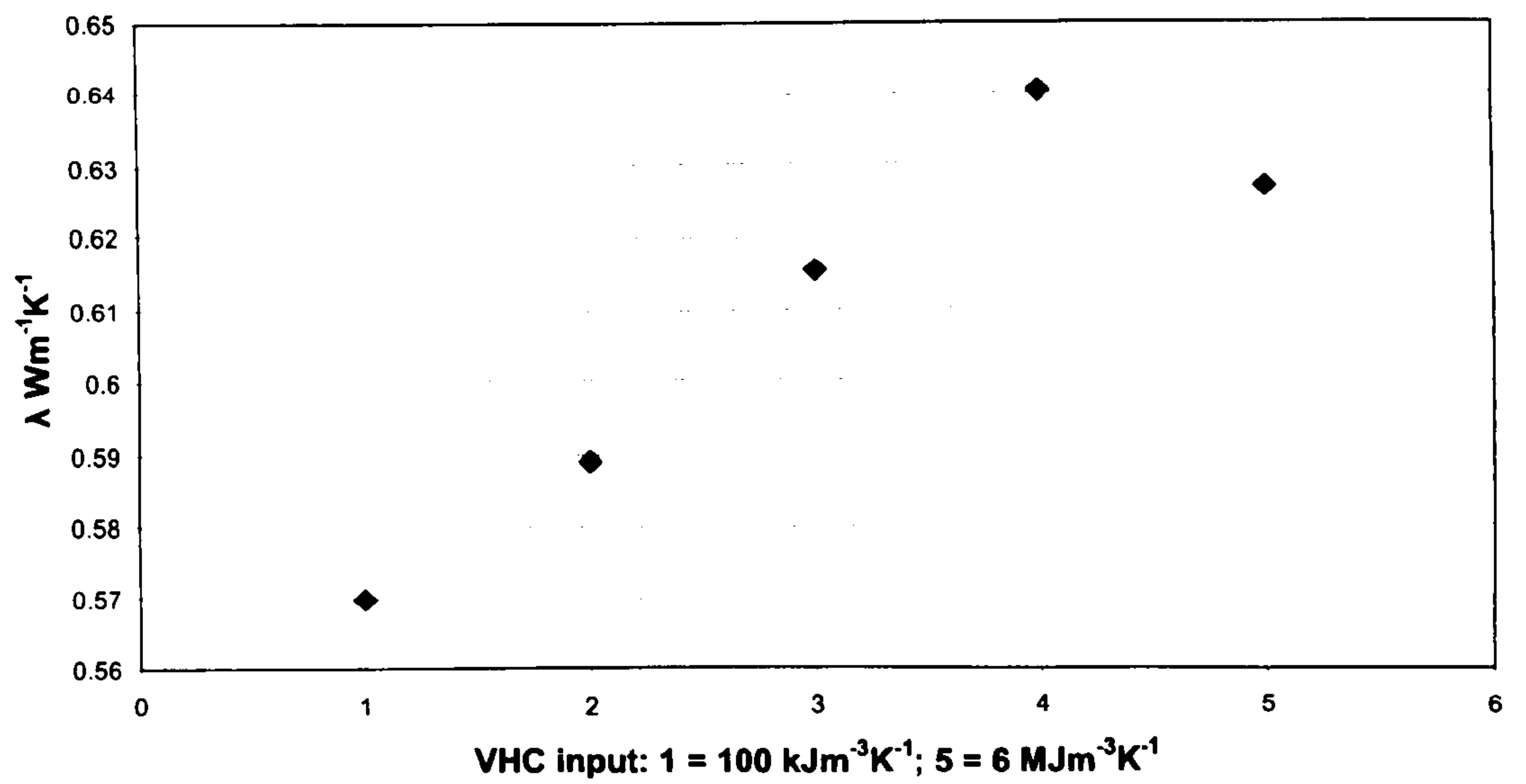
Chart 56: Voltra thermal conductivity outcomes for 0.6 Wm -1 K -1 input, varied pC
