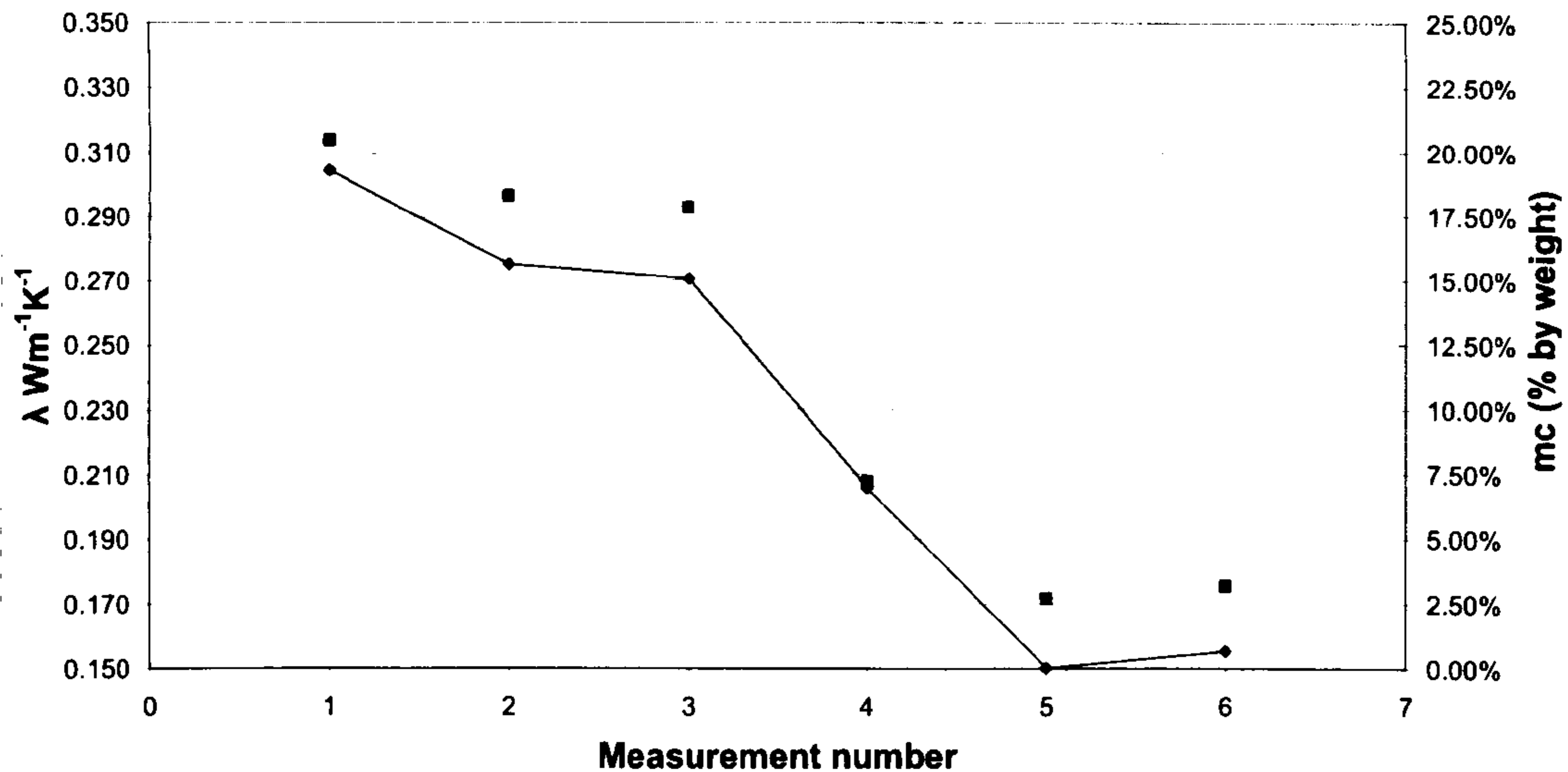
Chart 36: Thermal conductivity, aerated concrete, varied moisture content
