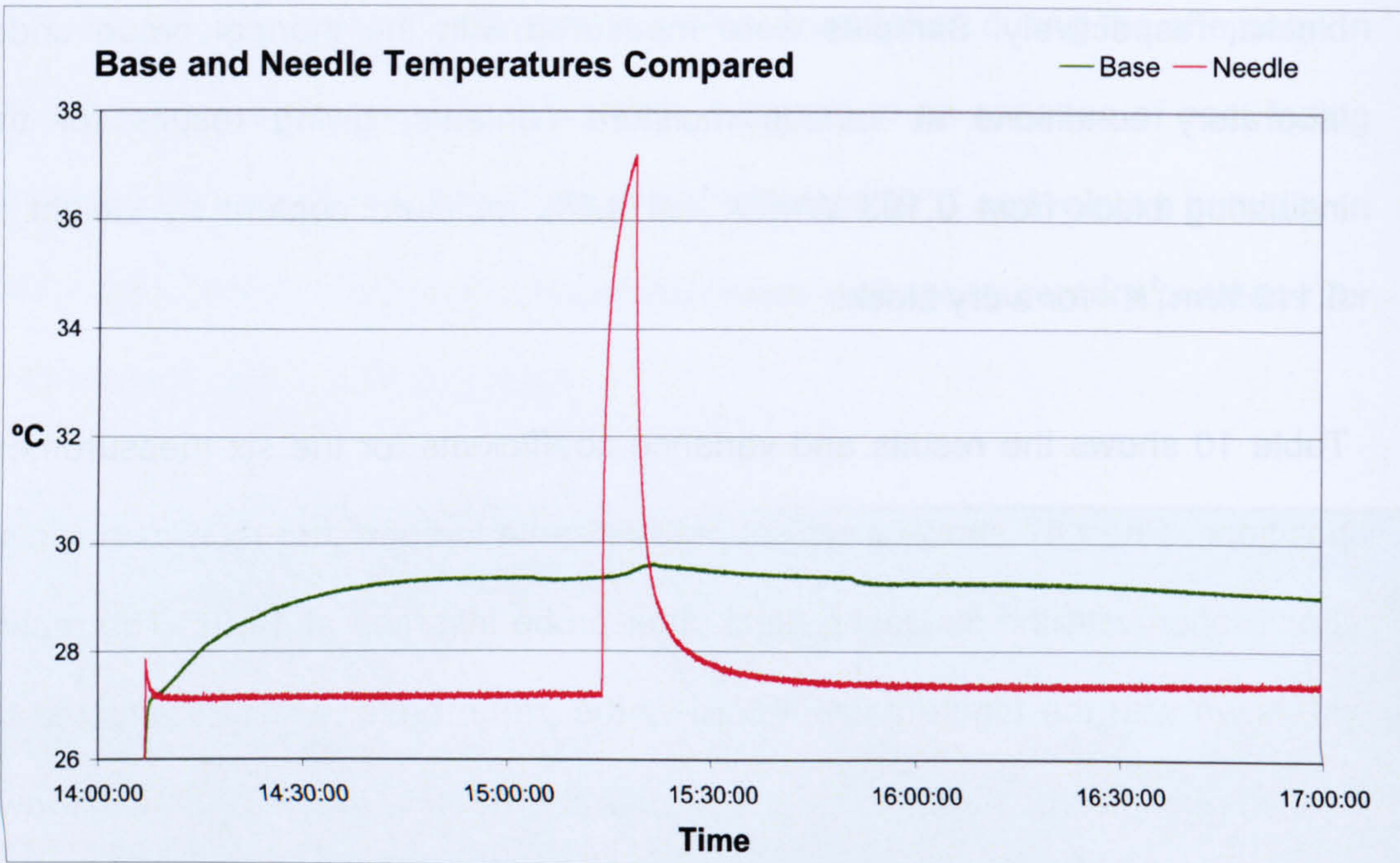
Chart 47: Temperature record of probe base and needle, aerated concrete, internal
