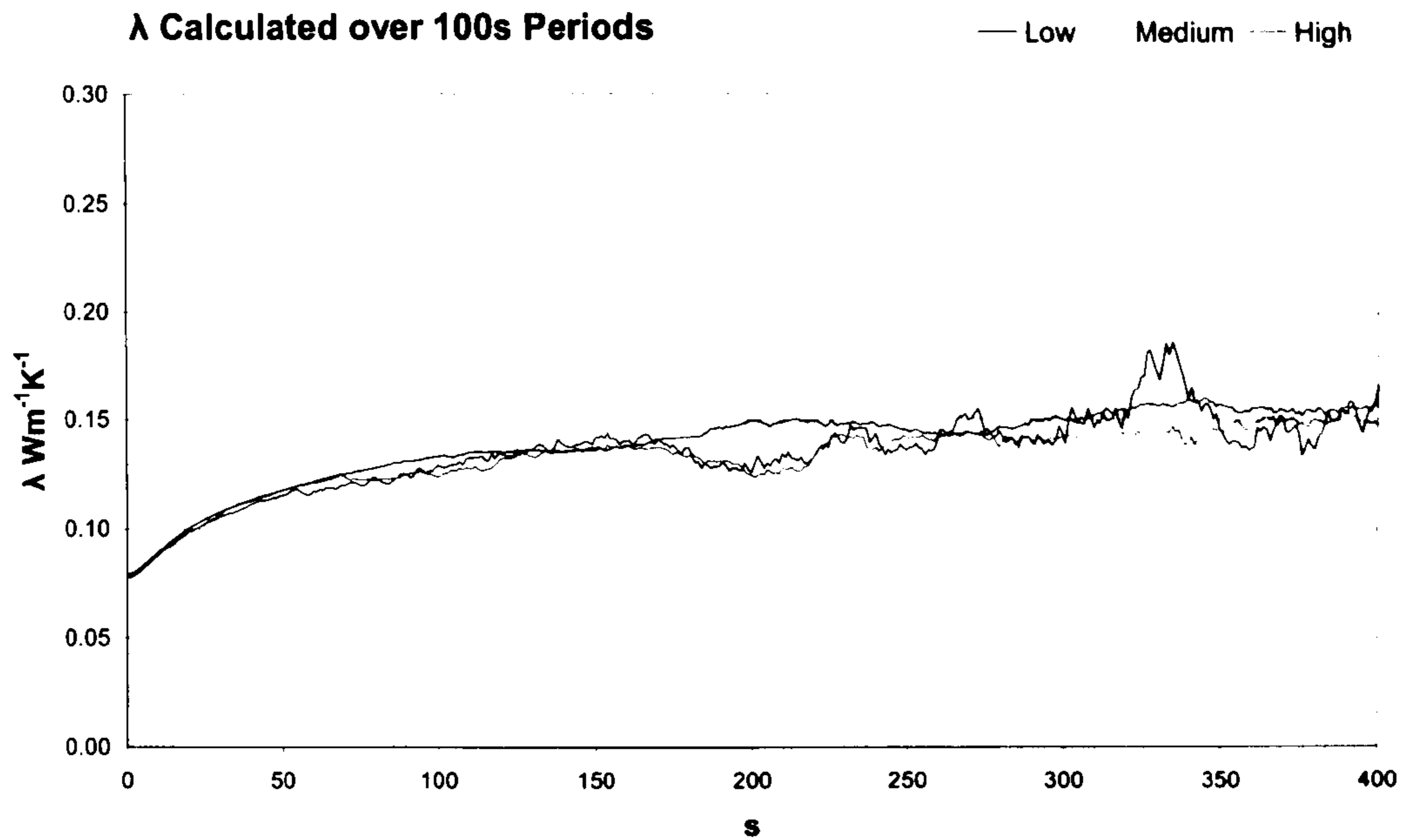
Chart 27: Thermal conductivity results for aerated concrete at three power levels
