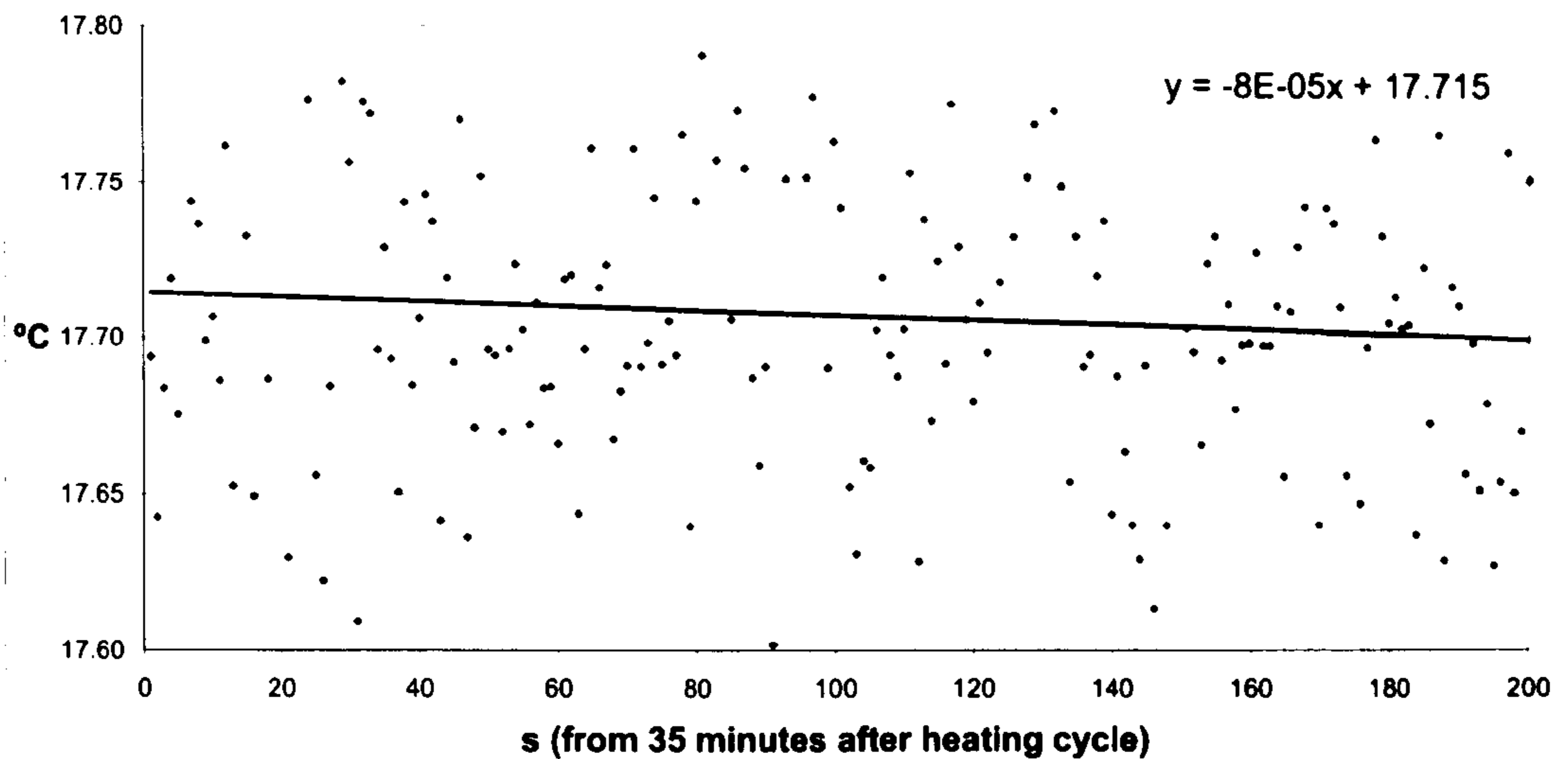
Chart 21: Temperature equilibrium in aerated concrete after a heating cycle
