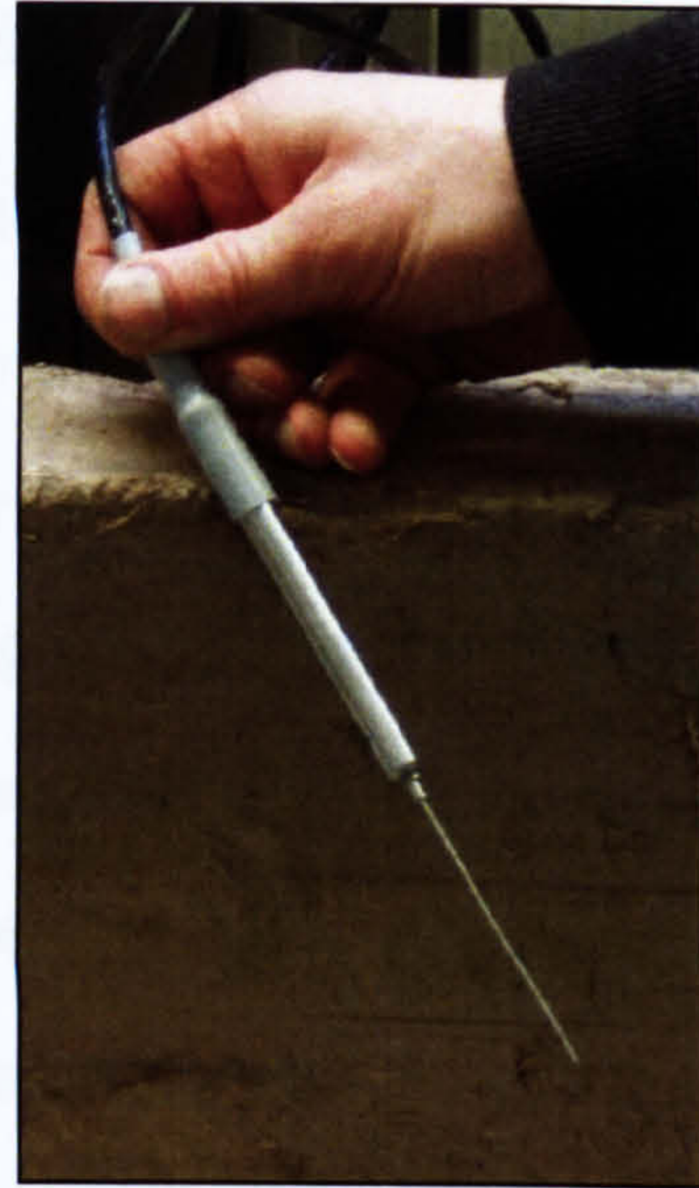
Figure 2: A Hukseflux TP08 thermal probe
