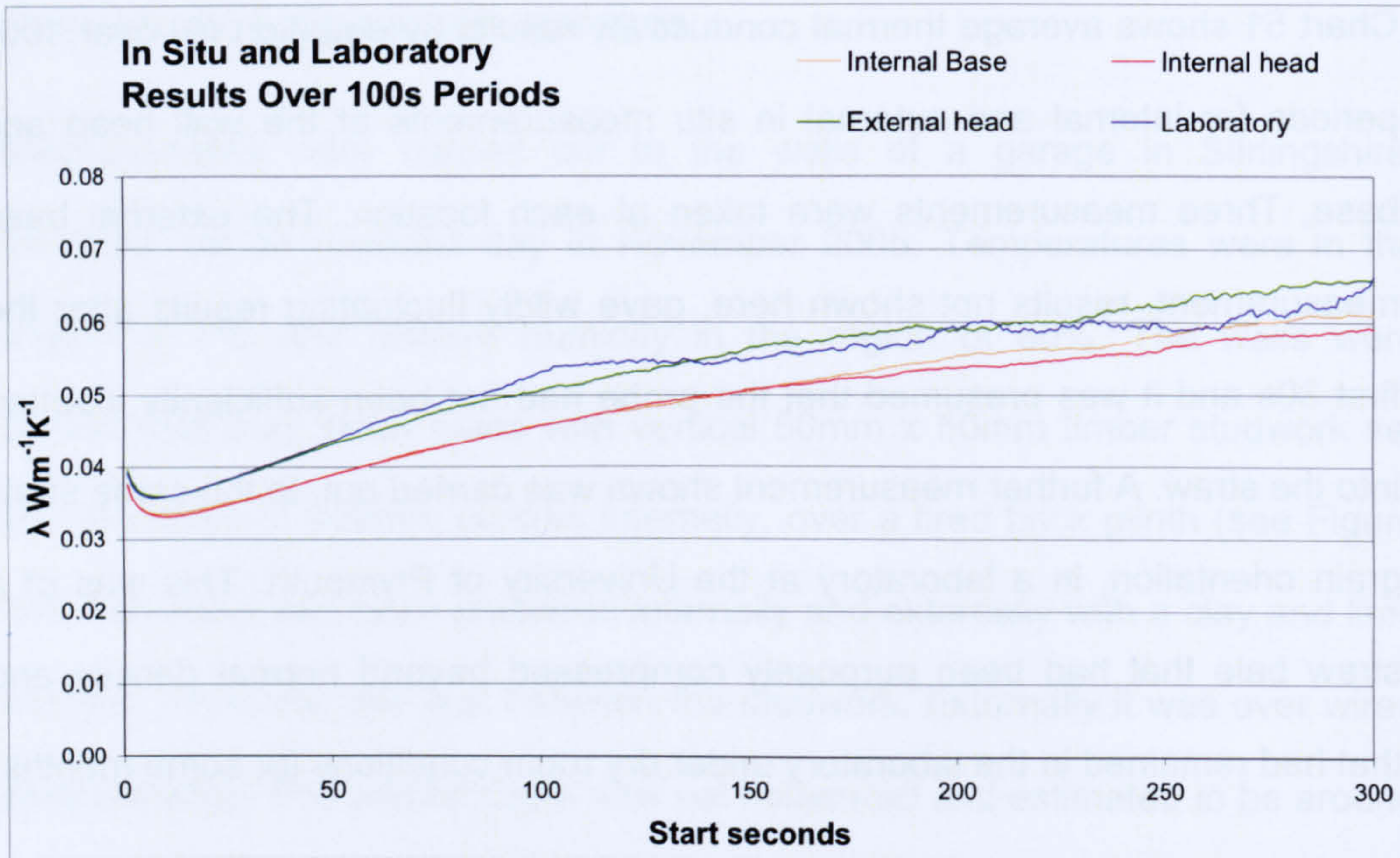
Chart 51: In situ and laboratory results for straw bale construction
