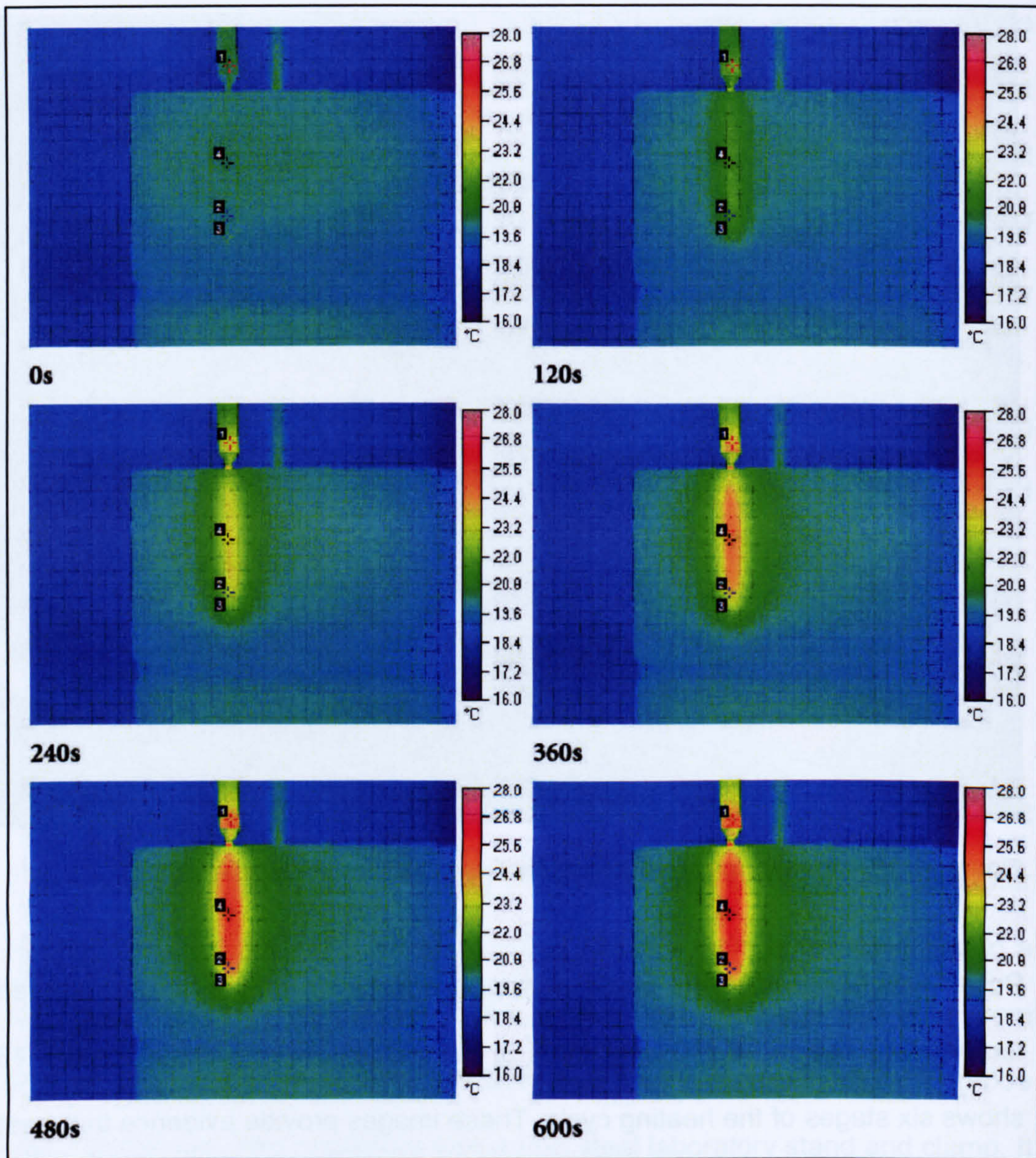
Figure 15: Thermal images of a probe heating profile in aerated concrete
