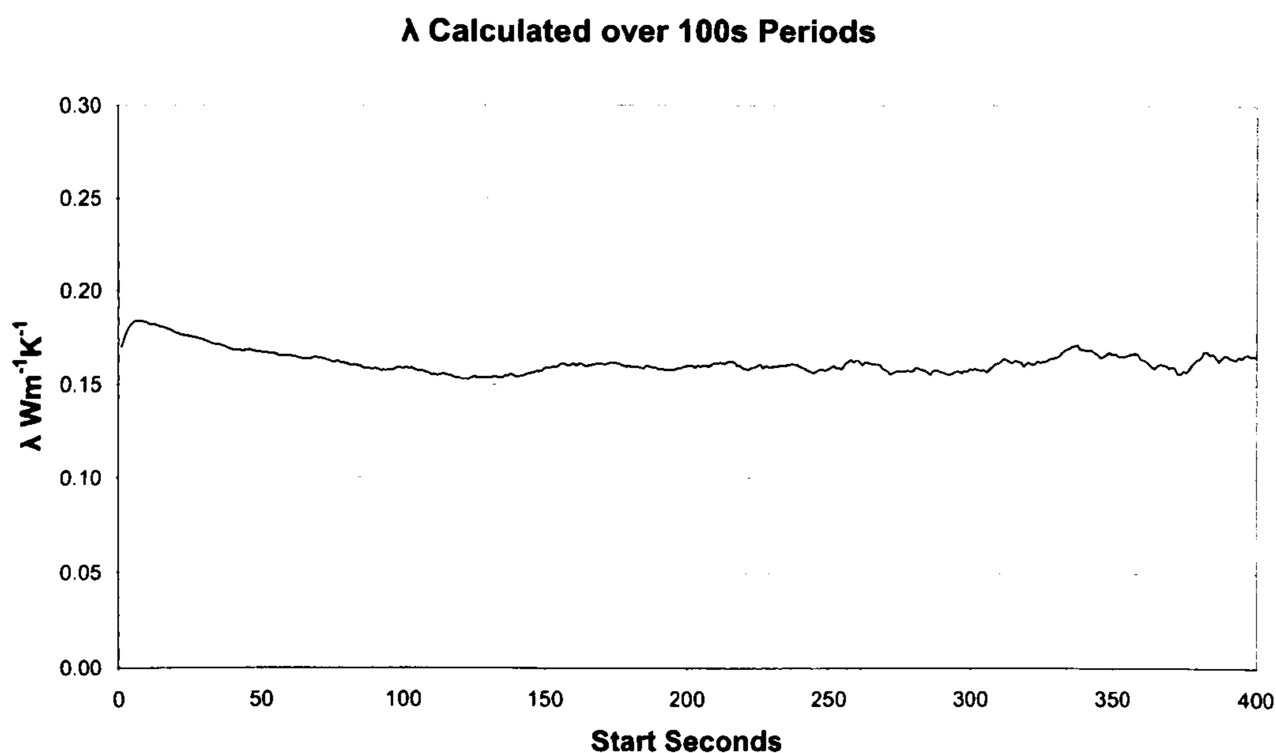
Chart 33: Thermal conductivity results for aerated concrete after oven drying
