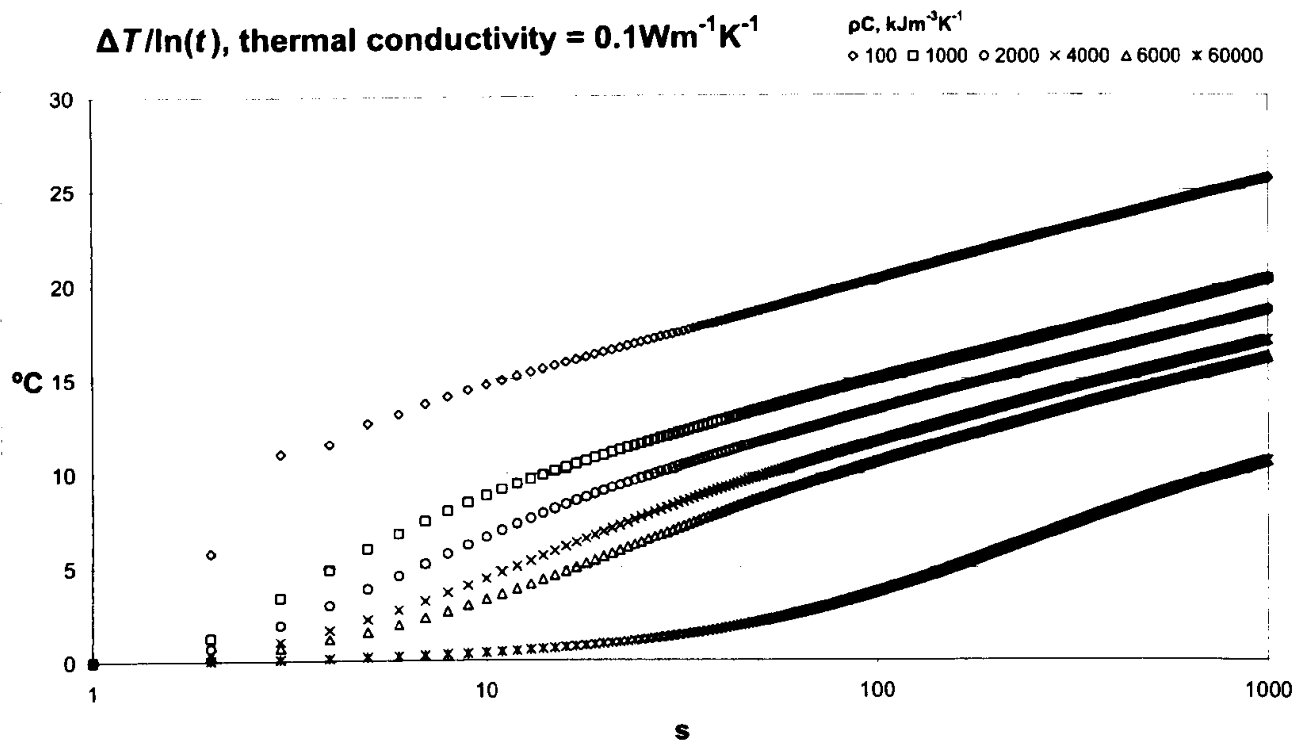
Chart 54: Voltra temperature rises for 0.1 \text{ Wm}^{-1}\text{K}^{-1} thermal conductivity
