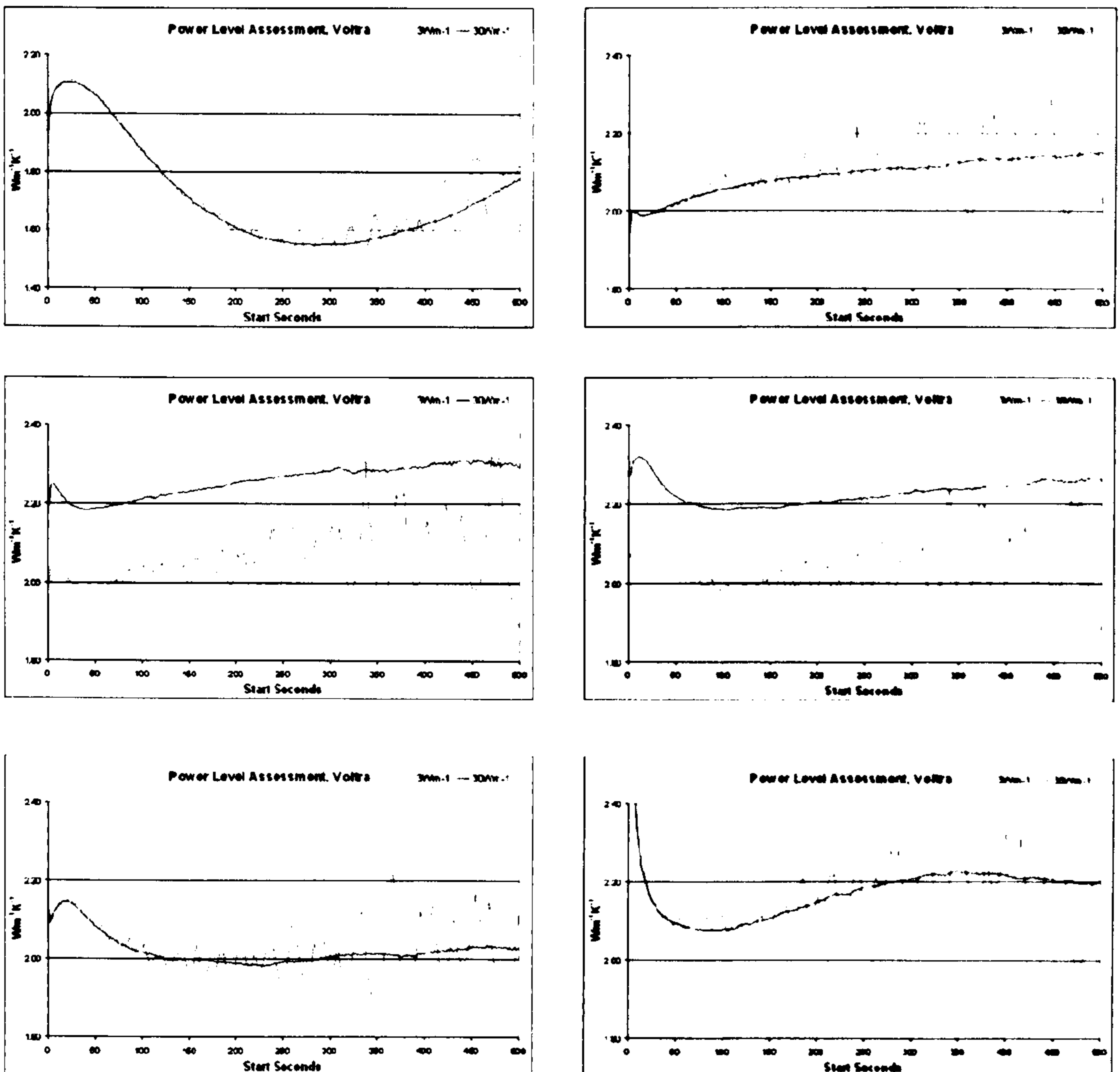
Figure 13: Voltra output \lambda from: 2.0 \text{ Wm}^{-1}\text{K}^{-1} , varied \rho C , at two powers
