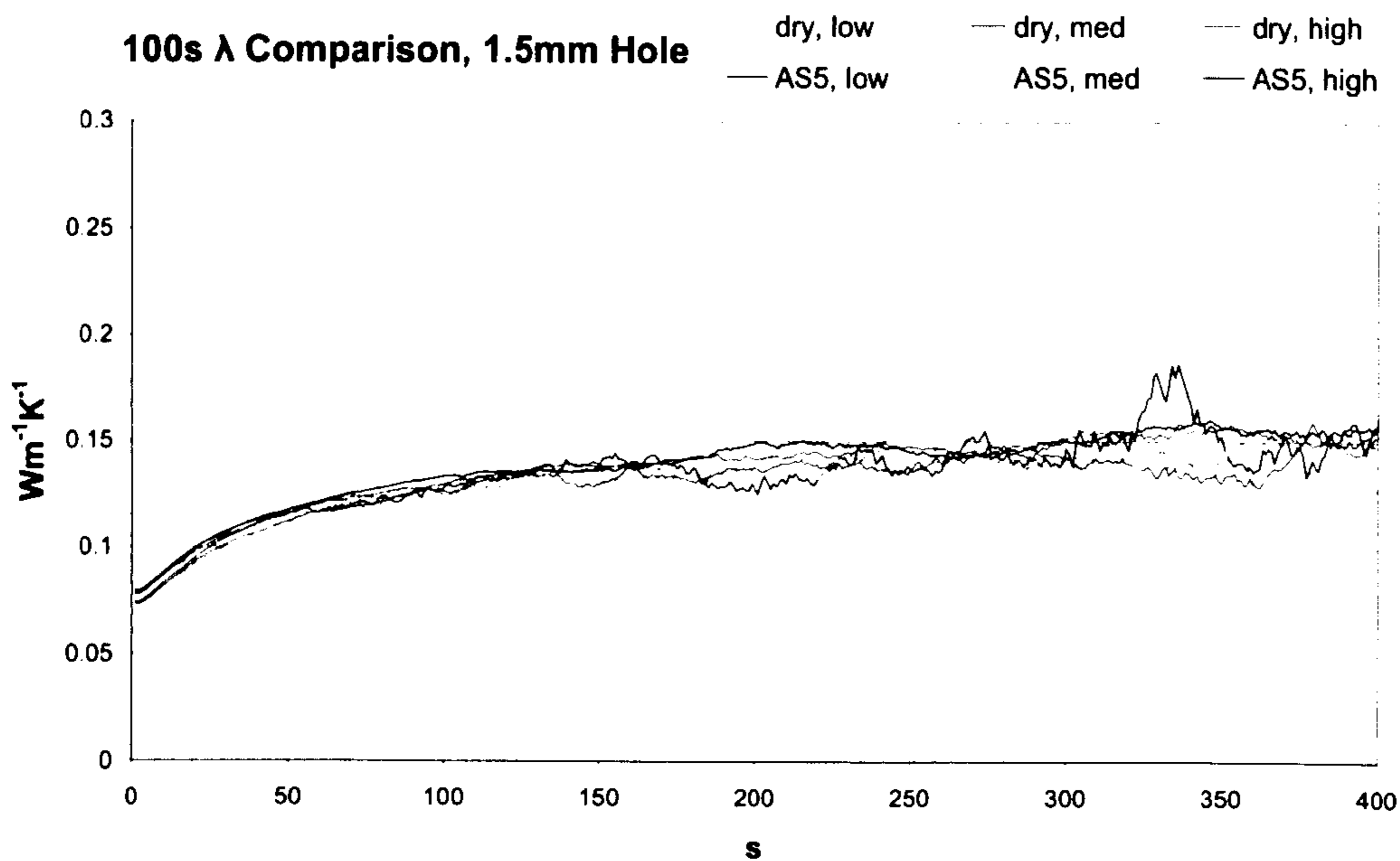
Chart 14: Thermal conductivity results from a 1.5mm hole, aerated concrete
