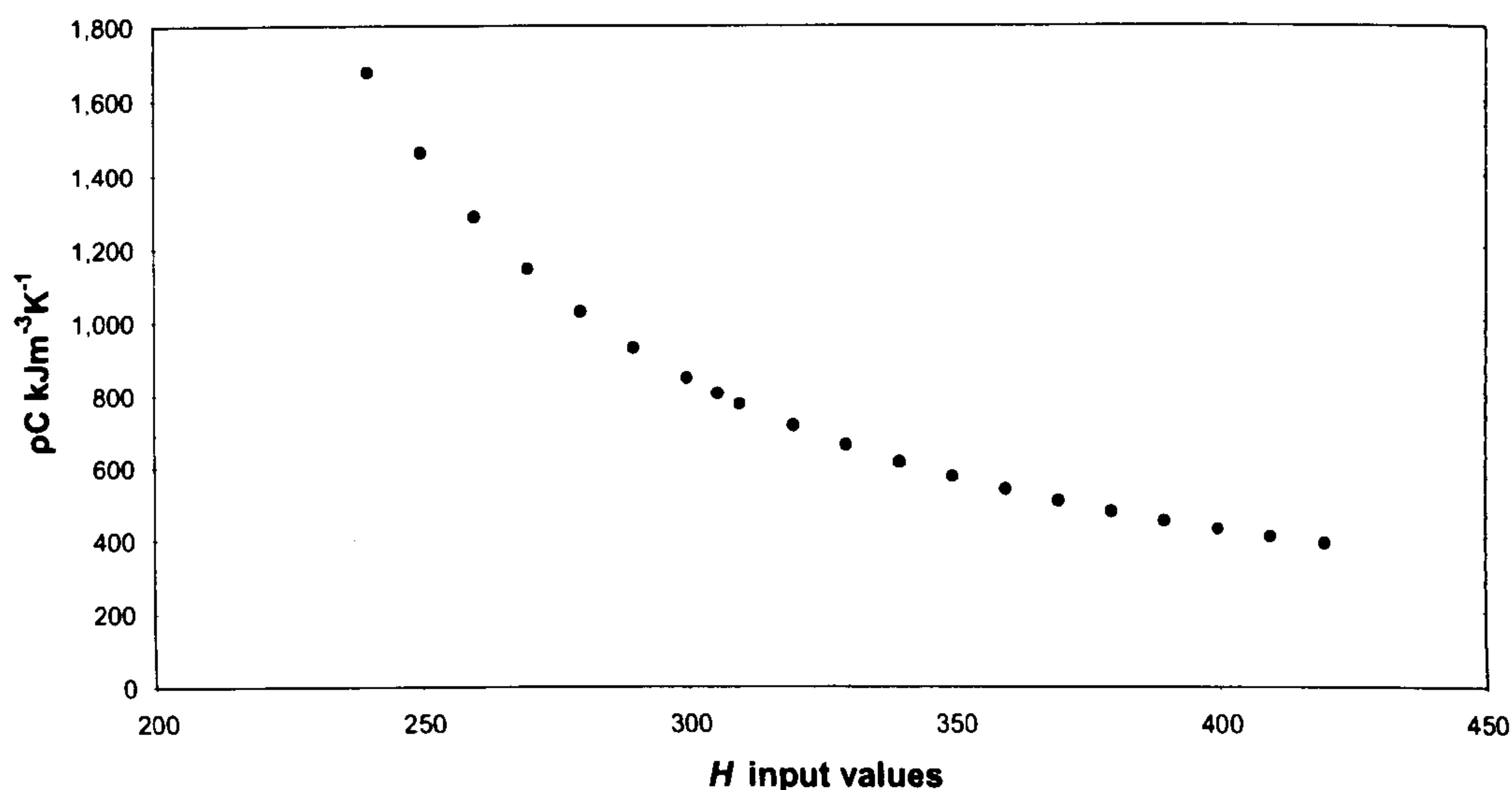
Volumetric heat capacity ( \rho C ) by estimated H value
