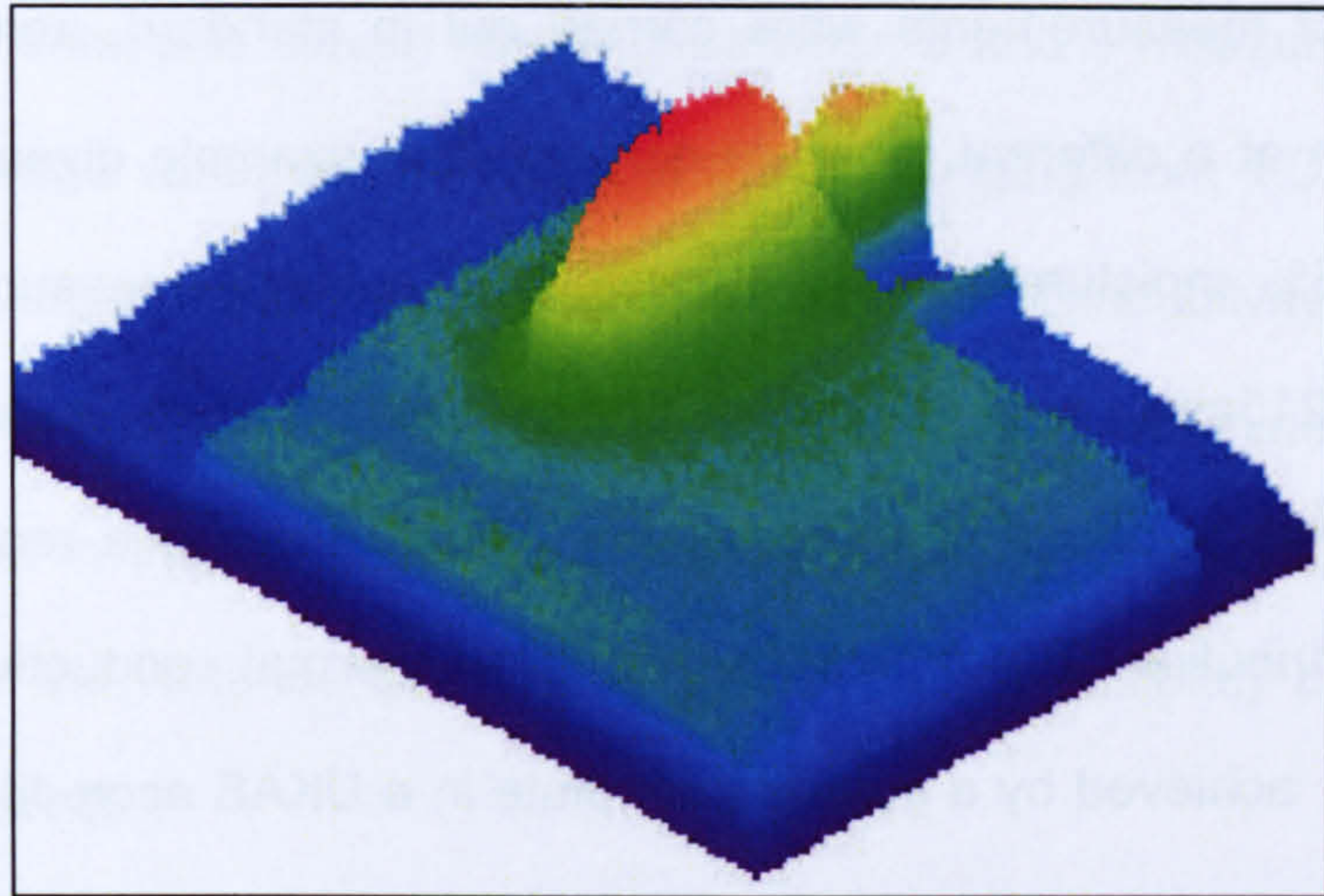
Figure 16: 3D thermal image of a probe heating profile in aerated concrete
