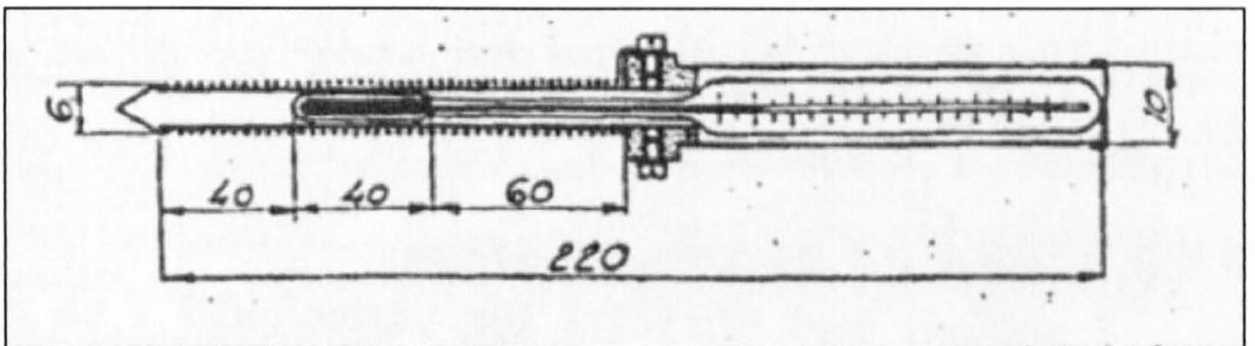
Figure 7: Stalhane and Pyk (1931) thermal probe
