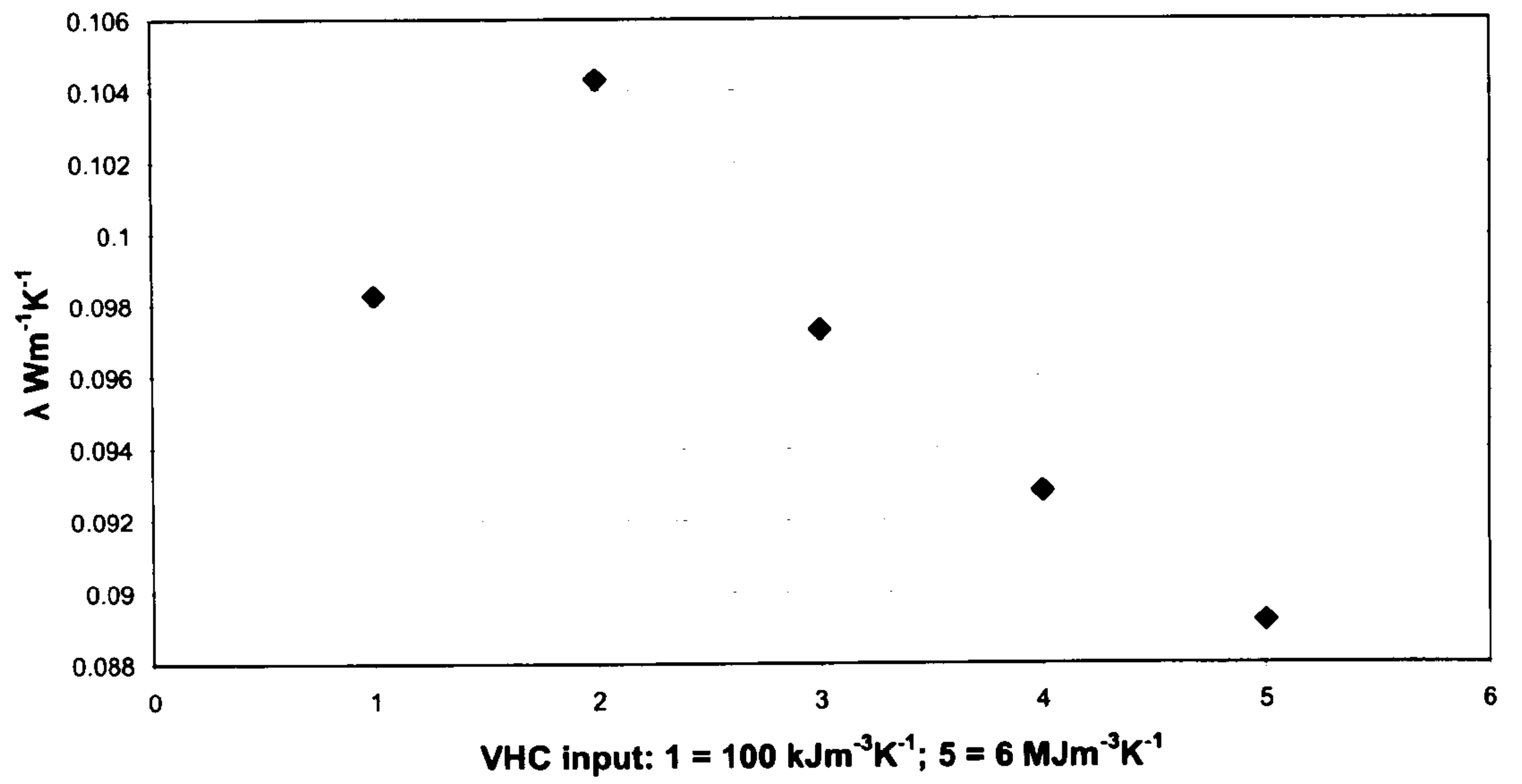
Chart 55: Voltra thermal conductivity outcomes for 0.1 Wm -1 K -1 input, varied pC
