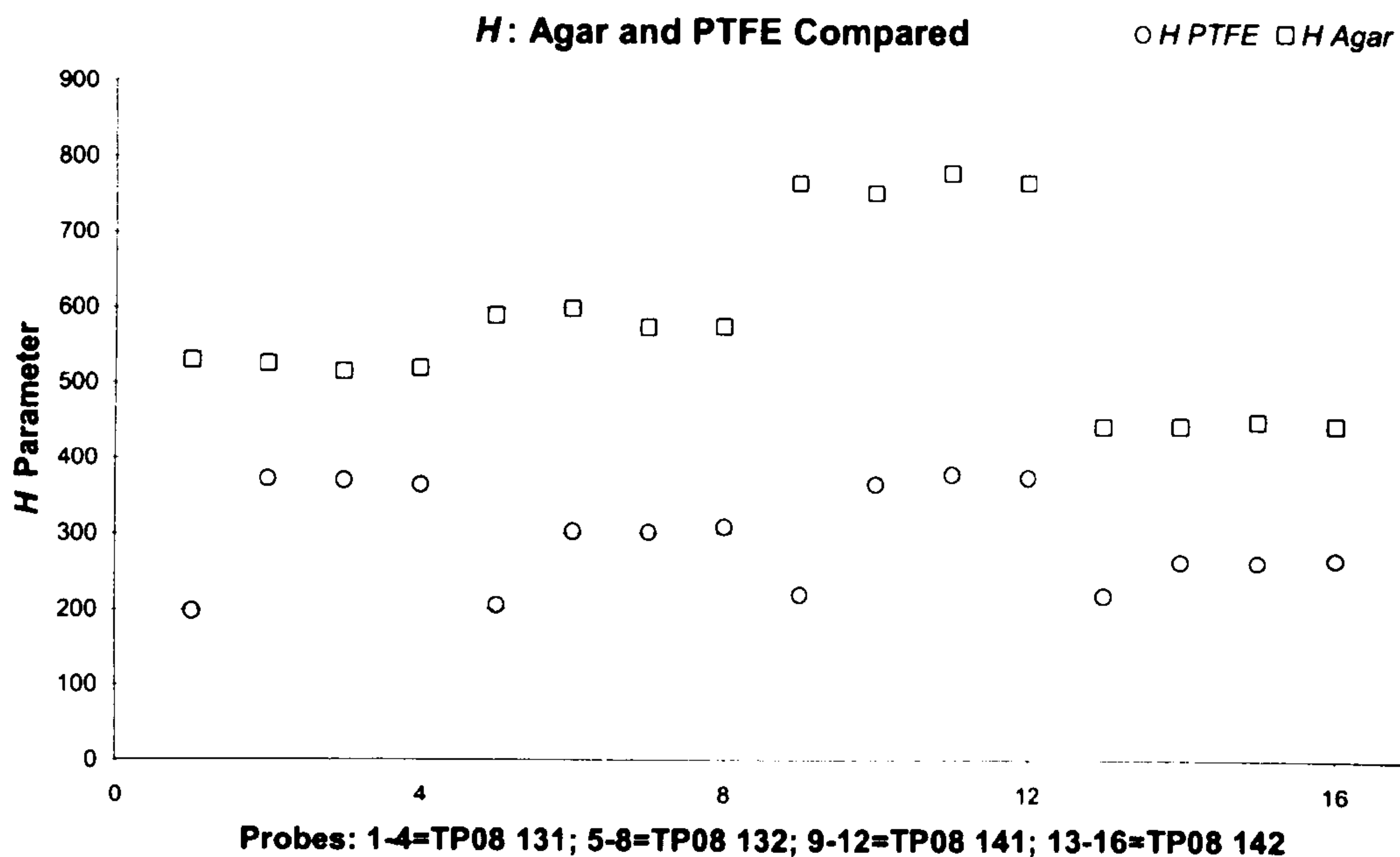
Chart 4: H values for TP08 probes in agar and PTFE
