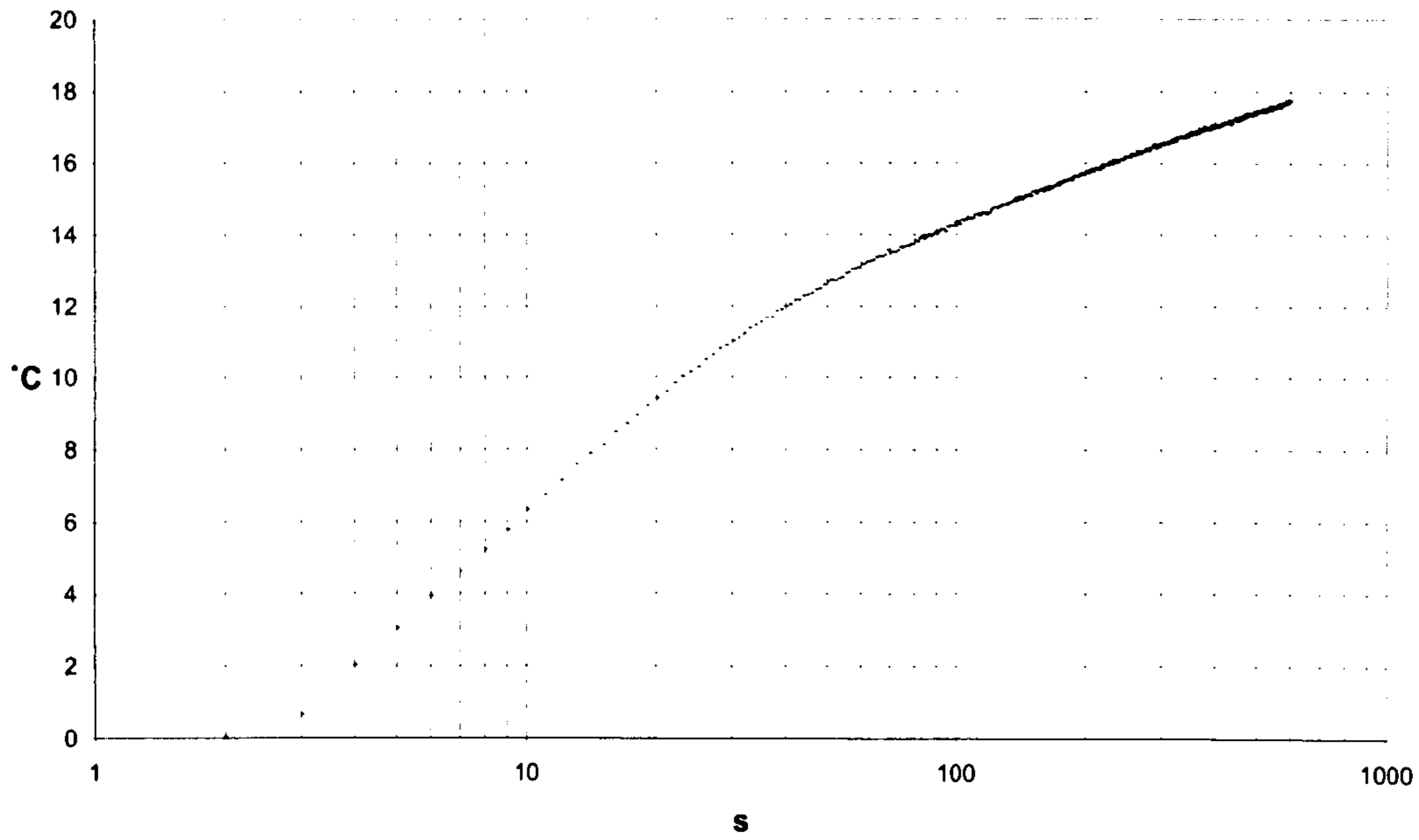
Probe Temperature v Elapsed Heating Time
