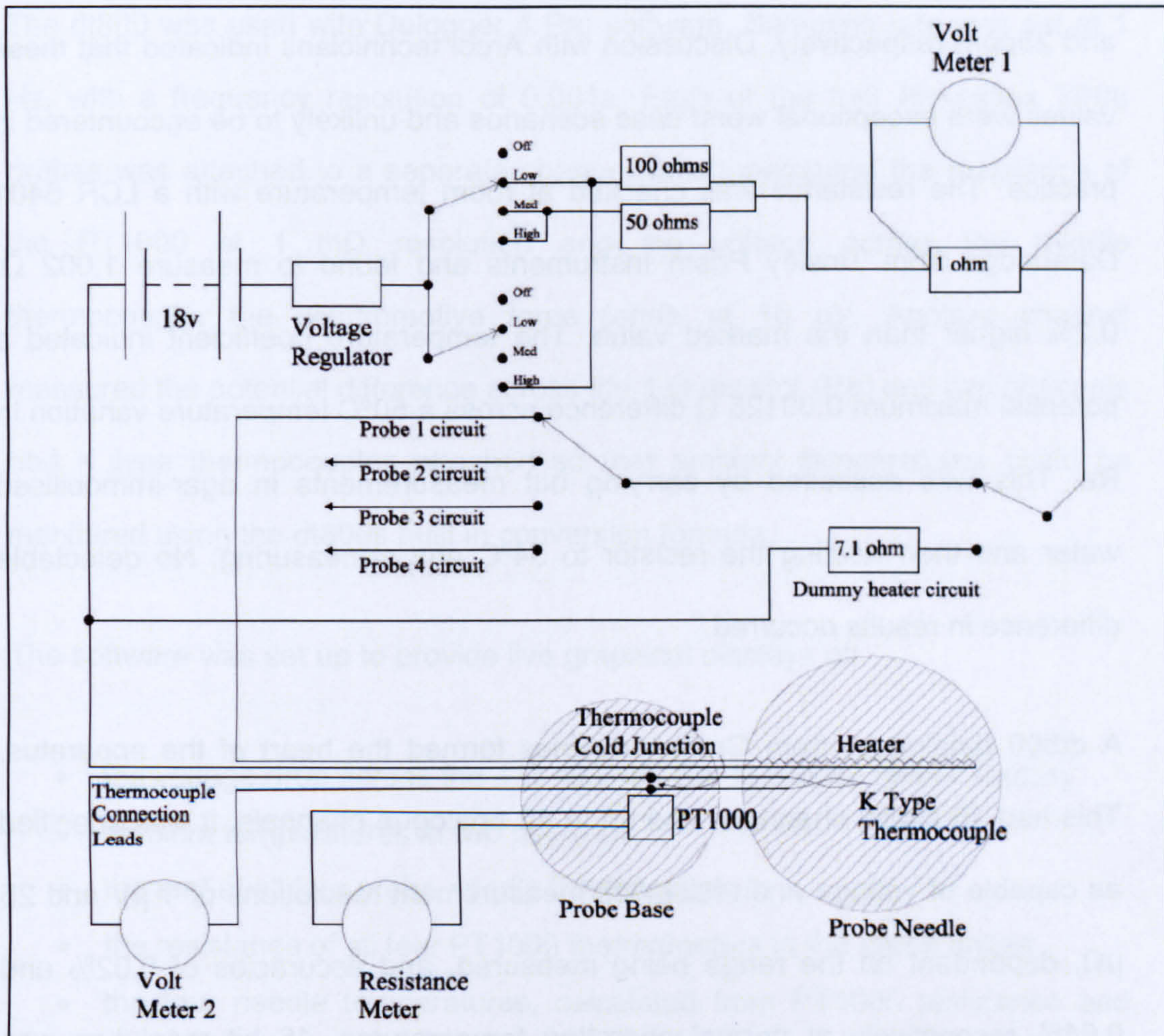
Figure 18: Field apparatus schematic
