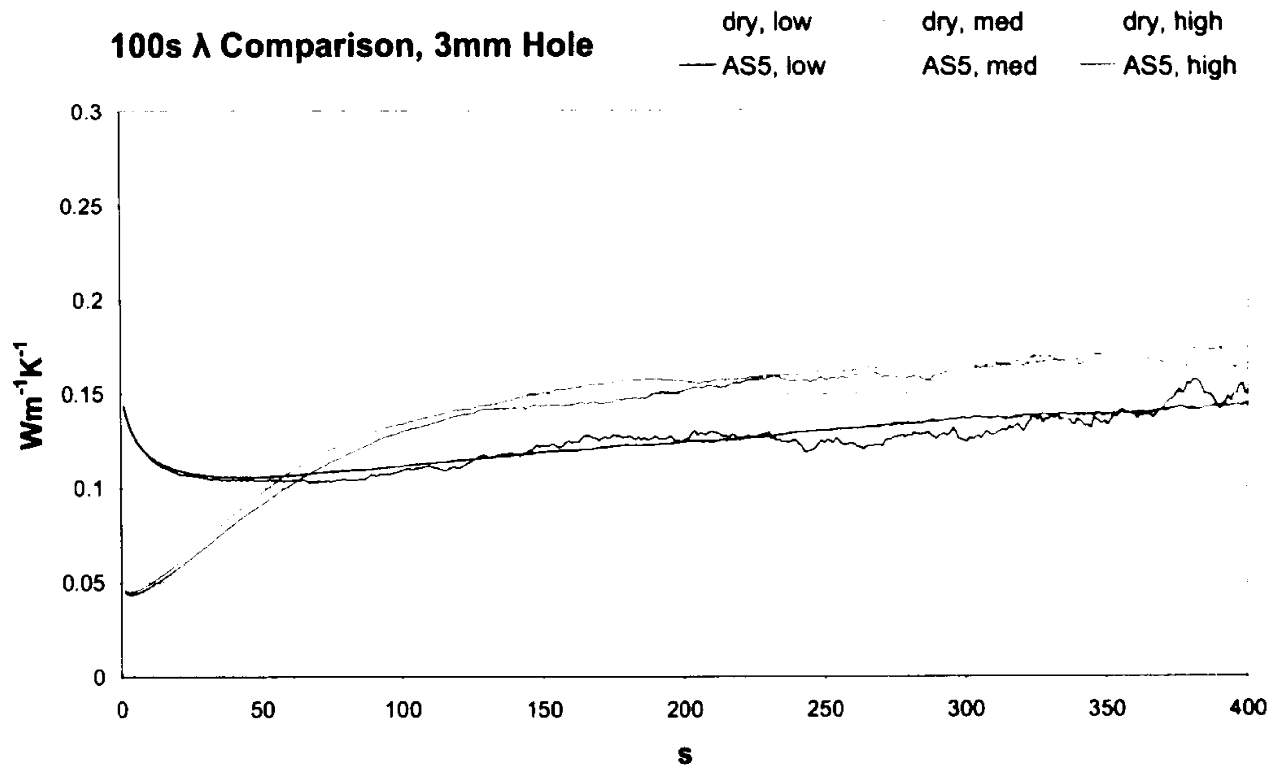
Chart 15: Thermal conductivity results from a 3mm hole, aerated concrete
