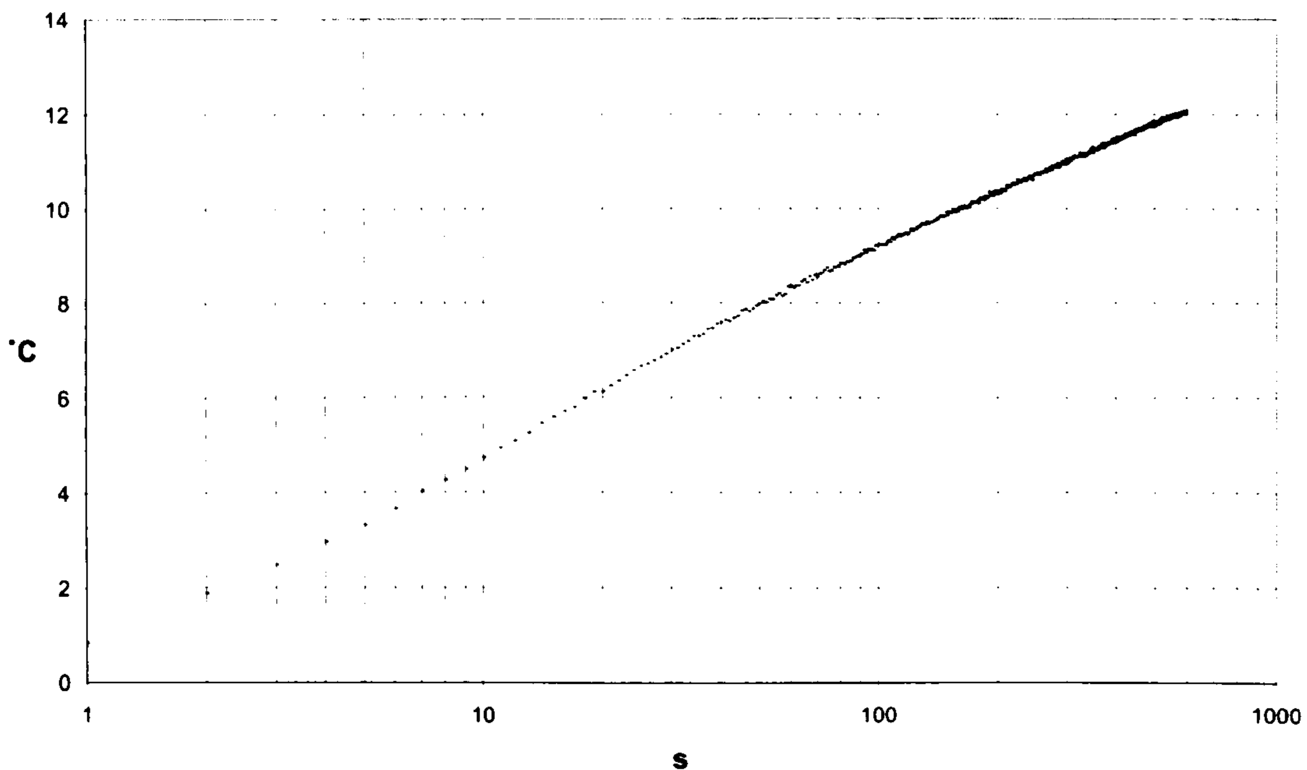
Chart 23: \Delta T/Int plot for a measurement in oak along the grain
