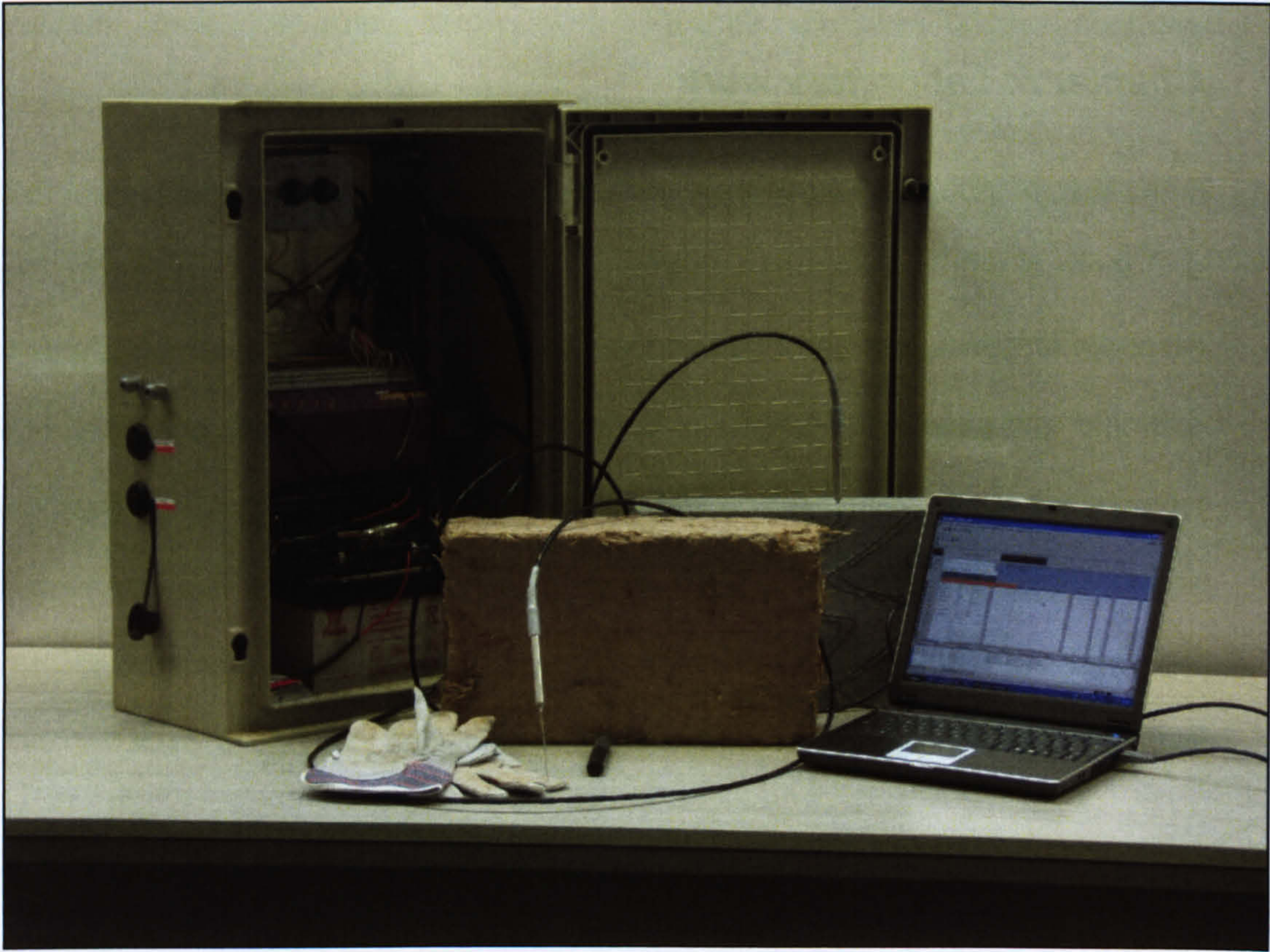
Figure 11: Laboratory based thermal probe apparatus
