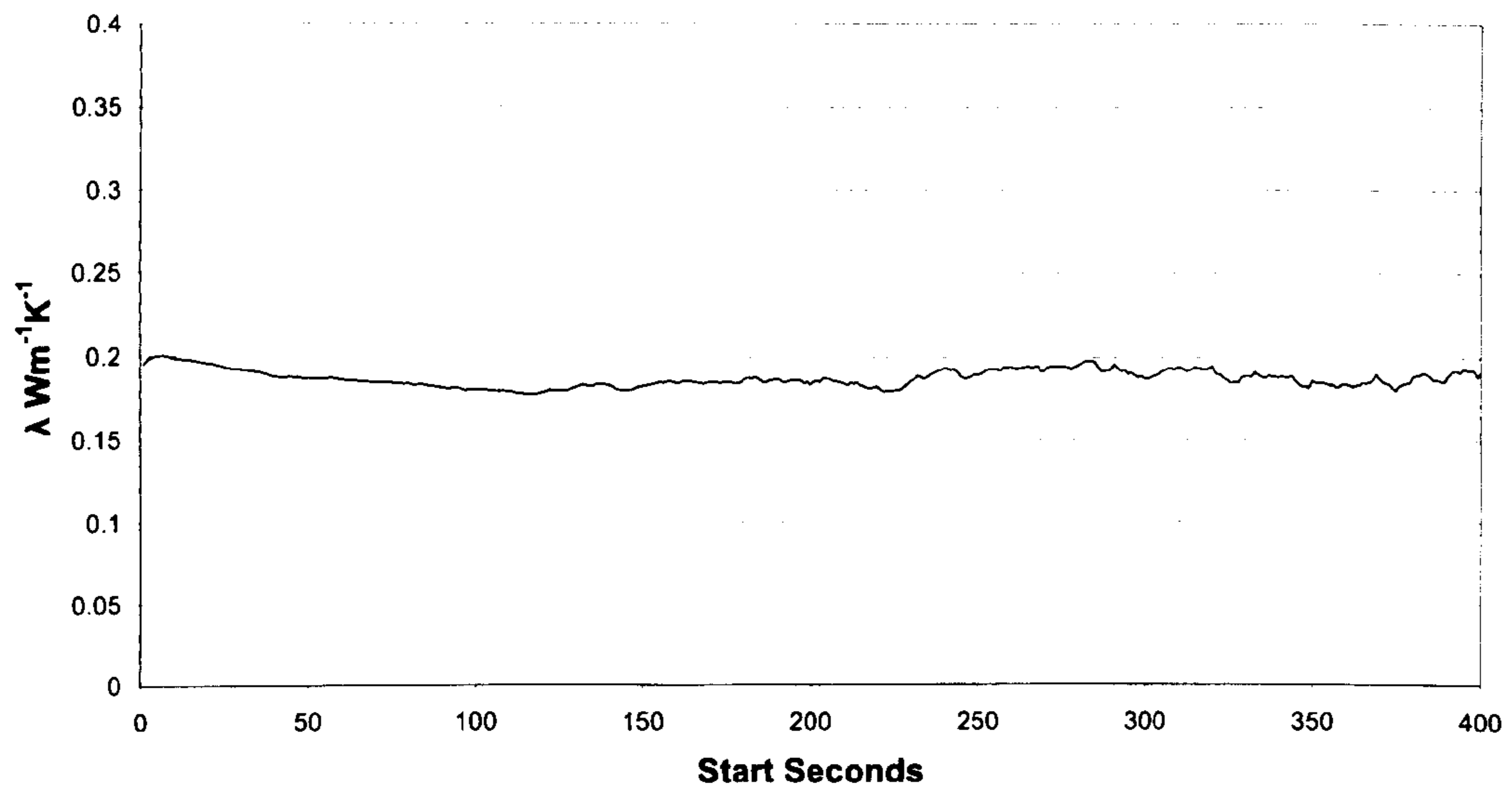
\lambda Calculated over 100s Periods
