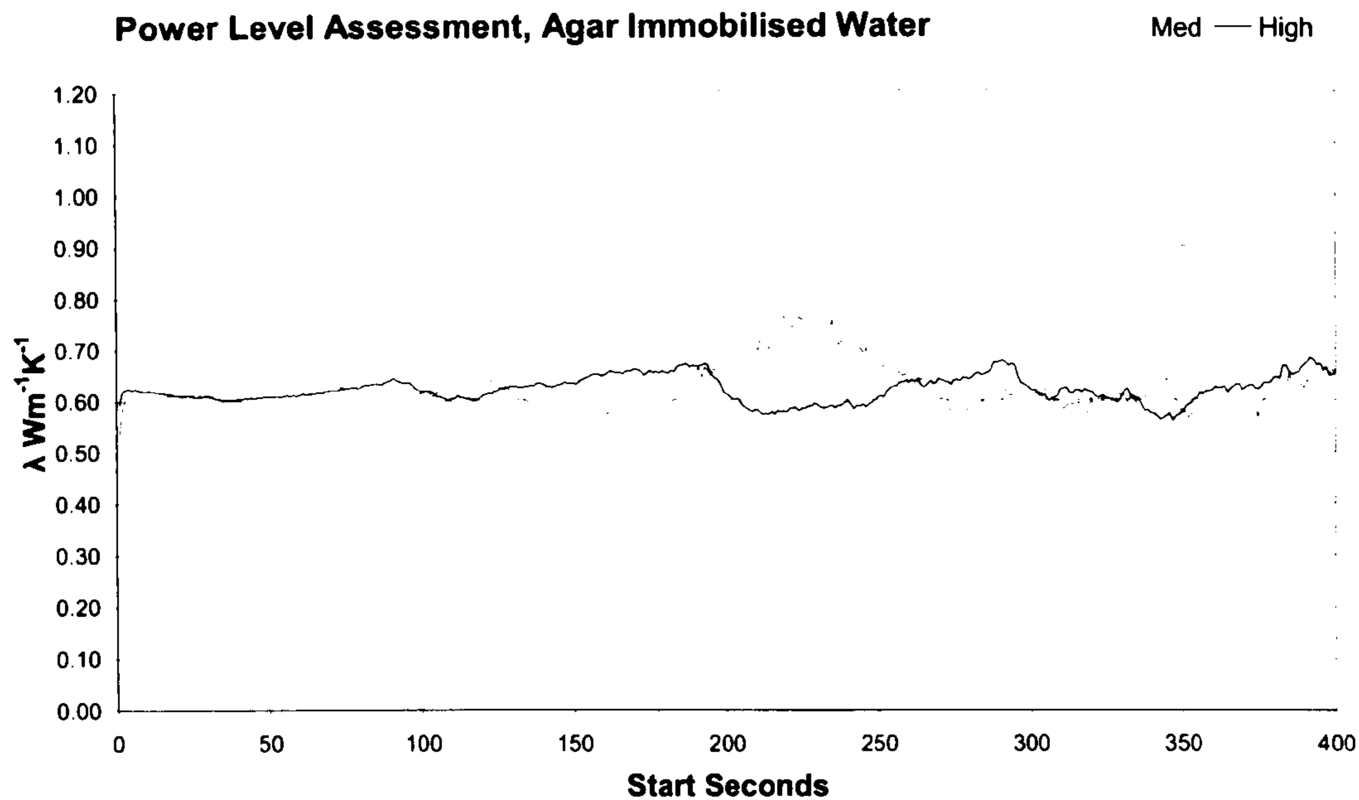
Chart 30: Thermal conductivity results for agar at two power levels
