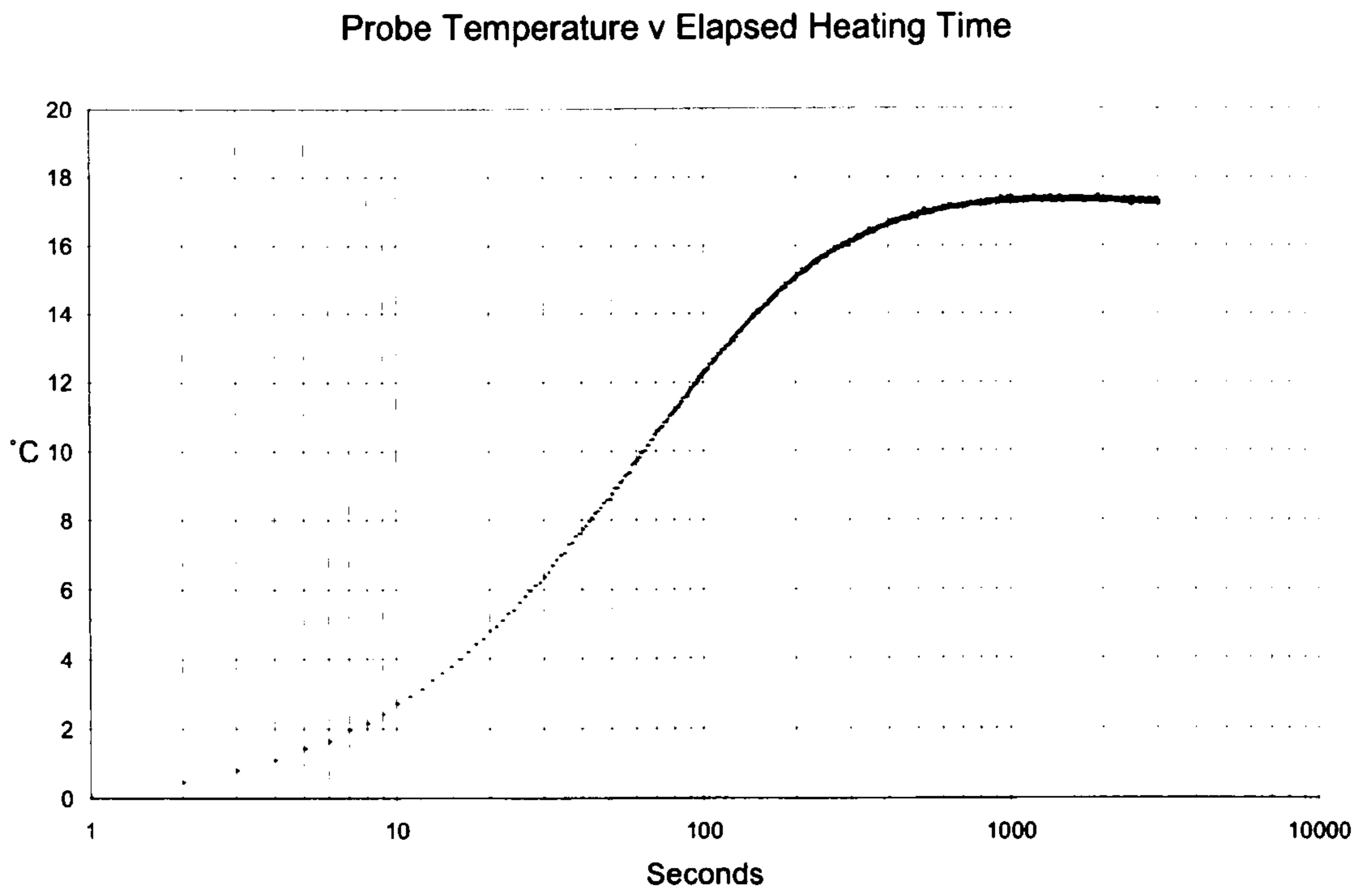
Chart 7: Typical S curve produced by a measurement in phenolic foam
