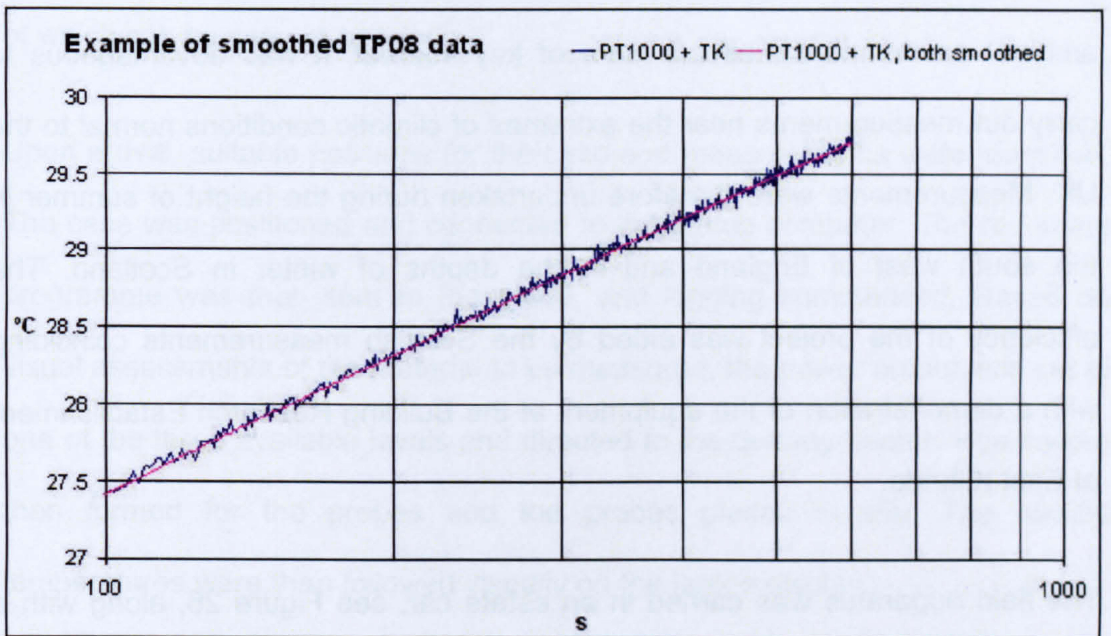
Chart 40: TP08 \Delta T/\ln t in petroleum jelly, with Lowess smoothing
