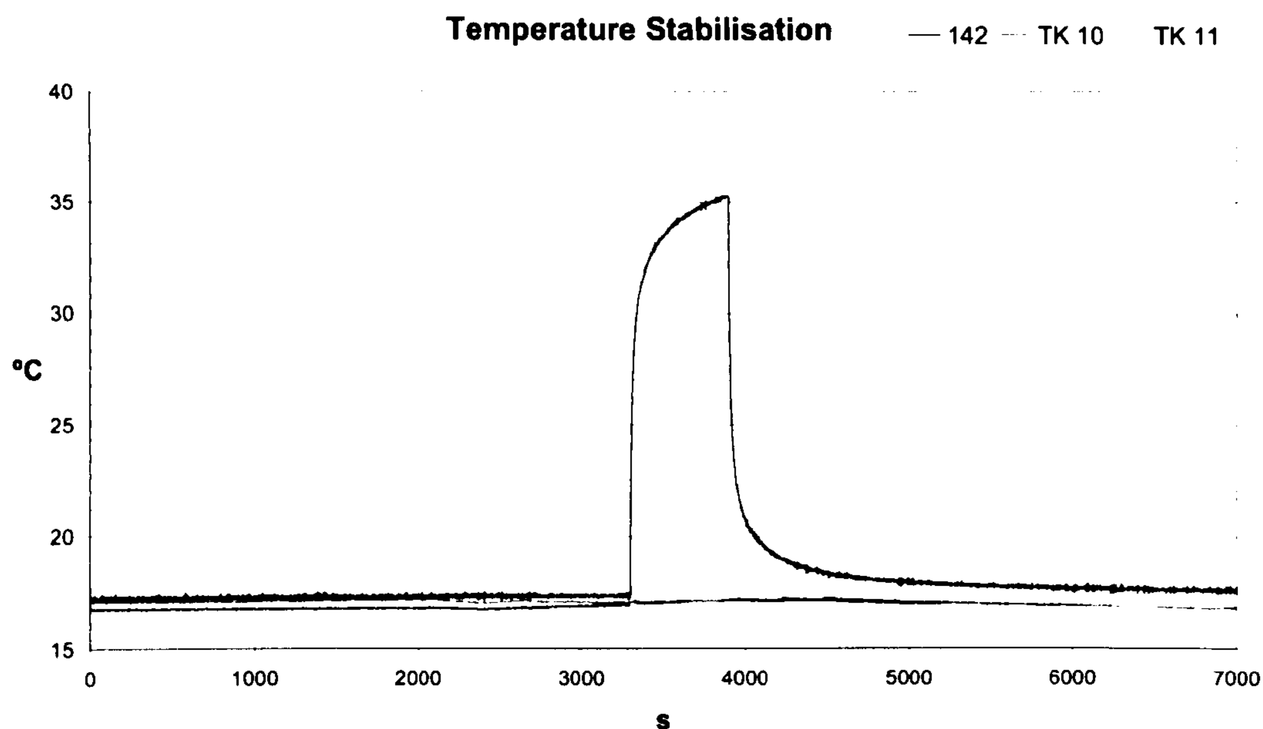
Chart 20: Temperature stabilisation following a heating cycle
