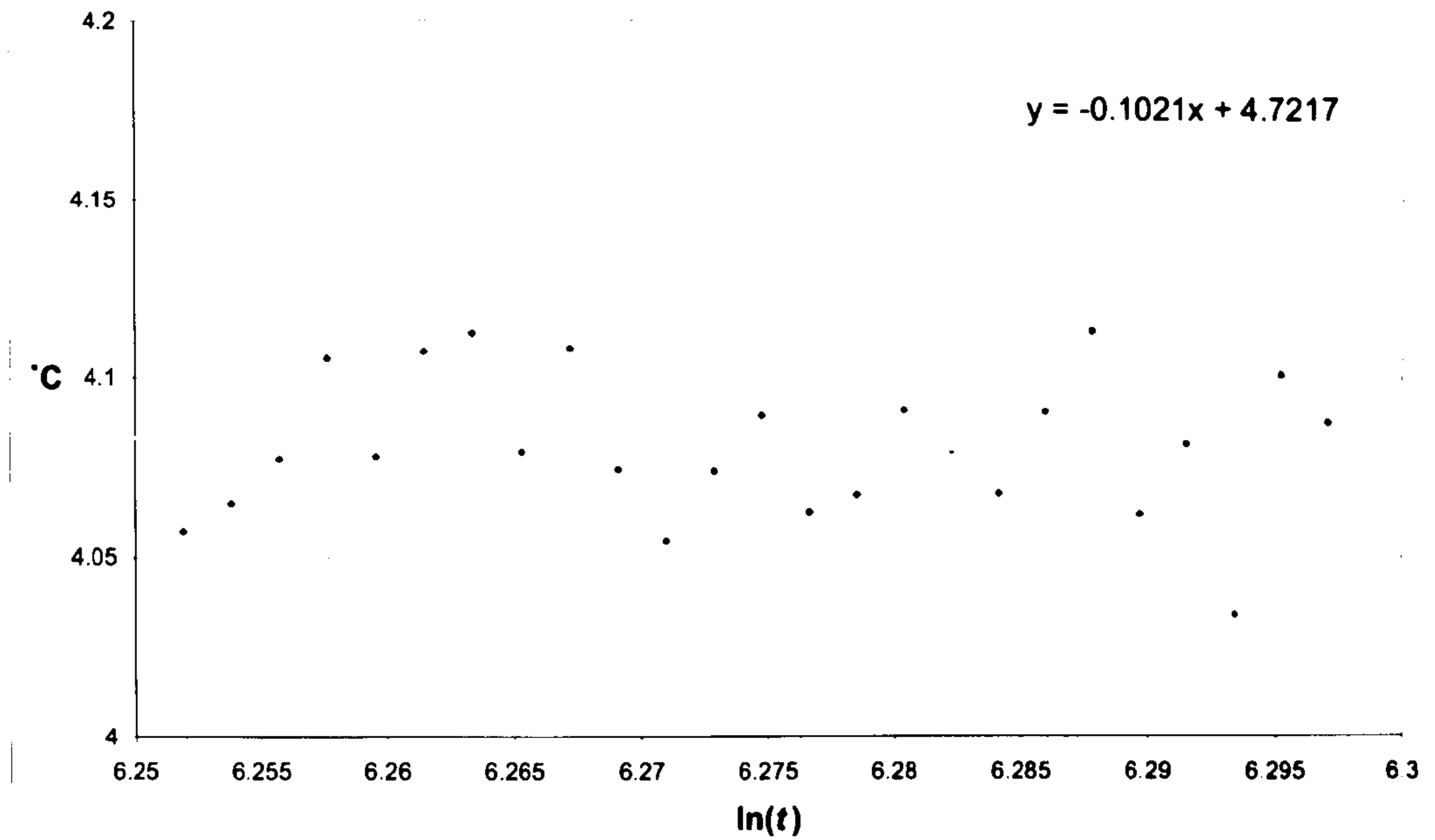
Chart 29: \Delta T/\ln t for later part of a measurement in agar immobilised water
