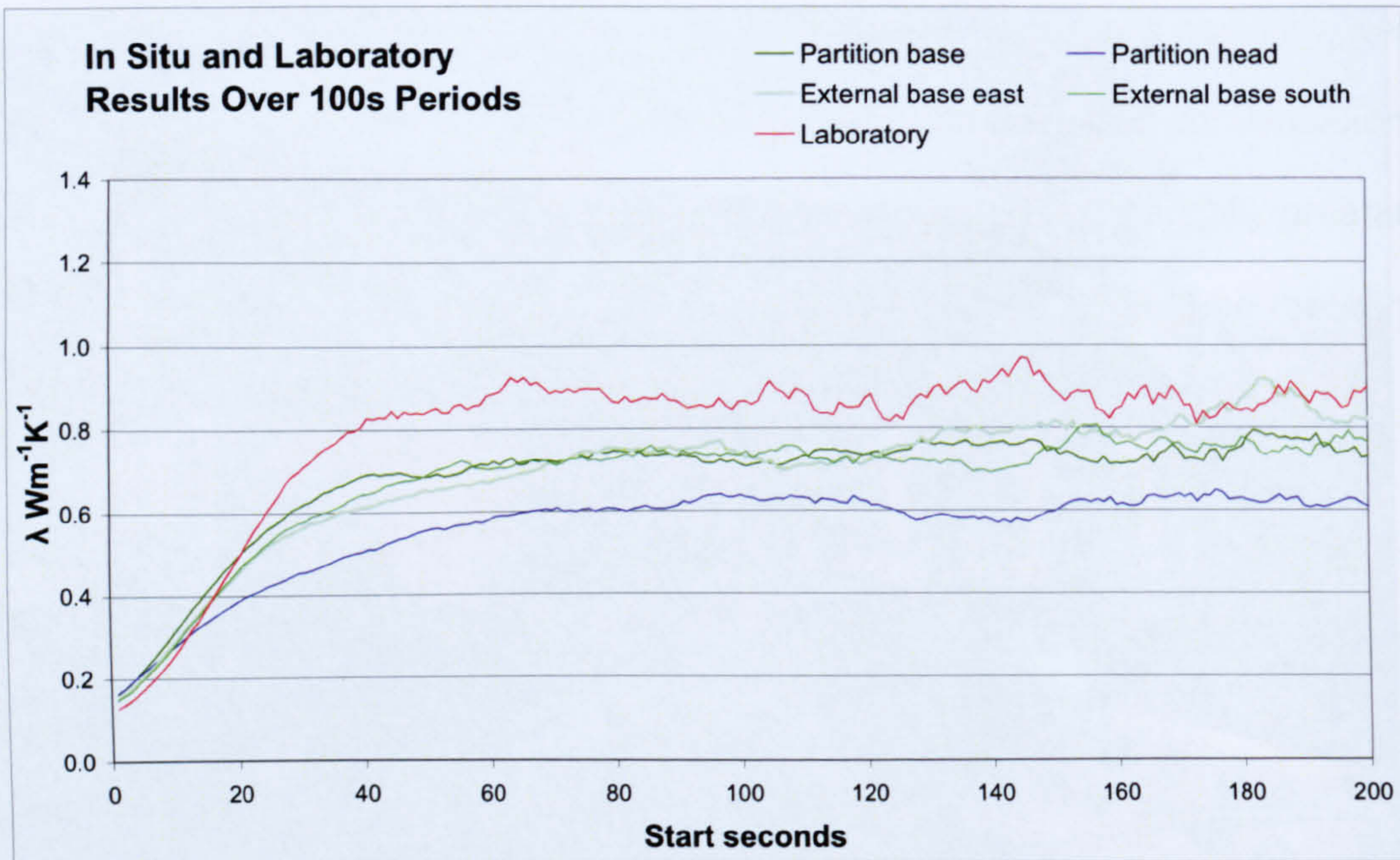
Chart 50: In situ and laboratory results for unfired earth and woodshaving bricks
