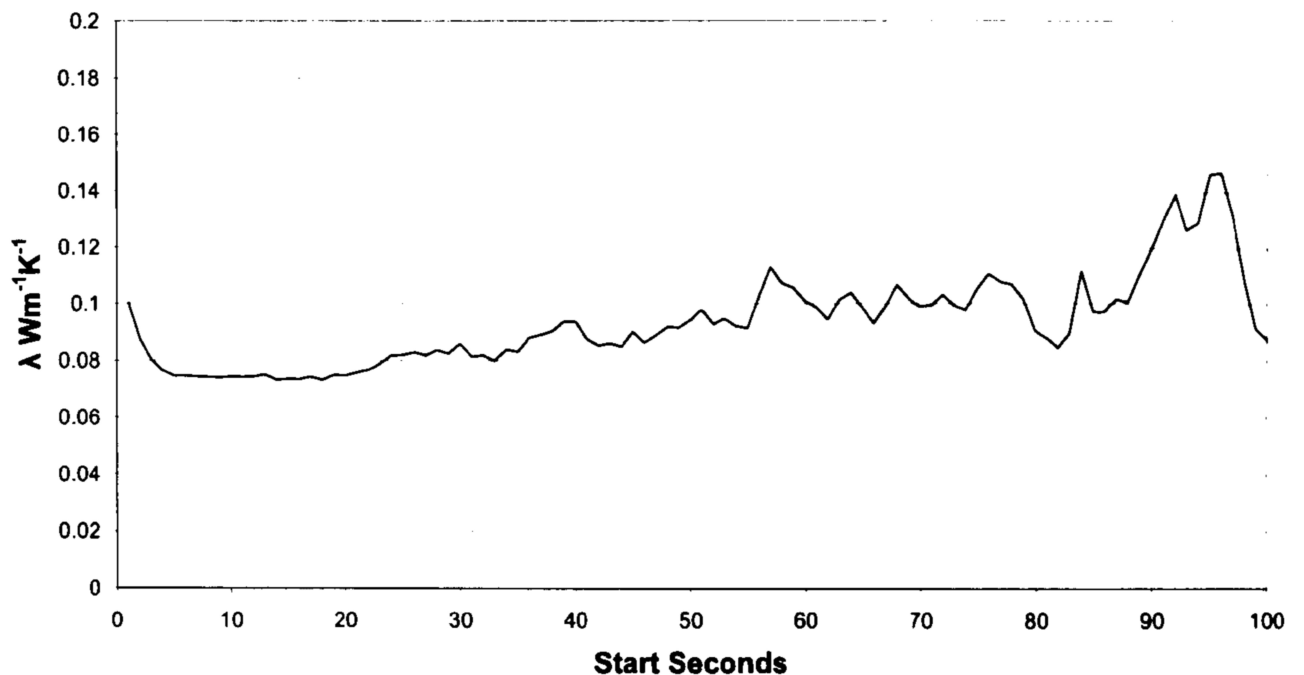
Chart 11: Hemcrete thermal conductivity, 10s time windows
