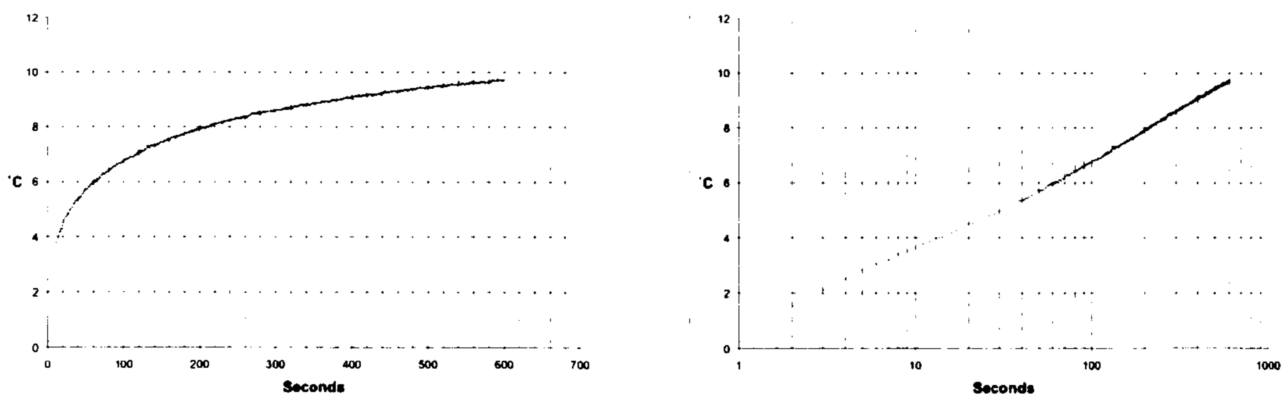
Figure 1: Example charts of temperature rise over time for aerated concrete
