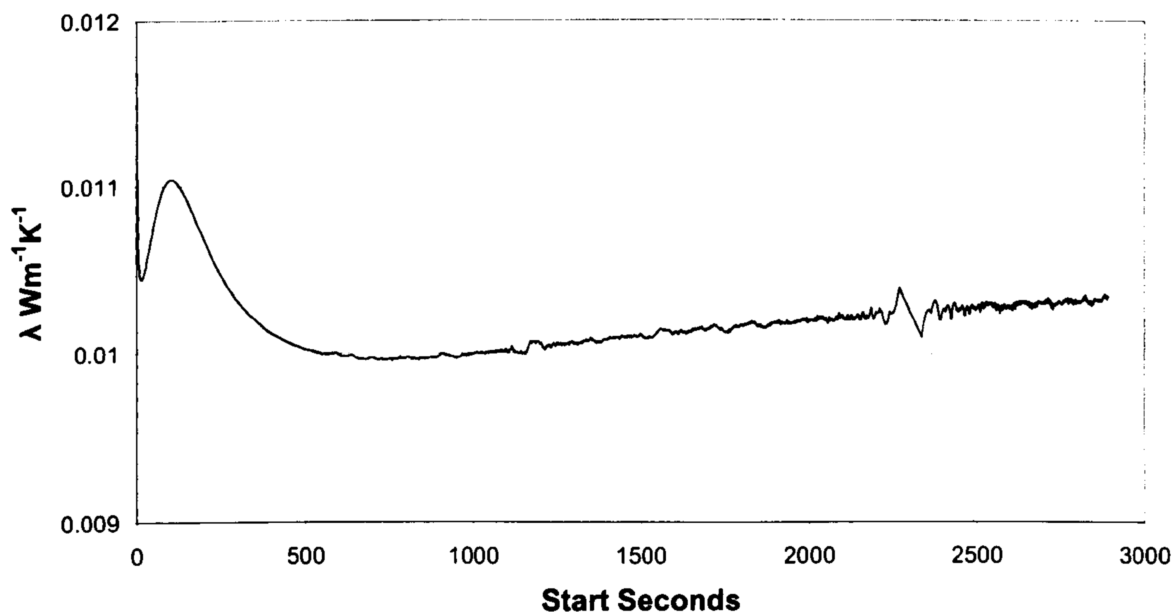
Chart 57: Voltra 100s results for 0.01 \text{ Wm}^{-1}\text{K}^{-1} , 100 \text{ kJm}^{-3}\text{K}^{-1}
