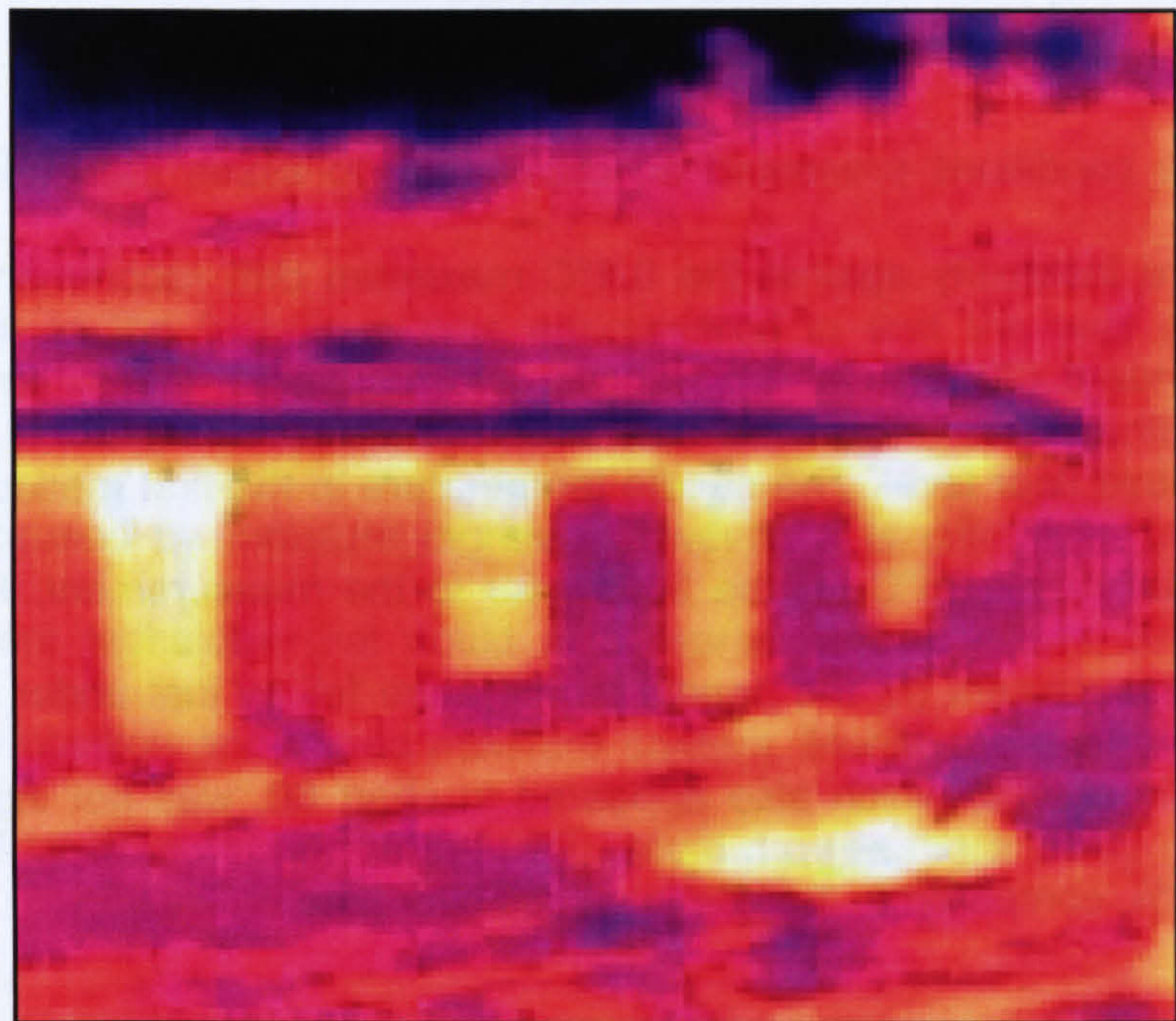
Figure 26: Thermal image of clay straw studio, ambient temperature -8°C
