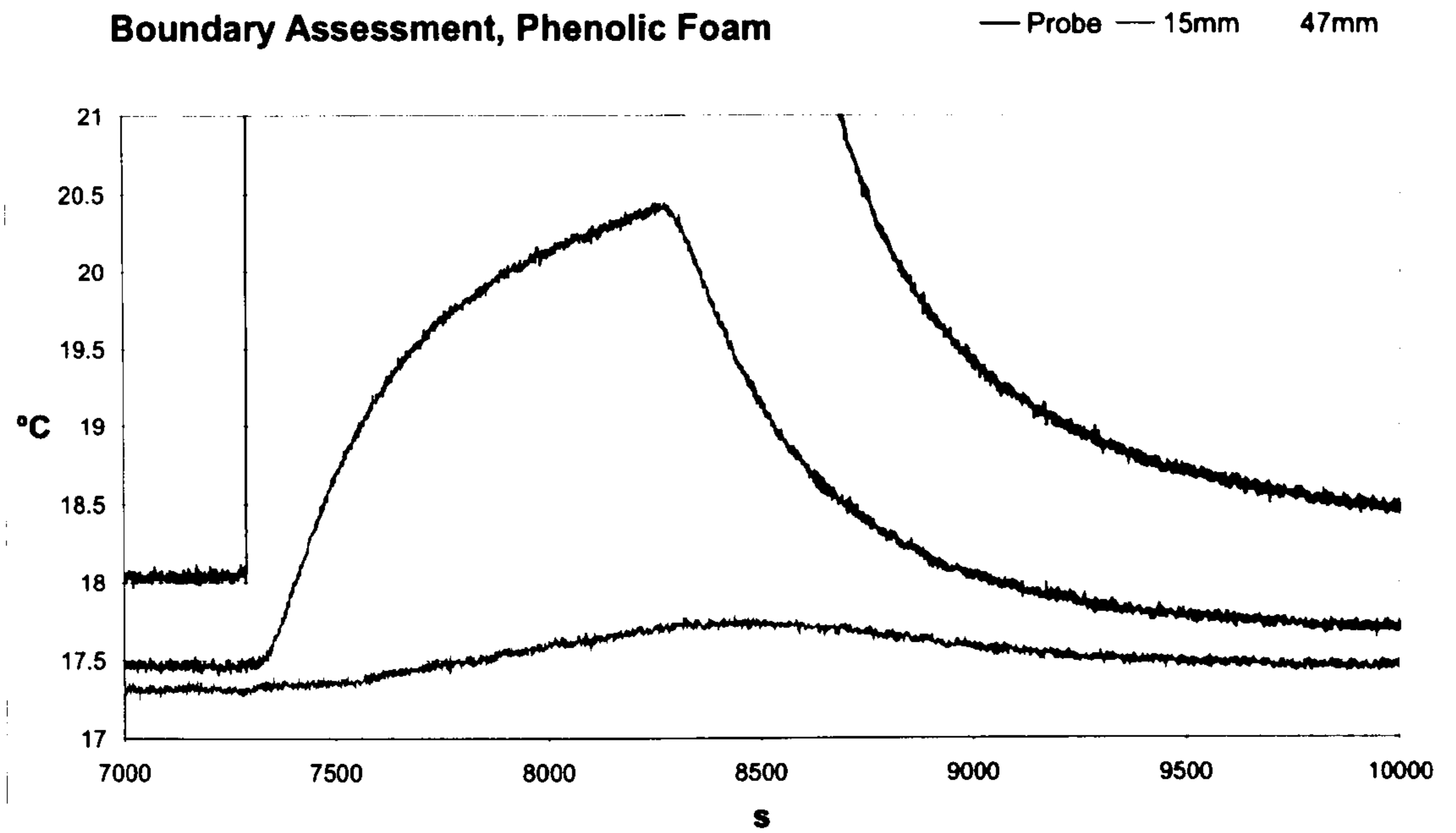
Chart 31: Temperature rise at 15mm and 47mm, phenolic foam
