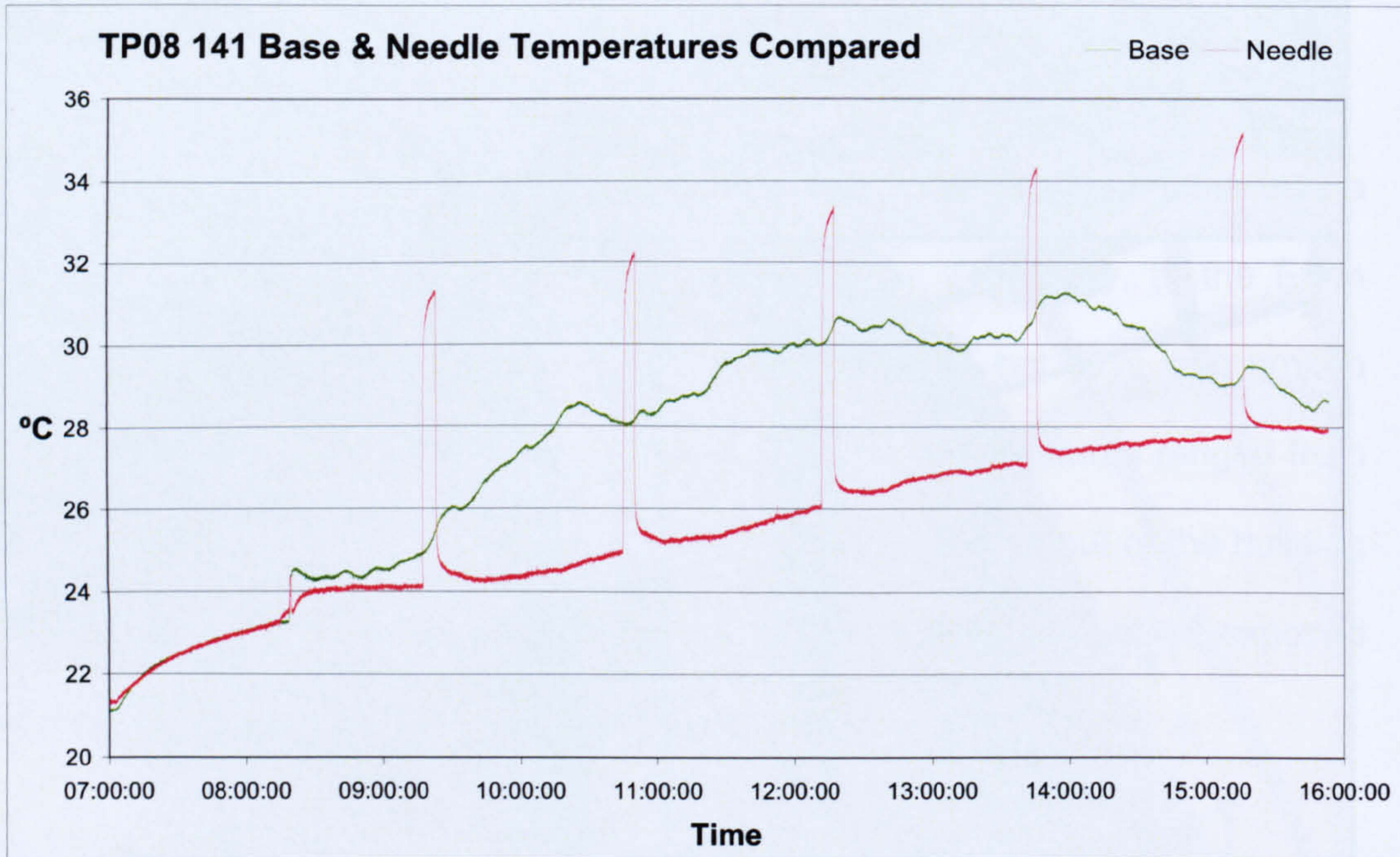
Chart 41: Temperature record of base and needle at internal wall head, the Body
