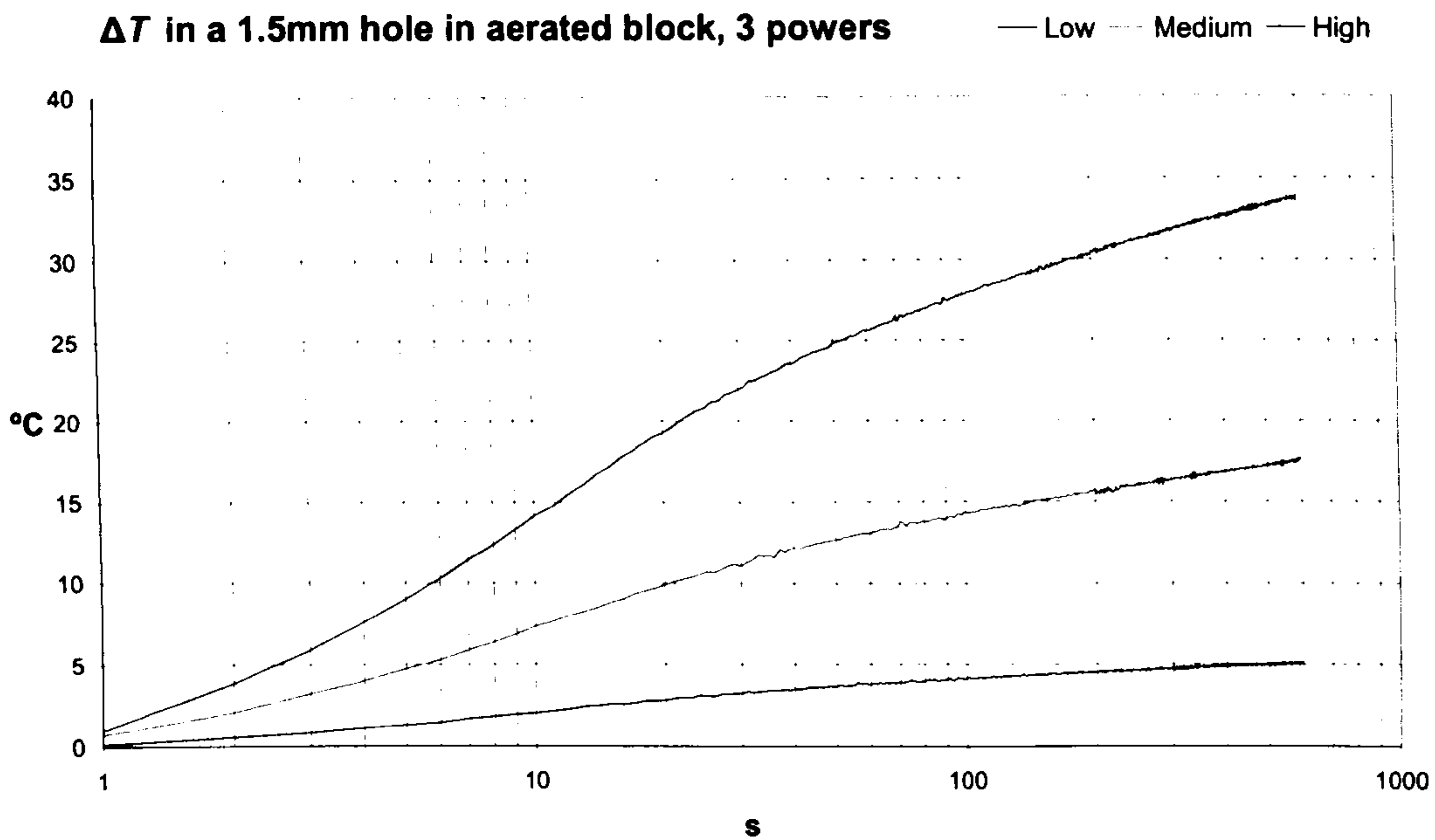
Chart 26: \Delta T/Int plots for measurements in aerated concrete at three power levels
