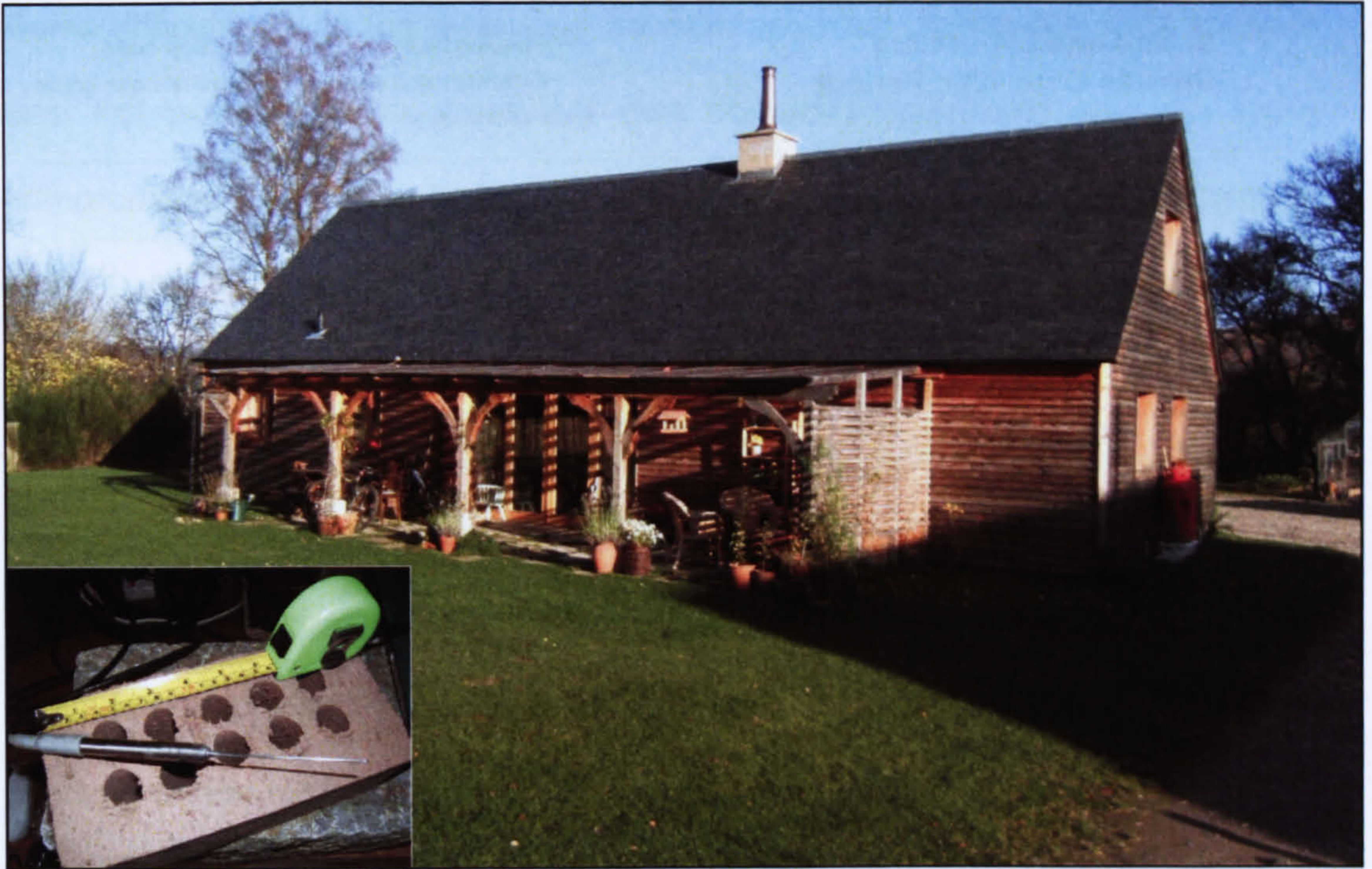
Figure 23: Unfired earth and woodshaving brick house with an example brick
