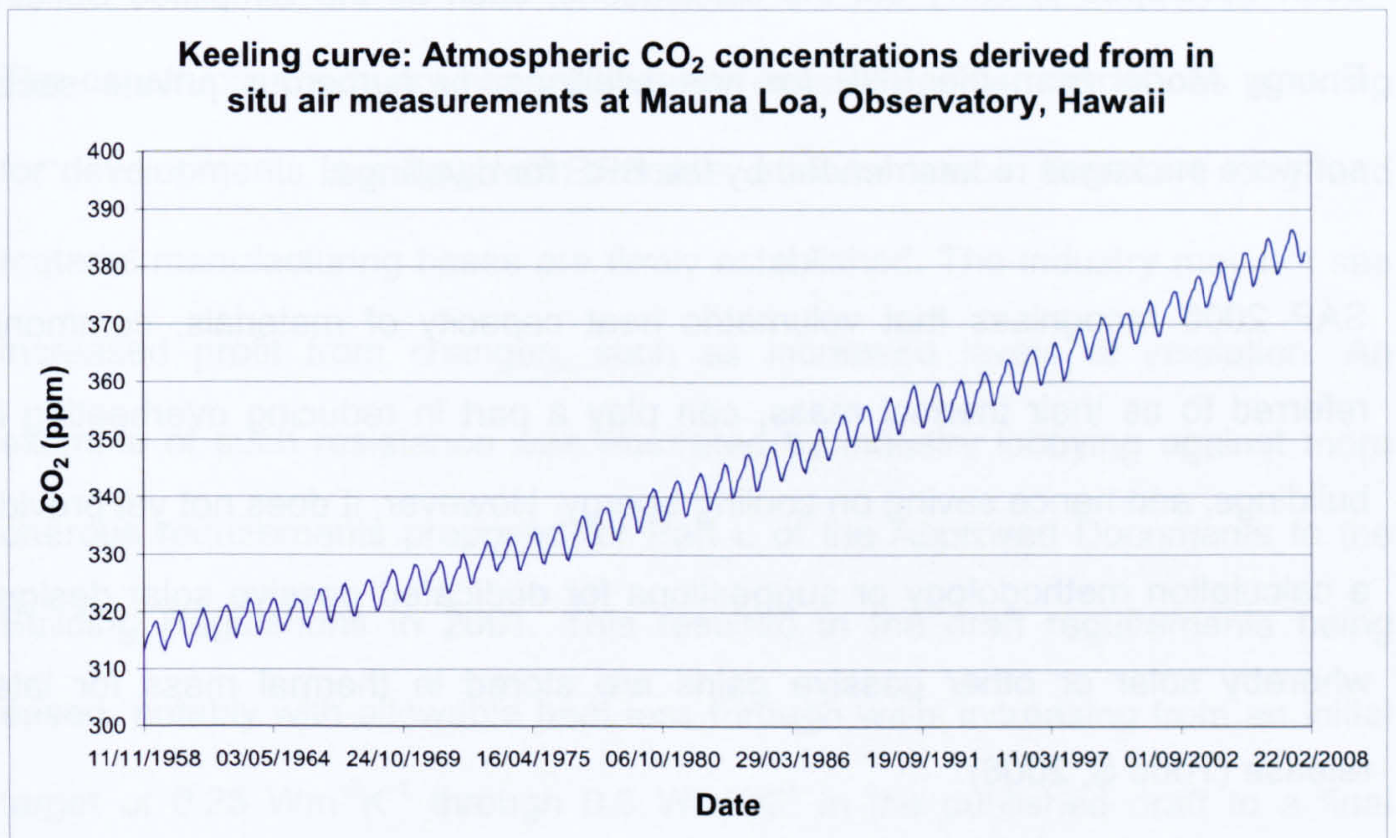
Figure 5: Keeling Curve of atmospheric carbon dioxide (Scripps, 2007)
