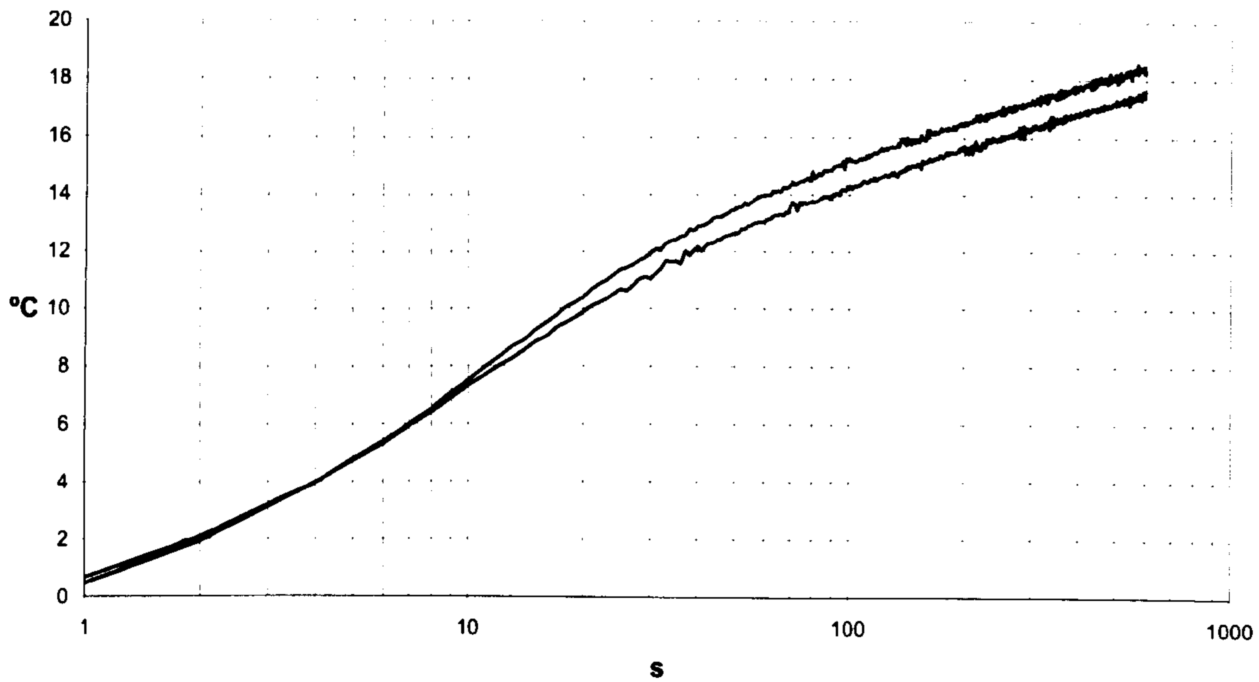
\Delta T in a 2mm hole in aerated block, with and without filler — Dry — ArcticSilver5
