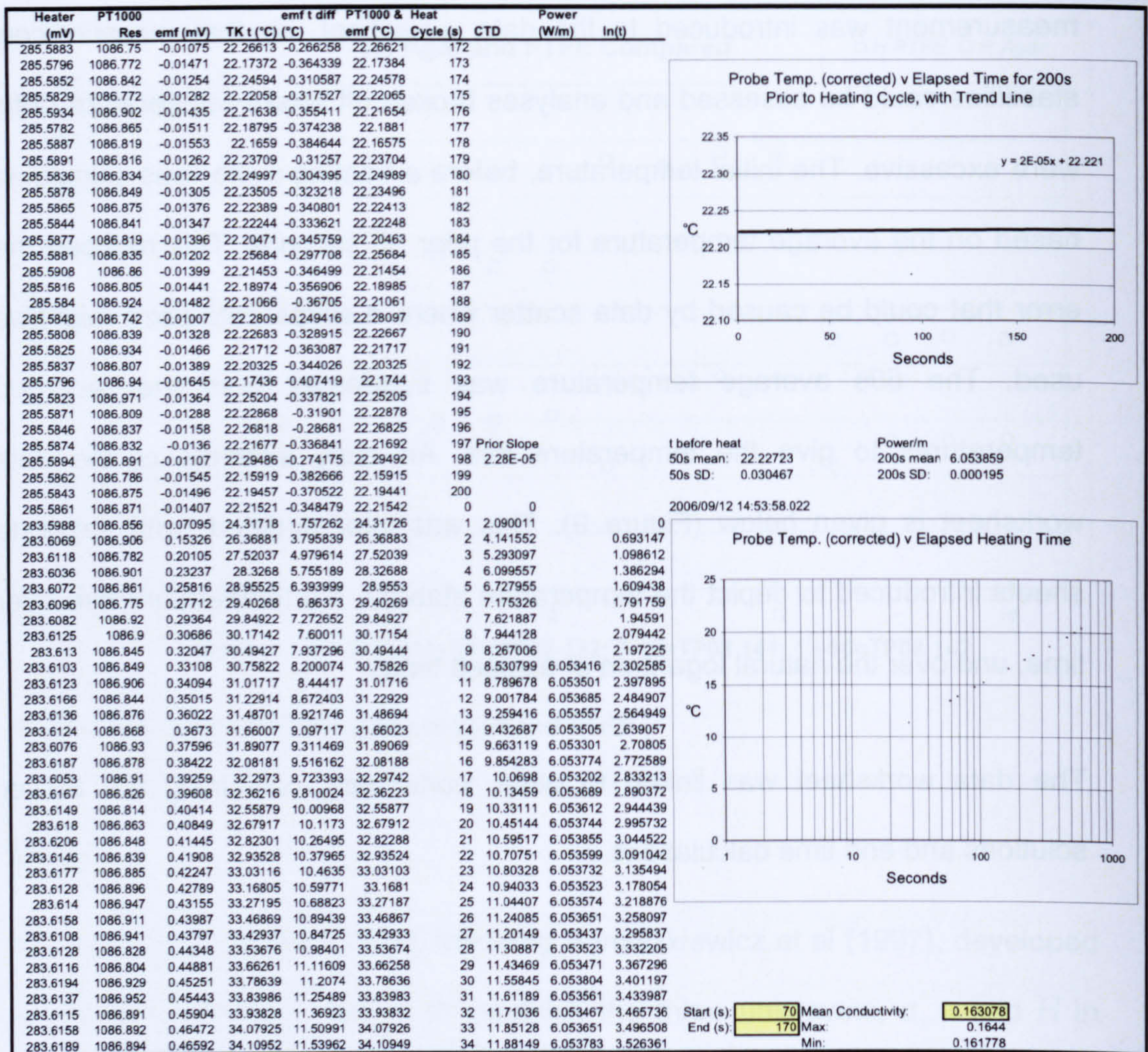
Figure 9: Example of a data sheet for a measurement in petroleum jelly
