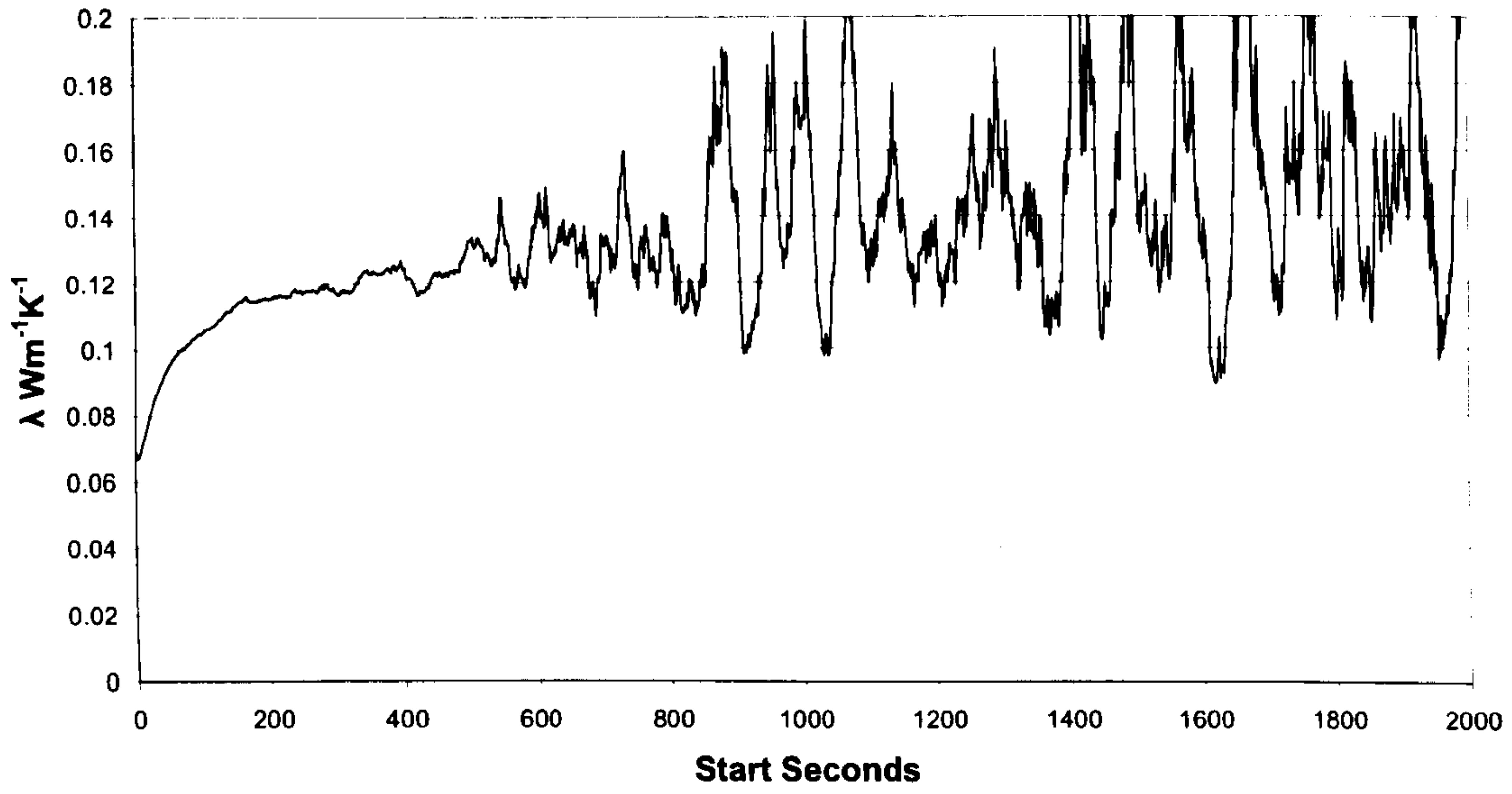
\lambda Calculated over 100s Periods - Hemp & Hydraulic lime
