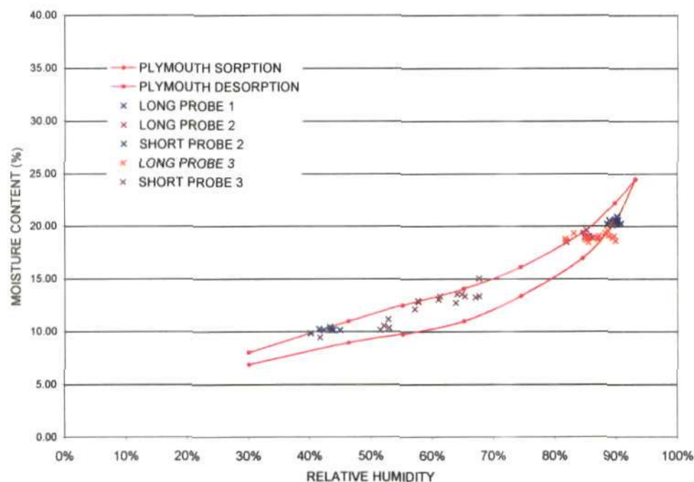
Fig.57 Results from wood block probes compared to Plymouth isotherms
