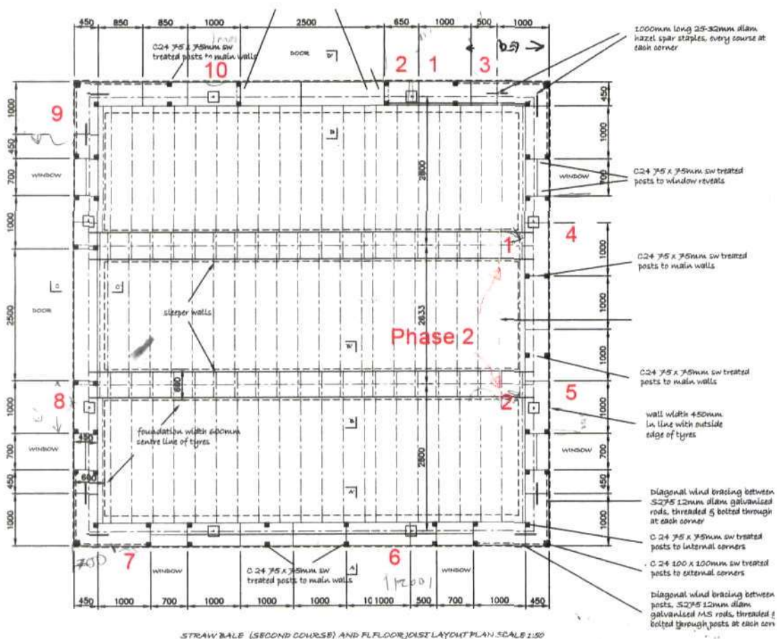
Fig.A40 Floor plan of Ocombe Farm
