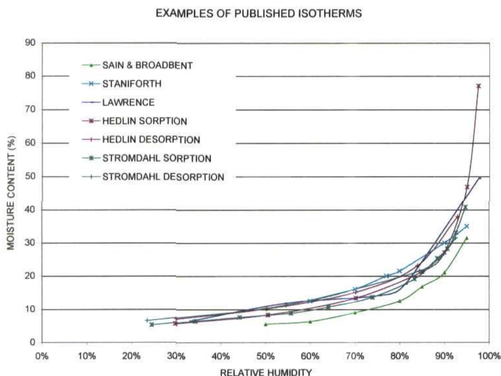
Fig.17 Published isotherms for straw
