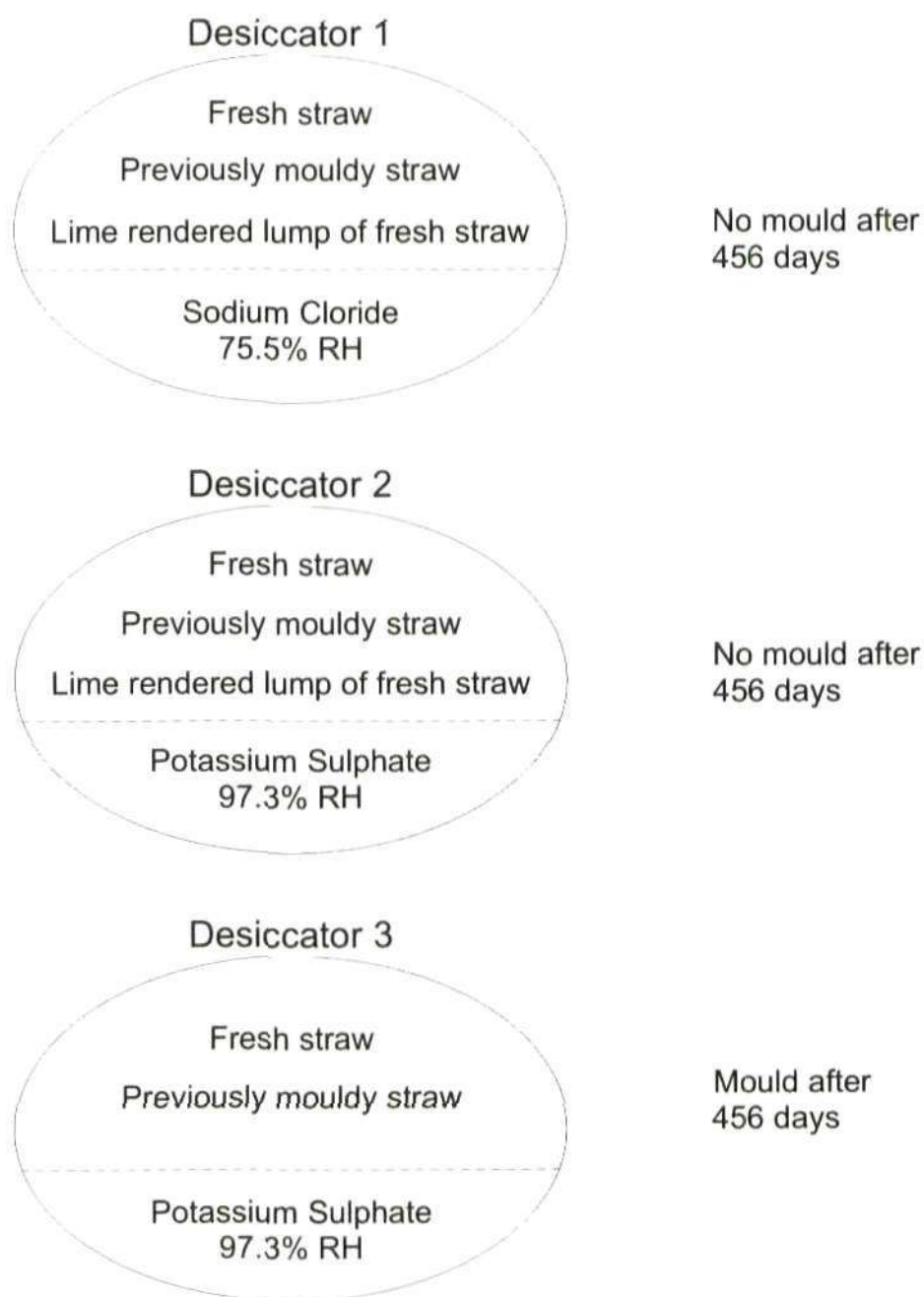
Fig.48 Diagram showing the contents of the three desiccators with their RH levels
