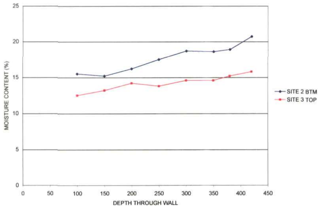
Fig.A32 Moisture profiles at Bristol studio
