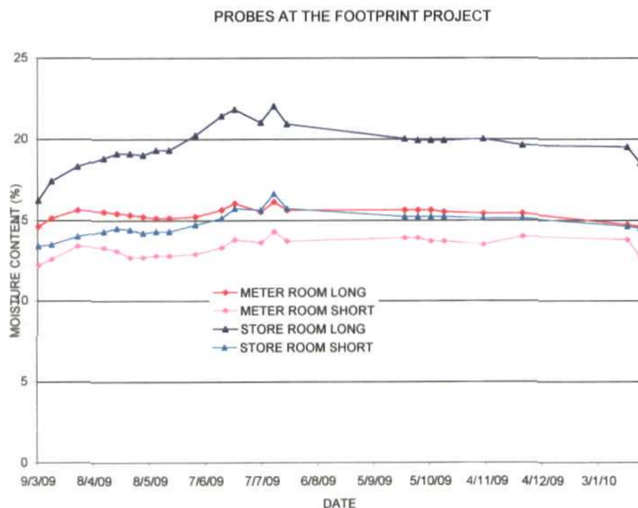
Fig.87 Readings from the new wood block probes installed at the Footprint Project
