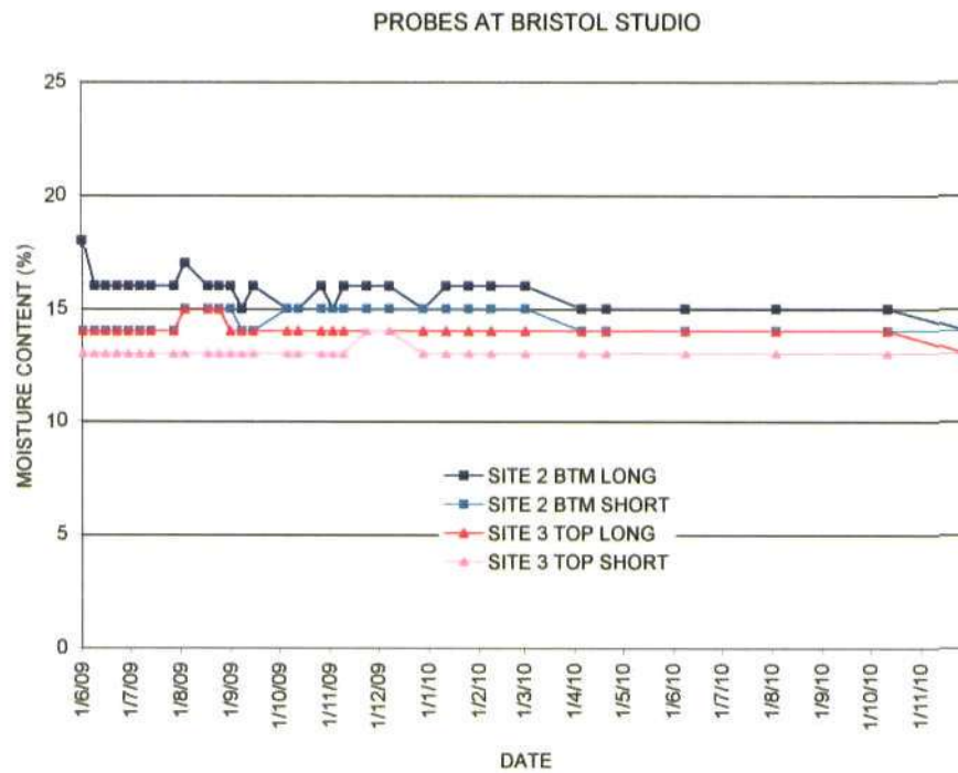
Fig.A33 Probe readings from Bristol studio
