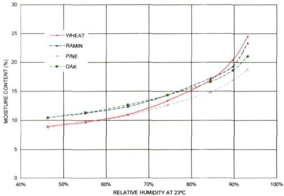
Fig.43 Section of sorption isotherms for three species of timber and wheat straw
