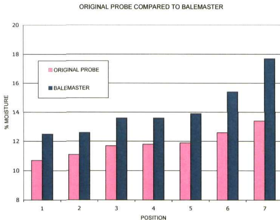
Fig.22 Comparing the original probes with the “Balemaster”
