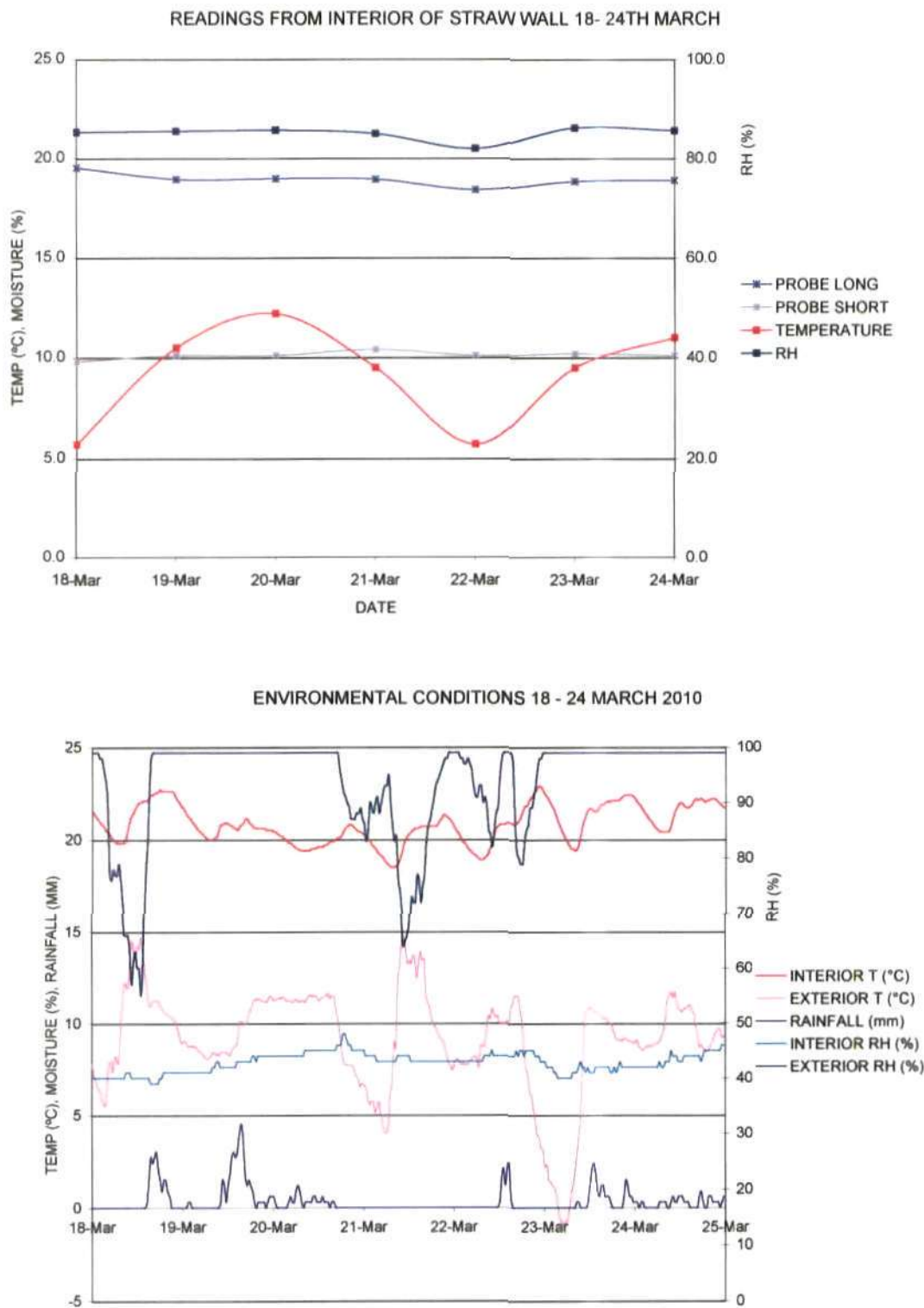
Fig.77 Moisture levels inside a wall compared to environmental conditions on the interior and exterior of the Totnes House recorded over a week
