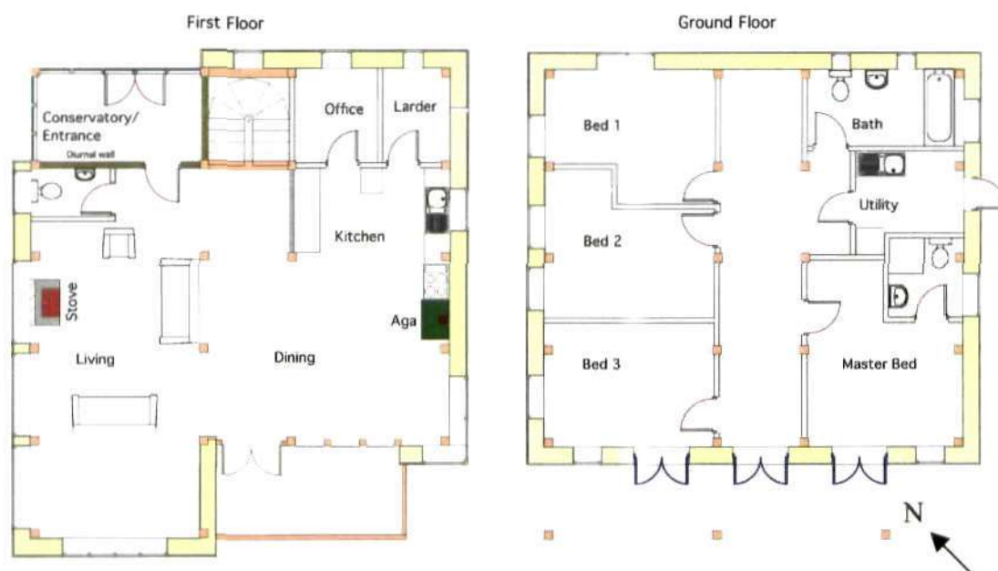
Fig.62 Floor plans of Totnes House
