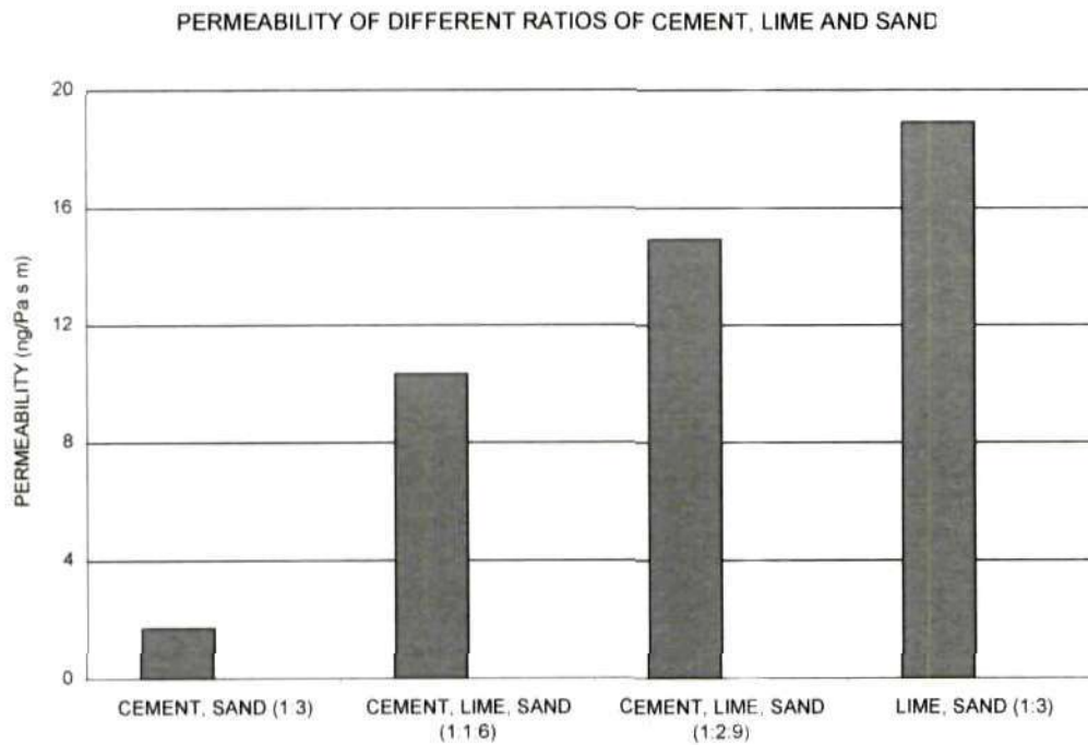
Fig.18 Graph showing the considerable difference in the permeability of renders using varied combinations and ratios of cement, slaked lime, and sand (Straube 2000a).
