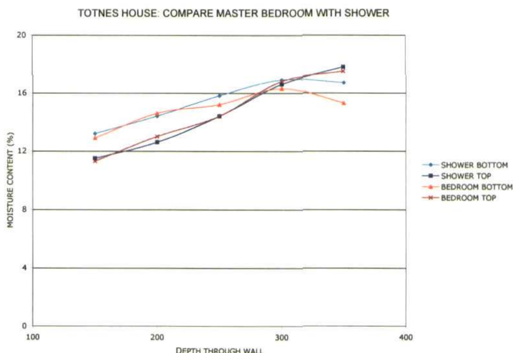
Fig.74 Comparing bedroom with adjacent shower room on the same day. 26 th Oct. 2007
