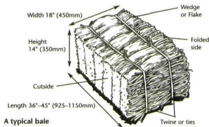
Fig.3 Illustration of a typical straw bale. Drawn by Julliet Breeze, from (Jones 2007)
