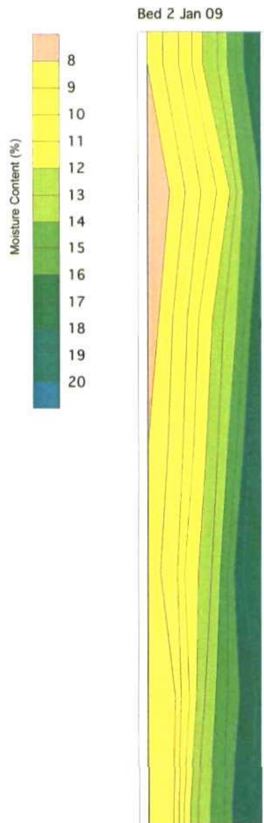
Fig.69 Moisture map of the wall of bedroom 2 (Interior of the house on the left)
