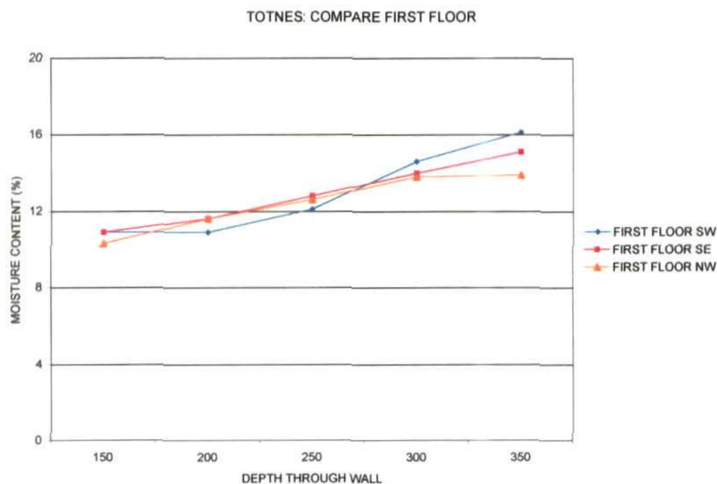
Fig.75 Readings from different walls of the first floor of the Totnes House 25 th Jan. 2010 The readings shown in Fig.75 above are were all taken from the bottom of the walls. Unlike the ground floor walls, an additional cedar rainscreen cladding protects all these walls
