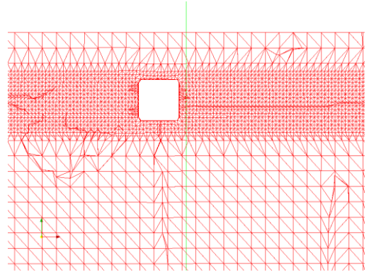
Fig. 27 Split-hexahedra mesh (vertical Section) around cylinder
