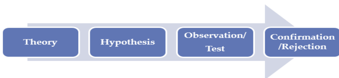
Figure 4.2: Deductive process
