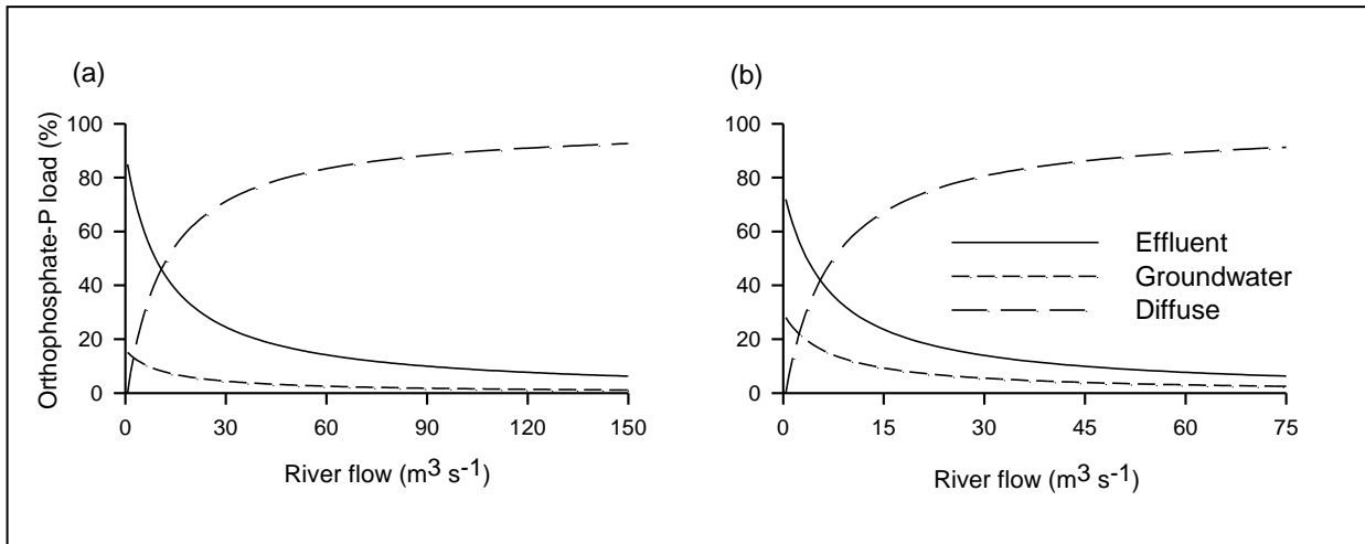
Figure 3. Calculated orthophosphate-P load from effluent, groundwater and diffuse run-off (%) vs river flow ( \text{m}^3 \text{s}^{-1} ) at (a) site 2 on the R. Taw and (b) site 14 on the R. Mole. Note changes in scales.
