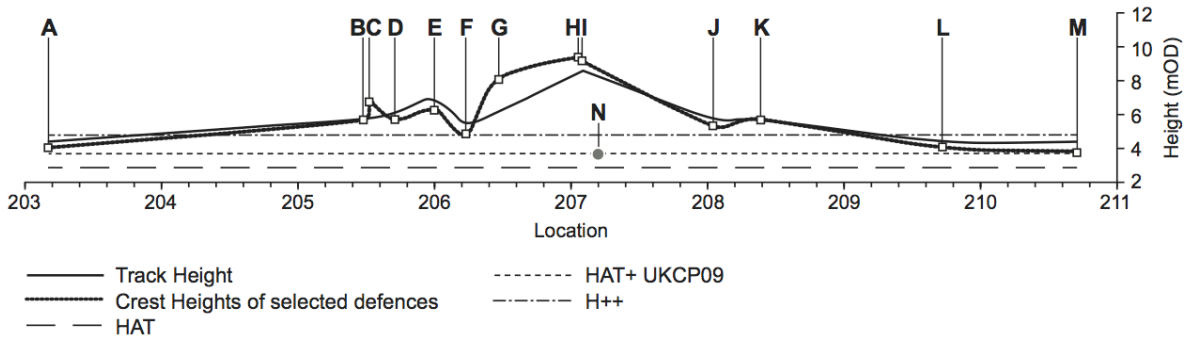
Figure 3. Elevation profile (in metres relative to Ordnance Datum) of the Dawlish-Teignmouth section of the London to Penzance railway line (in chainage). Locations (A-M) correspond with Figure 2. Crest heights have been compared with the current highest astronomical tide (HAT) and the UK Climate Impact Programme’s sea-level estimates (high & H++) for 2100 (Lowe et al., 2009).
