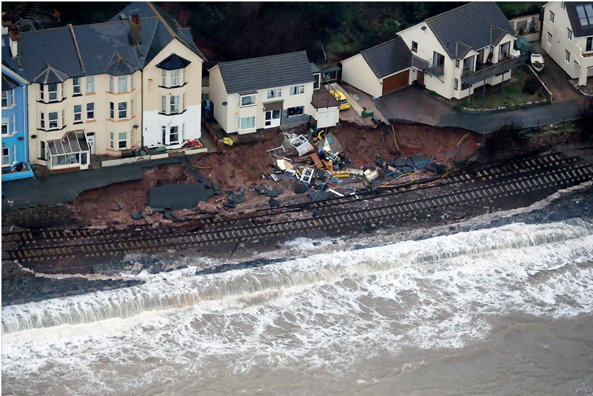
Figure 1: The breach in the sea wall near King Harry's Walk at Dawlish, Devon, on 7 February 2014 (see Figure 2 for map). The damage was caused by gales and high seas on 4 February and the railway track was left hanging over the breach. Source: Network Rail, 2014d.
