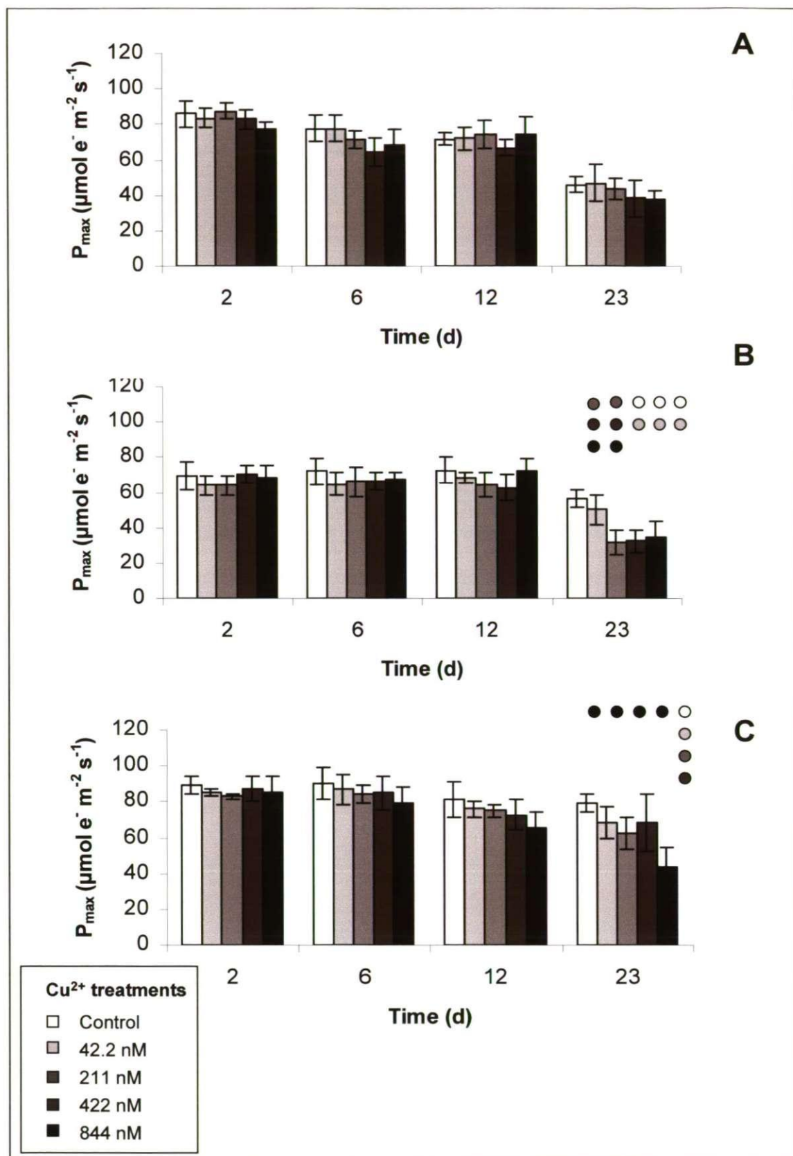
Figure 2.10. Effects of Cu 2+ on photosynthetic capacity P max calculated from chlorophyll fluorescence measurements of Bantham (A), Wembury (B), and Restrouquet fronds (C). Fronds were incubated for 23 days various concentrations of Cu 2+ . Significant differences (p<0.01) in the P max values between fronds in two treatments within the populations on the different days are indicated by their appropriate colour code. Values represents means ± 1 SD (n=5).
