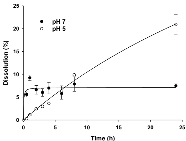
Fig. 2. Dissolution of Cu-NPs (% of measured total Cu) in dechlorinated Plymouth tap water adjusted to pH 7 (closed symbols) and 5 (open symbols) over 24 h. Data are means \pm S.E.M., n = 3 replicates. Curves for dissolved Cu concentration were fitted by using a rectangular hyperbole function (one site, ligand binding to saturation) in SigmaPlot v. 13. The Cu concentrations in controls (no Cu-NPs, dialysis tubing only) were below the instrument detection limits and are not shown.
