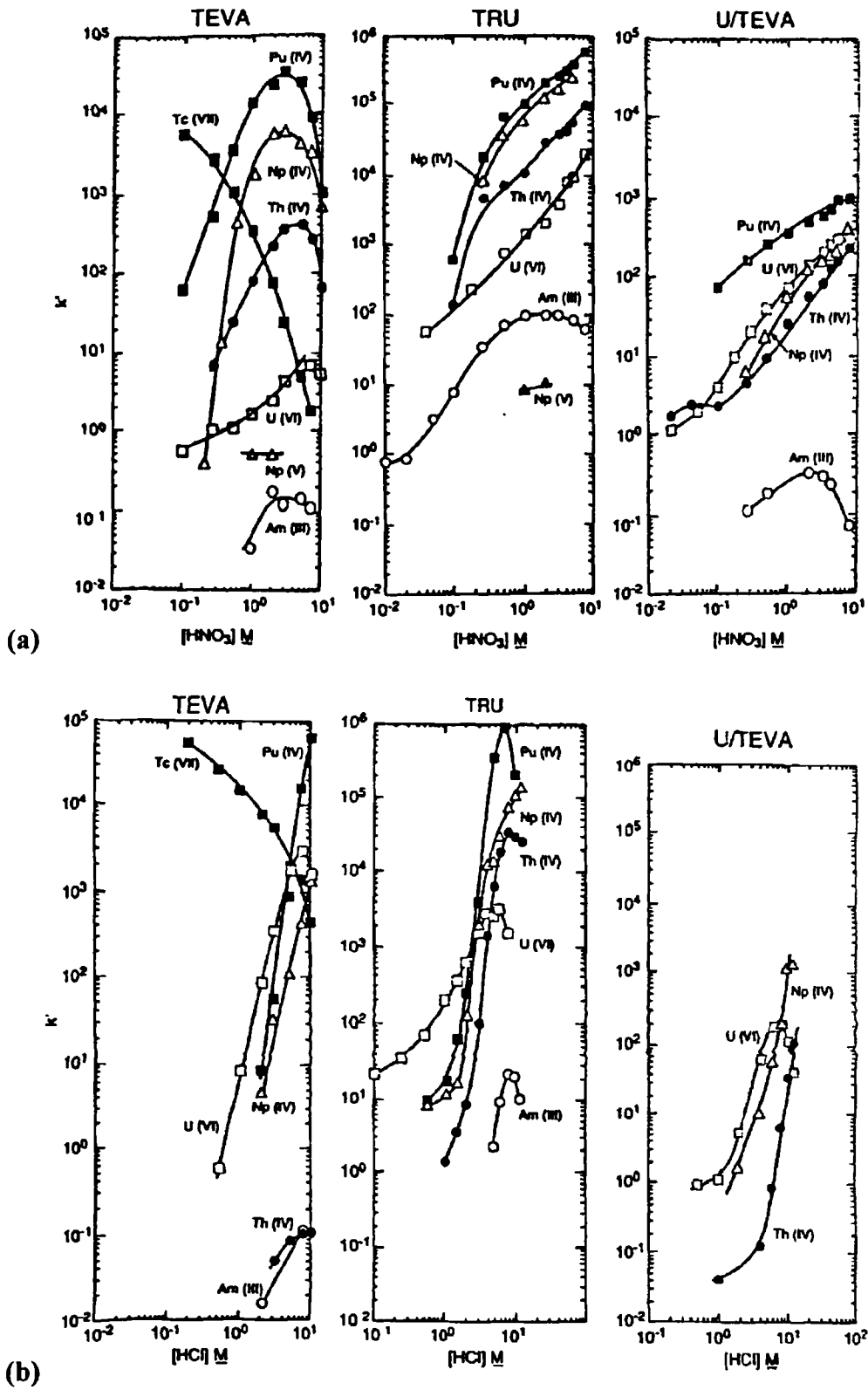
Figure 1.6 (a) Nitric acid and (b) hydrochloric acid dependency of k' for actinides at 23–25°C 79
