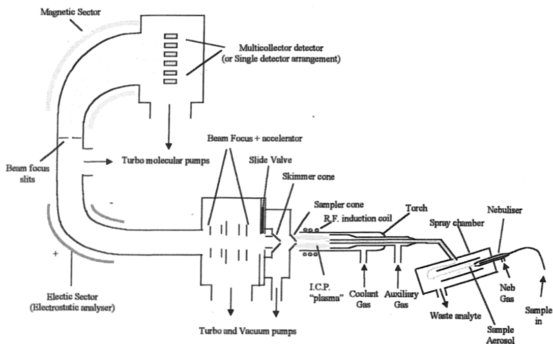
Figure 1.3 Generalised layout for a double-focusing Sector Field ICP-MS instrument, with a multi-collector detector arrangement
