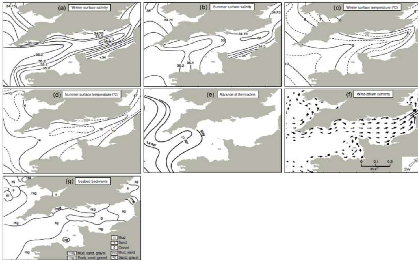
Figure 2. A summary of the physical oceanography and sedimentology of the English Channel. (a) winter surface salinity, (b) summer surface salinity, (c) winter surface temperature, (d) summer surface temperature, (e) temporal advance of the seasonal thermocline (f) residual currents for a southwest wind (arrows representing residual velocities of < 0.01 \text{ m s}^{-1} have been omitted) and (g) distribution of surficial seabed sediment types (from Uncles and Stephens, 2007).
