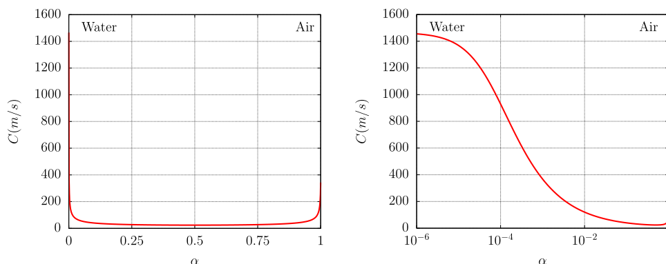
FIG. 1. The speed of sound in water-air mixture at one atmospheric pressure and 15 °C. 30 \alpha indicates the volume fraction of air in the mixture. Left: normal scale; right: log scale.
