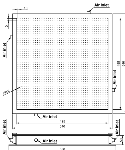
FIG. 3. The bubble generator (units in mm).
