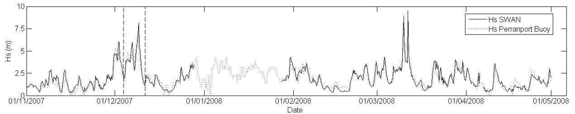
Figure 5: Time series of simulated ( H_{s,SWAN} ) and measured ( H_{s,buoy} ) significant wave height to validate the high resolution wave propagation model. The storm conditions studied (from 5 Dec 2007, 00:00 UTC; to 10 Dec 2007, 18:00 UTC) to assess the impact of the wave farm are highlighted.
