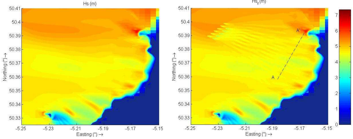
Figure 6: Significant wave height in the baseline scenario ( H_s ) and with the wave farm ( H_{sf} ) at the first peak of the storm studied (5 Dec 2007, 18:00 UTC). [Deep water wave conditions: H_{s0} = 6.89 m, T_p = 15.64 s, \theta_p = 268.45^\circ ]. The line AA' is shown.
