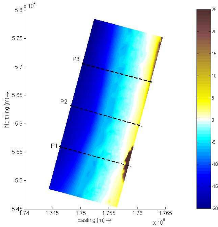
Figure 2: Bathymetry of Perranporth Beach for the coastal processes model. Profiles P1, P2 and P3 included. Water depth in relation to local chart datum [in m].
