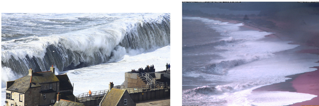
Figure 2. Left panel shows huge, parallel-incident storm waves (estimated breaking wave height of 8 m) breaking right at the base of the gravel beach at the southeastern end of Chesil Beach, Dorset, UK, during the storm of 05/02/2013 (photo by Richard Broome, reproduced with permission). Right panel shows very large, obliquely-incident storm waves (estimated breaking wave height of 4 m) on Slapton Sands, south Devon, also during the storm of 05/02/2015 (photo represents a video snapshot from the ARGUS camera station deployed at the northern end of Slapton Sands). This figure is available in colour online at wileyonlinelibrary.com/journal/espl
