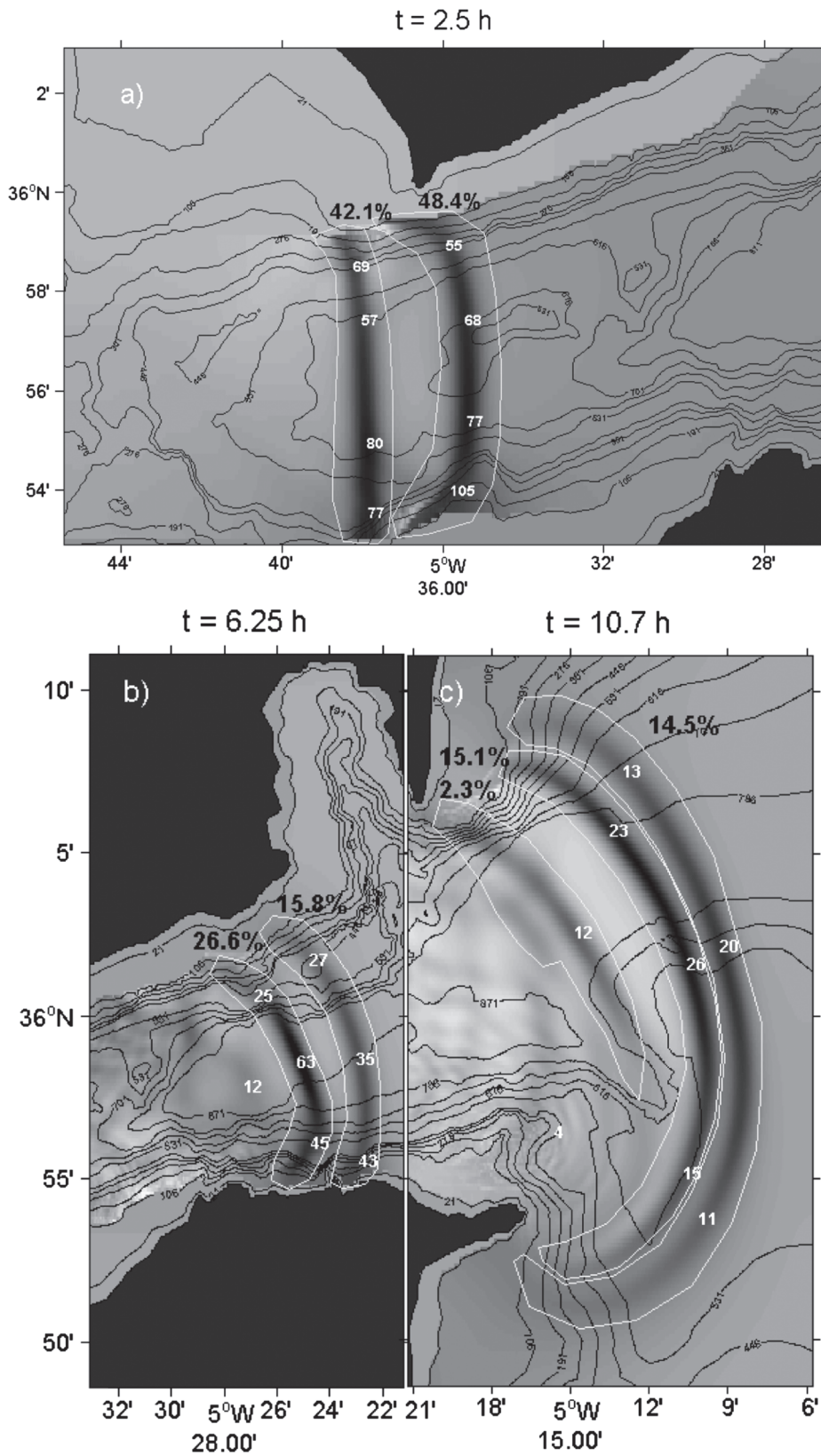
FIG. 11. As in Fig. 4, but for two propagating LAIWs with initial amplitudes of 83 and 73 m for the first and second waves, respectively.
