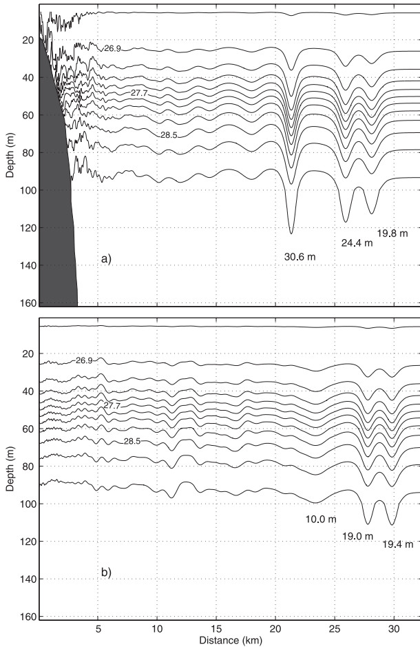
FIG. 14. (a) Zonal cross section of density along 36°3.7'N (see Fig. 13c) showing a non-rank-ordered system of LAIW propagating eastward into the Alboran Sea. (b) A similar cross section along 35°57.9'N showing a well-rank-ordered system of LAIW.
