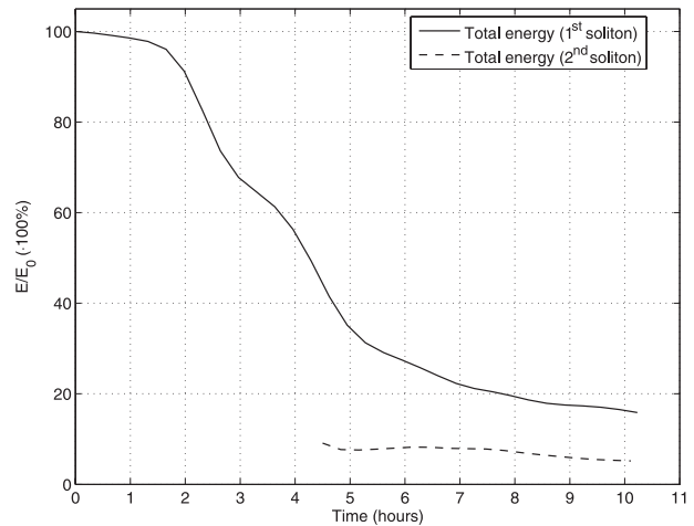
FIG. 5. Time evolution of the total energy of the leading LAIW (solid line) and the generated secondary internal solitary wave (dashed line) normalized by the energy of the initial LAIW. The energy calculation procedure is explained in Fig. 4 and appendix A. The energy of the secondary wave was calculated for t > 4.5 h when its shape was clearly identified as a quasi-2D propagating wave.
