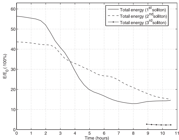
FIG. 12. Time evolution of the total energy of the leading and second LAIW (solid and dashed lines, respectively) as well as the generated secondary internal solitary wave (dotted line), normalized by the energy of the two initial LAIW.
