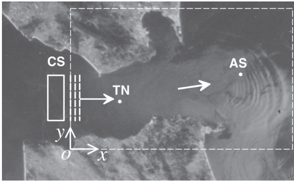
FIG. 1. Sea surface manifestation of a wave packet of LAIW s propagating from the strait toward the Alboran Sea [courtesy of the European Space Agency (ESA)]: CS is Camarinal Sill; TN and AS denote the locations of the moorings deployed at Tarifa Narrow and in the Alboran Sea.
