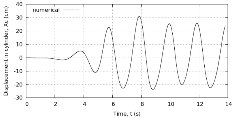
Figure 5.38: Numerical results for the displacement in the cylinder of the Wavestar device with the PTO disabled and when subject to extreme regular waves (RExt01)
