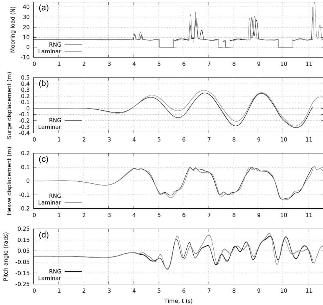
Figure 5.52: Results from numerical simulation of the Seabased wave energy generator in regular waves with the RNG k-\varepsilon model (black) or laminar flow (grey). (a) mooring load, (b) surge displacement, (c) heave displacement, and (d) pitch angle.
