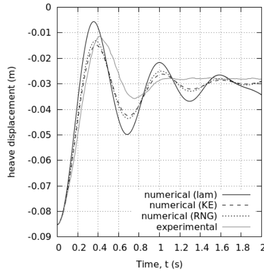
Figure 5.50: Comparisons between the heave displacement of the Seabased float in a physical and equivalent numerical decay test with either a k-\varepsilon , RNG k-\varepsilon or no turbulence (laminar) model implemented
