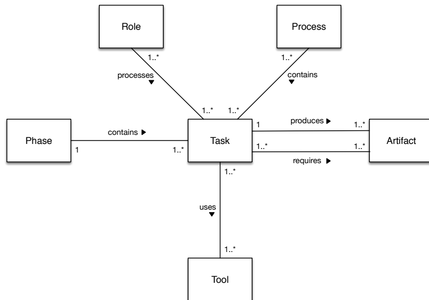
Figure 58: Metamodel
