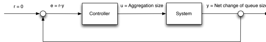
Figure 41: Feedback loop to control the aggregation size
