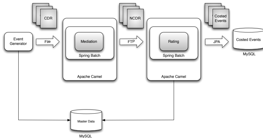
Figure 22: Batch prototype
