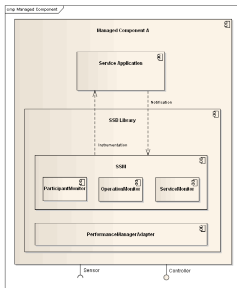
Figure 10: Managed Component
