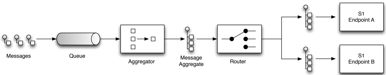
Figure 7. Middleware components
