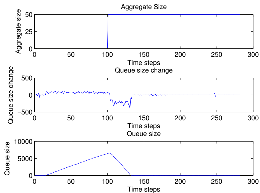
Figure 53: Step test
