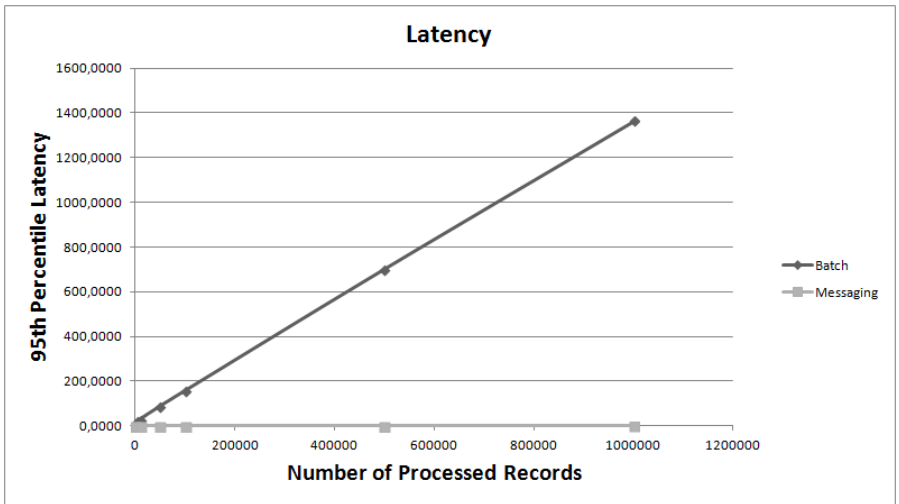
Figure 30: Latency
