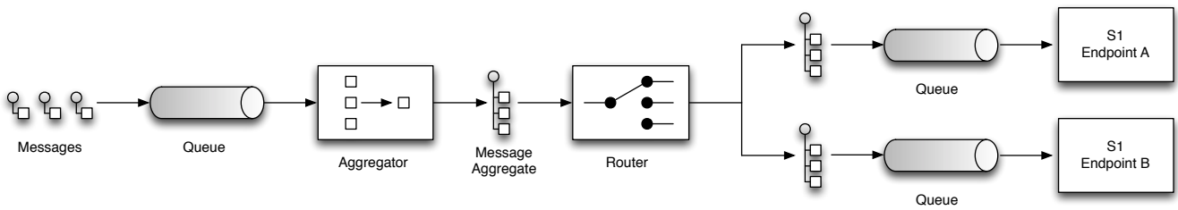
Figure 2. Overview of the adaptive middleware for bulk data processing [2]
