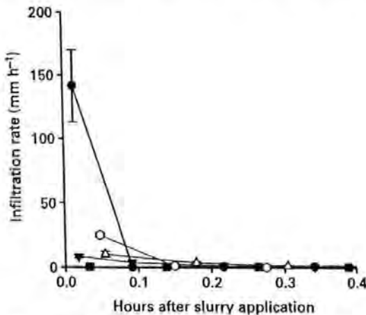
Figure 3. Infiltration rates for cattle slurries of varying DM content applied to sandy clay loam at 40 cm soil water tension. Slurry DM contents: 1.7% (●), 2.4% (○), 3.8% (▼), 4.8% (Δ) and 7.1% (■). Error bars show \pm 1 standard error of the mean ( n = 3 ).
