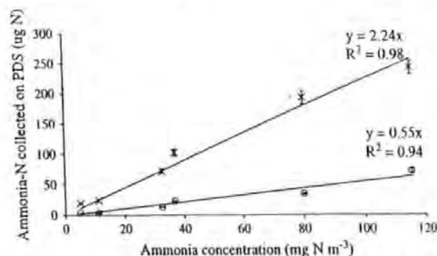
Fig. 3. Amount of ammonia-N ( \mu\text{g} ) collected on L-type (x) and C-type (o) PDS at different chamber ammonia concentrations ( \text{mg N m}^{-3} , as measured using absorption flasks), together with fitted regression lines. Error bars show \pm 1 standard error.
