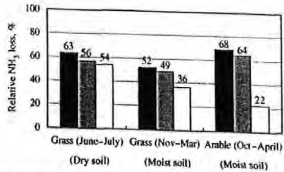
Fig. 4. Ammonia emissions following slurry application by surface placement techniques relative to splash-plate application: ■, bandspray; ▨, trailing shoe; □, shallow injection
