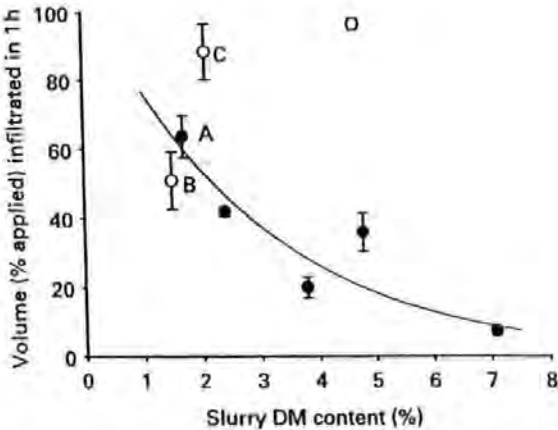
Figure 4. Influence of slurry DM content on infiltration volume. Data for cattle slurry (●) and pig slurry (○) and fitted line for cattle slurry. Error bars show \pm 1 standard error of the mean ( n = 3 ). Data points A, B and C are considered to be underestimates (see text).
