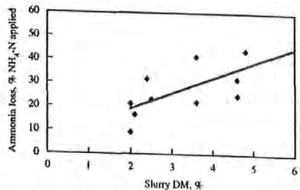
Fig. 5. Effect of slurry dry matter content (DM) on ammonia loss, splash-plate treatments; % loss(NH 4 -N) = 6.17 (DM) + 6.70, r^2 = 0.44 , P < 0.01 ; r^2 , coefficient of determination; P , probability; DM, slurry dry matter
