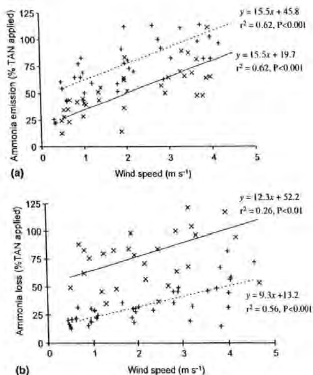
Fig. 1. Influence of wind speed on ammonia emission from (a) cattle slurry applied to grassland ((x) site 1, (+) site 2, (solid line) fitted site 1, (dashed line) fitted site 2); (b) pig slurry applied to cereal stubble ((x) site 3, (+) site 5, (solid line) fitted site 3, (dashed line) fitted site 5).
