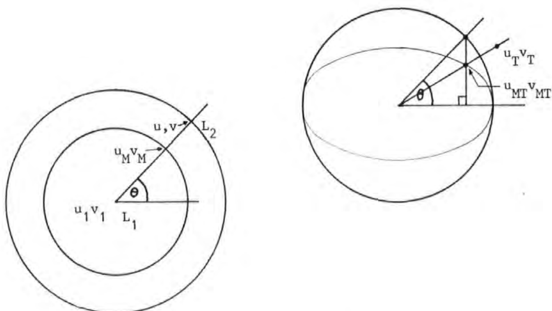
Fig. 3.42 Transformation for colours not lying on the hue circle.
