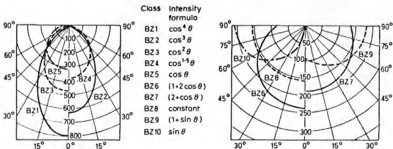
Fig. 2.04 Polar distributions for various BZ classifications.
