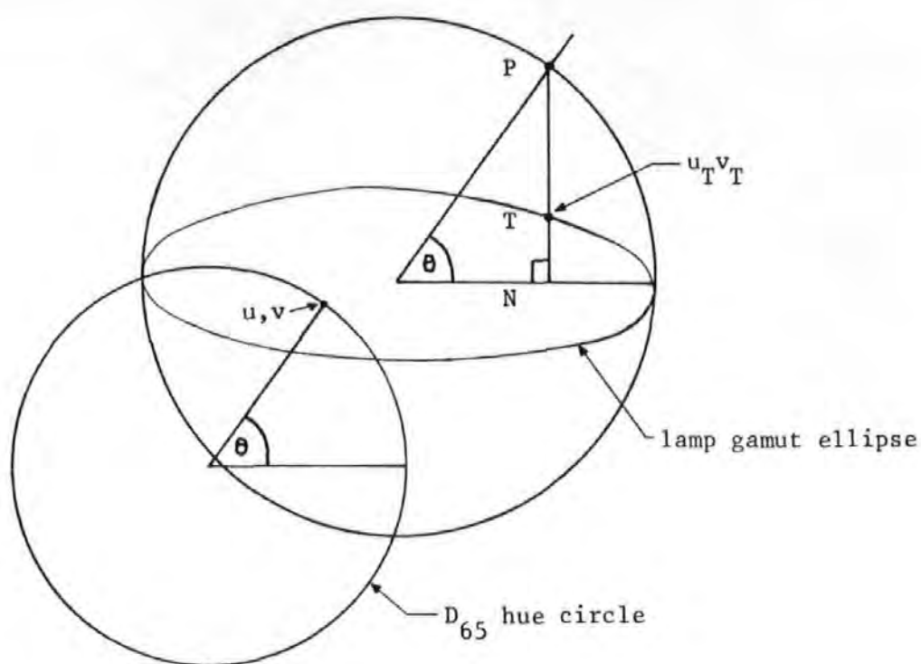
Fig. 3.41 The basic colour transformation.
