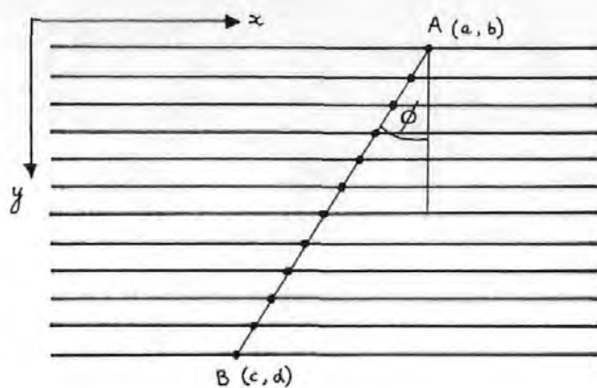
Fig. 4.05 Generation of a line segment with non-interlaced scan.
