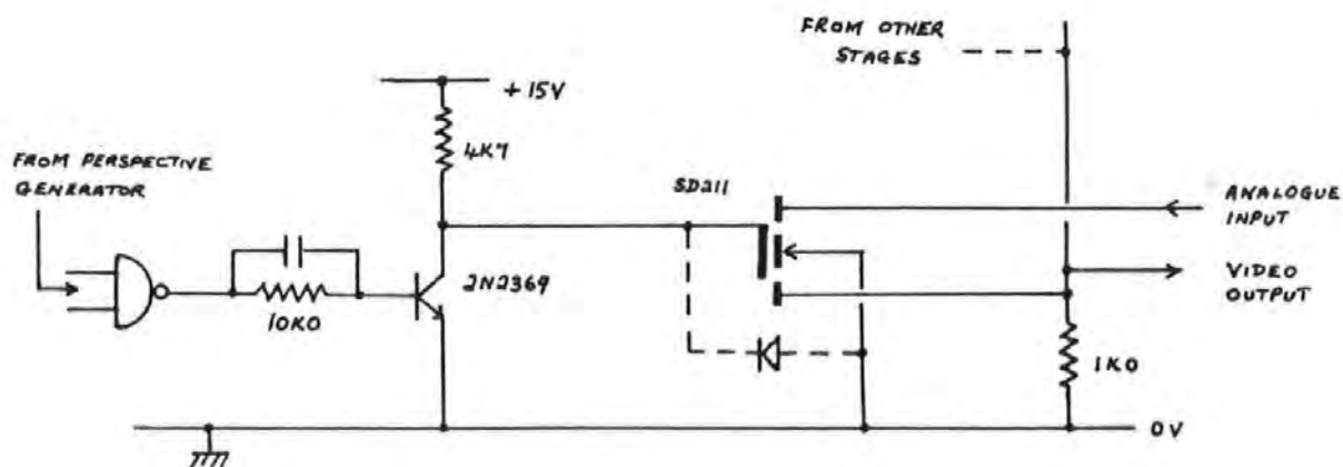
Fig 4.18 Analogue switching circuitry with TTL interfacing.
