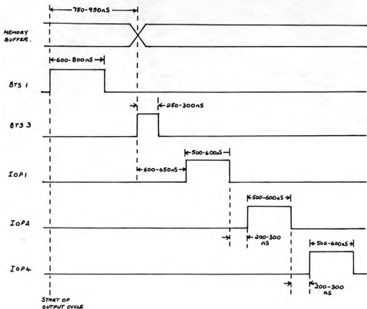
Fig. 4.22 Timing signals available to device interfaces from the PDP8 output bus.
