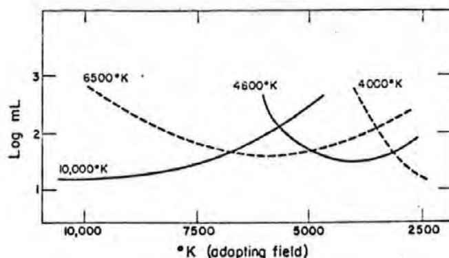
Fig. 5.01 Luminance thresholds for a white sensation as a function of colour temperature for various adapting illuminant colours (1 second stimulus with an 11.7° target).
