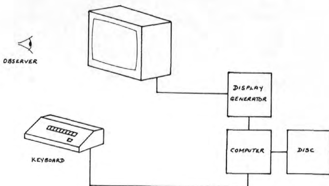
Fig. 5.04 Experimental arrangement for measurement of the achromatic point.
