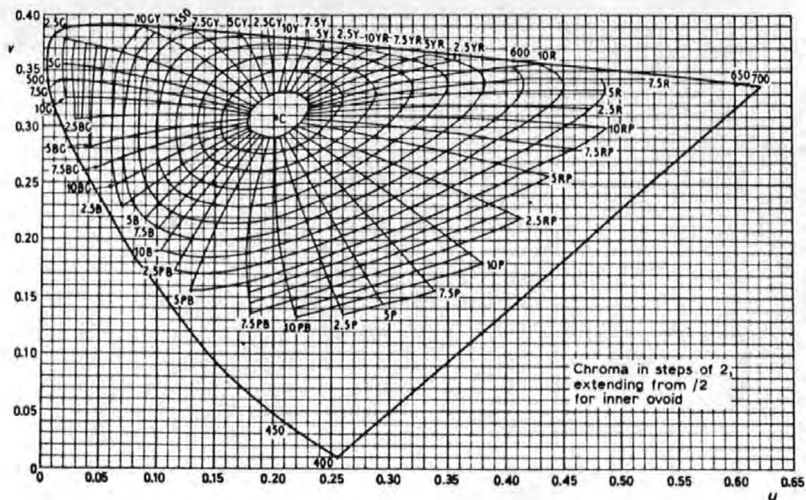
Fig. 3.08(a) Loci of constant Munsell renotation hue and chroma (value = 4) in the C.I.E. UCS diagram.
