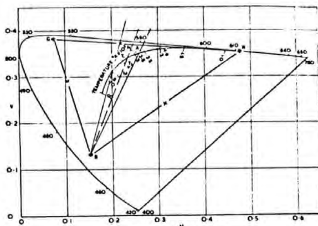
Fig. 5.02 Construction to find the best approximation to reference white points, matching illuminants A and C by adjusting only the level of the blue display primary.
