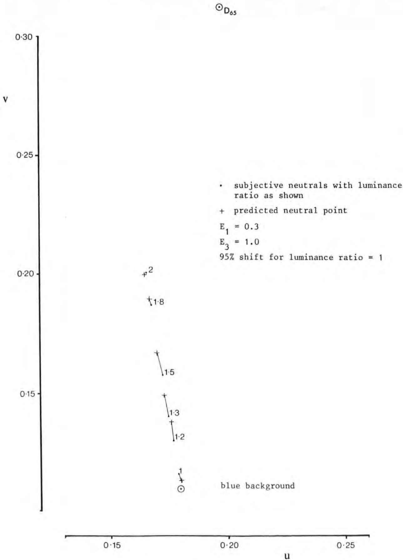
Fig. 5.15c Subjective neutral points for varying luminance ratio with a blue background of luminance 25 \text{ cd/m}^2 .
