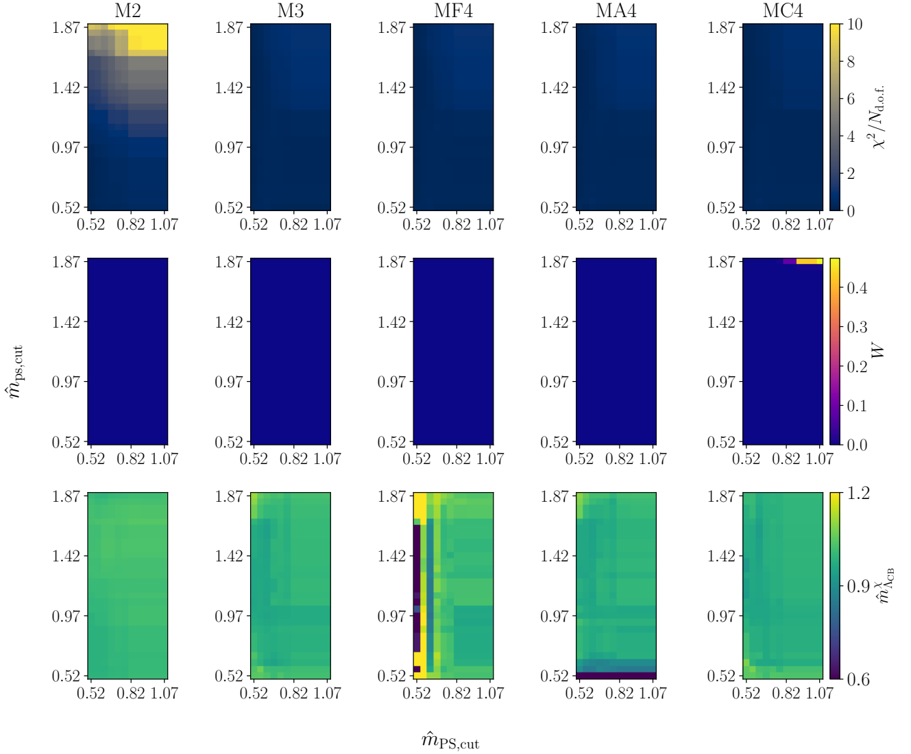
FIG. 6: Heat-map plots of \chi^2/N_{\text{d.o.f.}} , W and \hat{m}_{\text{CB}}^\chi (top to bottom) for the analysis of \hat{m}_{\Lambda_{\text{CB}}} using different fit ansatz in Tab. 3. The horizontal and vertical axes are \hat{m}_{\text{PS,cut}} and \hat{m}_{\text{ps,cut}} , respectively.
