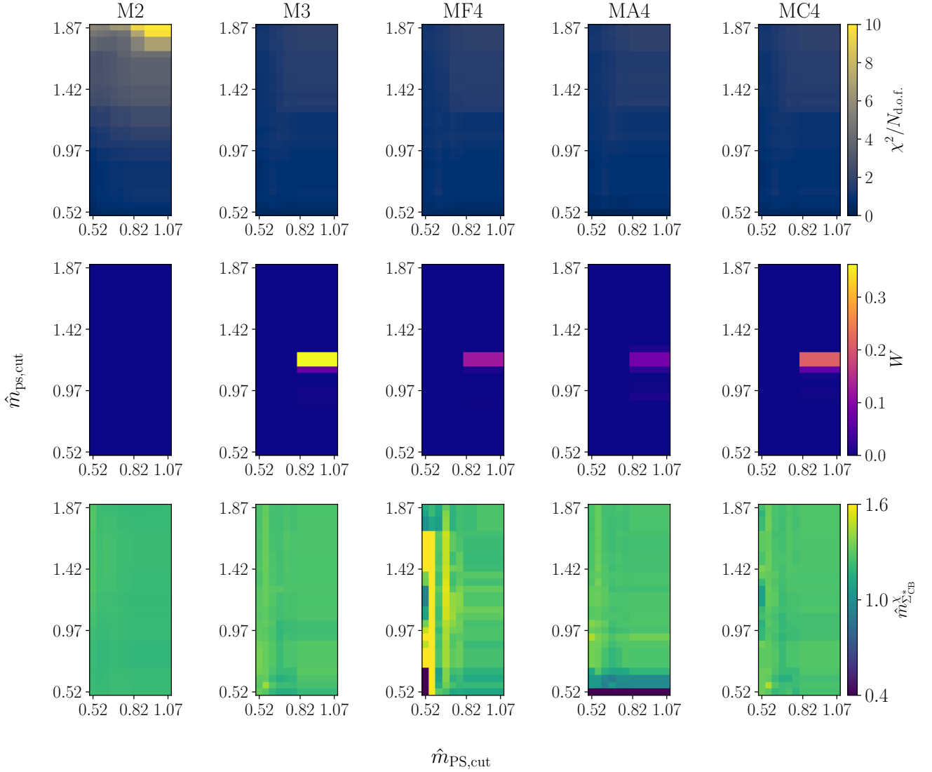
FIG. 8: Heat-map plots of \chi^2/N_{\text{d.o.f.}} , W and \hat{m}_{\Sigma_{\text{CB}}}^x (top to bottom) for the analysis of \hat{m}_{\Sigma_{\text{CB}}}^* using different fit ansatz in Tab. 3. The horizontal and vertical axes are \hat{m}_{\text{PS,cut}} and \hat{m}_{\text{ps,cut}} , respectively.
