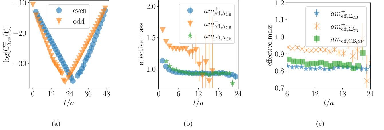
FIG. 1: Illustrative examples of chimera baryon correlation functions, (a), and effective mass plots, (b) and (c), obtained on the ensemble QB1 with hyperquark masses am_0^{(f)} = -0.77 and am_0^{(as)} = -1.05 . (a): the parity-projected correlators, C_{\Lambda_{CB}}^{\pm}(t) . (b) effective masses, am_{\text{eff}} , extracted from correlation function obtained with, C_{\Lambda_{CB}}^{\pm}(t) , and without parity projection, C_{\Lambda_{CB}}(t) . (c): effective masses, am_{\text{eff}} , extracted from correlation functions upon which spin and parity projections are applied, C_{\Sigma_{CB}}^+(t) and C_{\Sigma_{CB}^*}^+(t) , or without any projection, C_{CB, \mu\nu}(t) .
