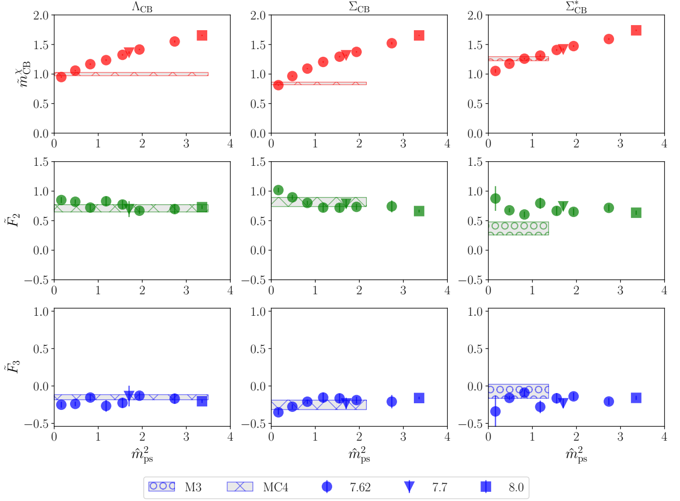
FIG. 9: Result of the cross checks based upon Eq. (32). The horizontal axis denotes the value of \hat{m}_{ps} . As indicated in the legend below the plots, different markers stand for measurements performed on different ensembles, and the bands represent results of \hat{m}_{CB}^\chi , F_2 and F_3 from the best global-fit analysis procedures (see Tab. 7). The height and the width of each band correspond to the size of the statistical error and the value of \hat{m}_{ps,cut} , respectively.
