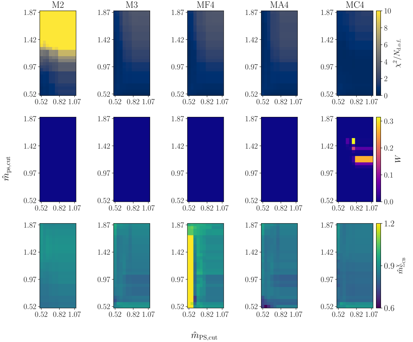
FIG. 7: Heat-map plots of \chi^2/N_{\text{d.o.f.}} , W and \hat{m}_{\Sigma_{CB}}^{\chi} (top to bottom) for the analysis of \hat{m}_{\Sigma_{CB}} using different fit ansätze in Tab. 3. The horizontal and vertical axes are \hat{m}_{PS,cut} and \hat{m}_{ps,cut} , respectively.
