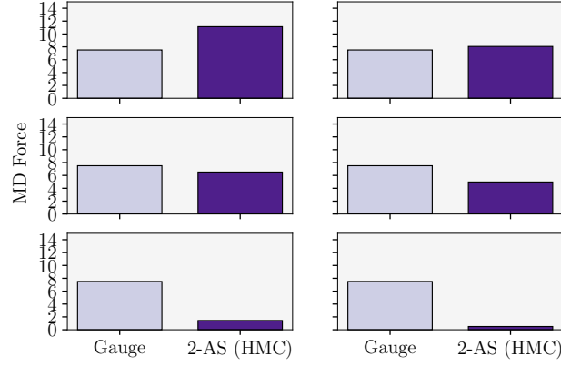
Figure 3: Field contribution to the MD force for the theory with N = 2 , N_f = 0 , and N_{as} = 4 , on isotropic lattice with \tilde{V} = (8a)^4 , and lattice coupling \beta = 6.8 . The two blocks are respectively indicating the gauge (light shading, left) and the fermion (dark shading, right) contribution. Fermion contributions are summed over flavor. The six panels correspond to different choices of bare mass: am_0^{as} = -0.9, -0.1, +0.6, +1.8, +15, +50 (left to right, top to bottom). The results are normalised so that the gauge contribution is held constant. The computation of the force contributions is made in Ref. [16]. (Figure taken from Ref. [17]).
