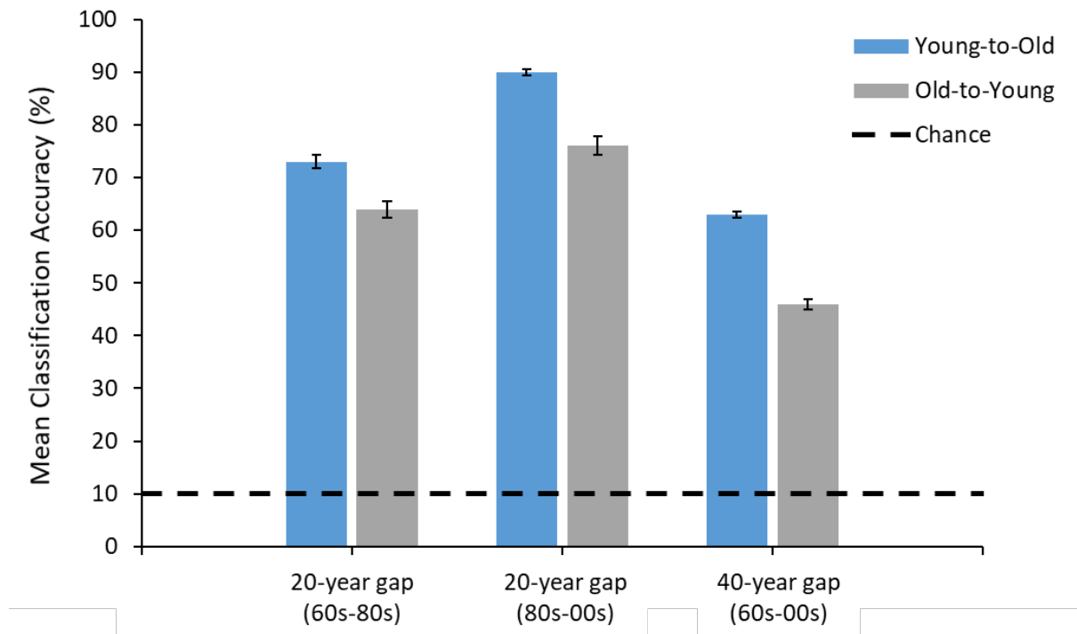
Figure 2: Mean PCA+LDA classification accuracy for young-to-old and old-to-young generalisation at three different age gaps between the training and test images. Dashed line represents chance classification performance and error bars show the standard error across the 49 iterations of the classification procedure.
