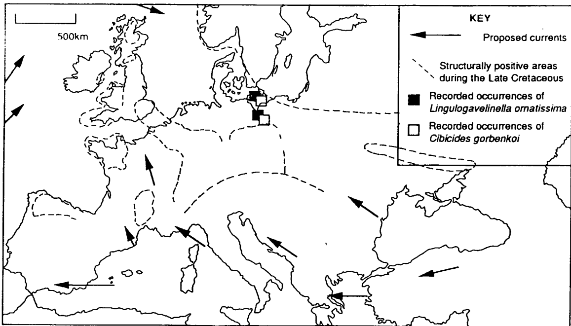
Figure 5.11. The European distribution of Lingulogavelinella ornatissima and Cibicides gorbekoi . (Base map and current patterns based on Bailey and Hart 1979.)
