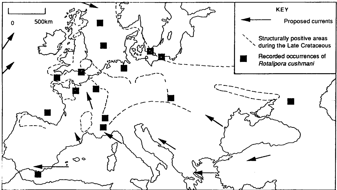
Figure 5.5. The European distribution of Rotalipora cushmani . (Base map and current patterns based on Bailey and Hart 1979.)
