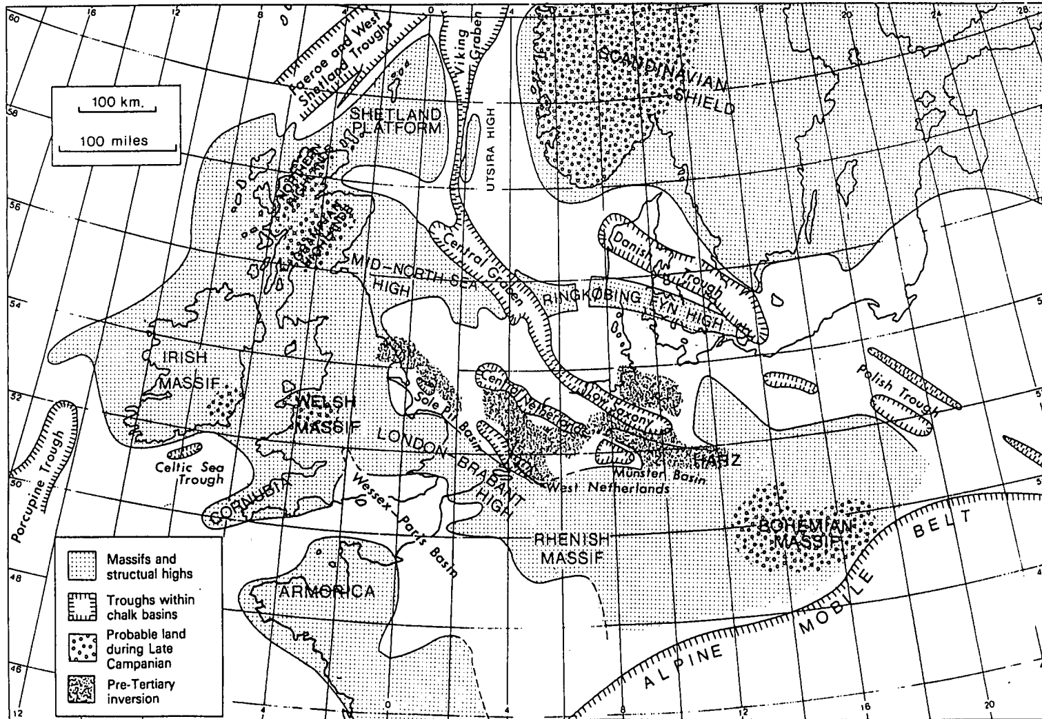
Figure 5.3 Geological setting of the Upper Cretaceous in north-west Europe (Reproduced from Hancock, 1984).
