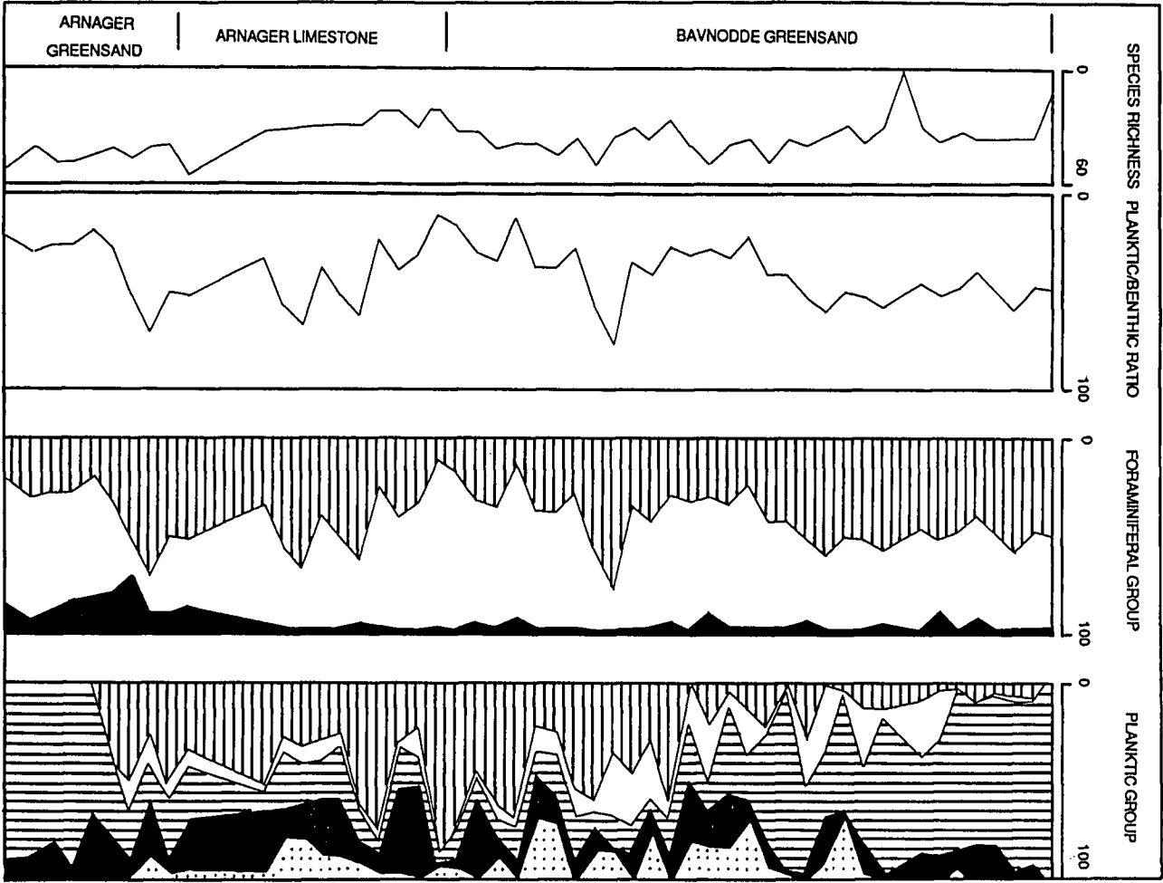
Figure 5. 1 Distribution of foraminiferal groups, richness and planktic / benthic ratio for the Arnager Greensand, Arnager Limestone and Bavnodde Greensand, from coastal exposures.
