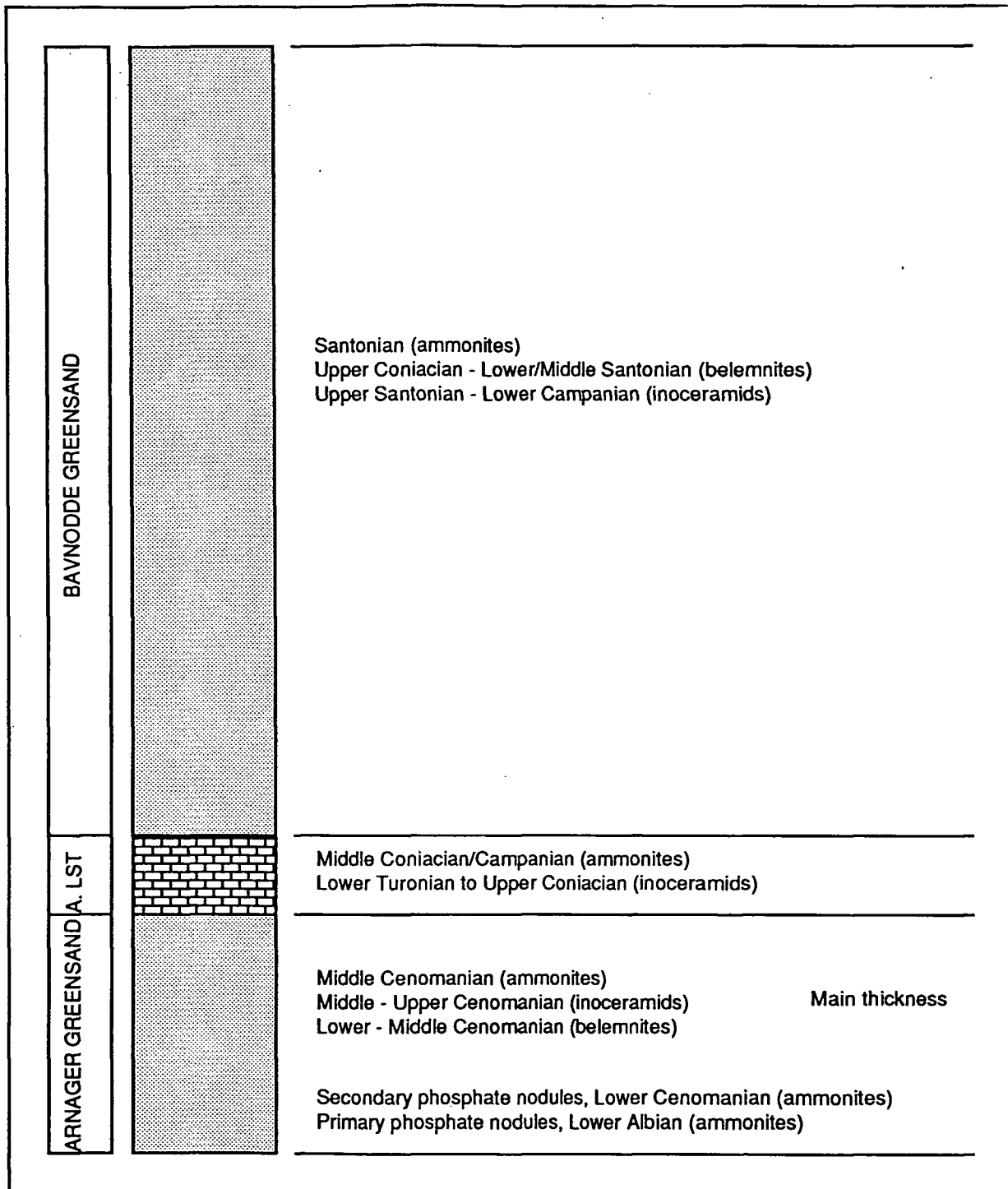
Figure 2.2 Macrofaunal evidence for the age of the Arnager Greensand, Arnager Limestone and Bavnodde Greensand, Bornholm, Denmark. Primary source Christensen (1984)
