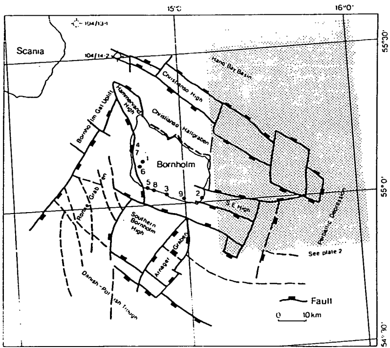
Major structural elements of the Bornholm area (Vejbæk, 1985).
