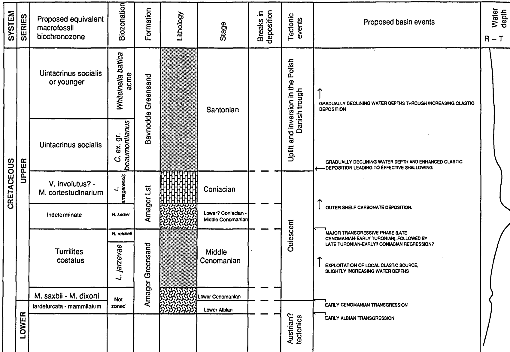
Figure 6.4 Proposed event synthesis for the Bornholm marine Cretaceous succession.
