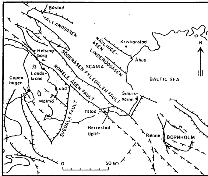
Main structural trends in southern Scandinavia (Christensen, 1984)
