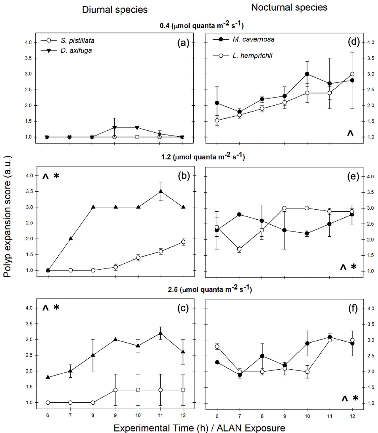
Fig. 4. The effect of exposure to fixed ALAN intensities (0.4, 1.2 and 2.5 \mu\text{mol quanta m}^{-2} \text{s}^{-1} ) on the polyp and tentacle expansion behaviour of diurnal and nocturnal corals during 6-hours of exposure during the night hours of isolated days. Data points show the means of corresponding timepoints collected on 4 different measuring days ( n = 4 ). Error bars denote means of \pm SD. (a–c) diurnal species ( S. pistillata , D. axifuga ). (d–f) nocturnal species ( M. cavernosa , L. hemprichii ). Polyp expansion scores refer to Table 1. Symbols represent GLMM significance at the 0.05 probability level for ALAN treatments ( \wedge ) and (*) coral species fixed effects.
