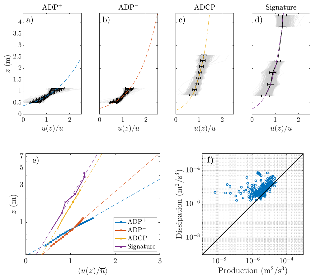
Figure 3. (a)–(d) In gray, velocity profiles of u(z) normalized by the mean velocity \bar{u} for all profiles where R^2 \geq 0.8 are shown. The black error bars show the time-averaged value and one standard deviation of each vertical bin. The dashed lines are the log profiles based on a best fit of the time-averaged profiles. Figures (a) and (b) show the ADP profiles when flow is directed north and south, respectively. (e) Time-averaged profiles and best fit as in (a)–(d), here on a logarithmic scale. (f) Dissipation of TKE as derived from the ADV and production of TKE as derived from the ADV and ADP.
