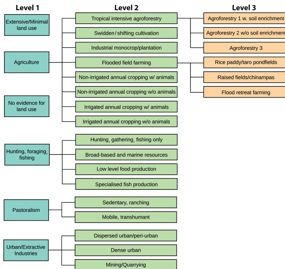
Figure 2: The LandCover6k land-use classification matrix.
