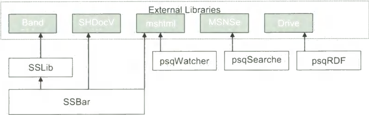
Figure 12: Interaction with external libraries
