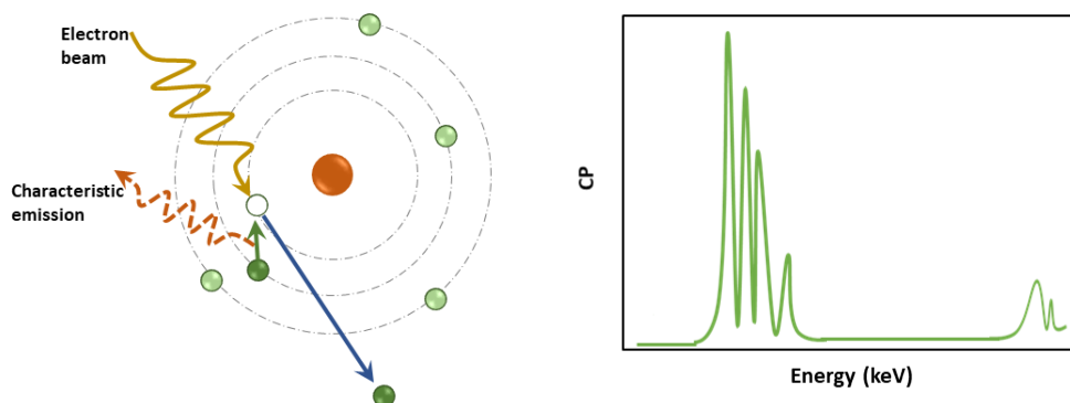
Figure 2.10: A schematic of the working principle of EDS where an electron is shifted from its orbit and an electron from a higher energy shell fills the electron hole, resulting in an X-ray emission (left). A sample spectrum of EDS (right).
