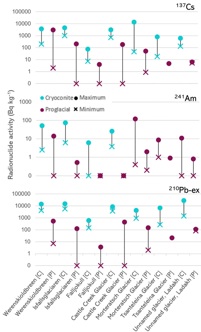
Fig. 5. The range (minimum and maximum) of ^{137}\text{Cs} , ^{241}\text{Am} , and ^{210}\text{Pb-ex} activities recorded in selected cryoconite [C], and proglacial soil / sediment [P] samples. Note that logarithmic scales and different scale ranges are used due to large variability in activity values.
