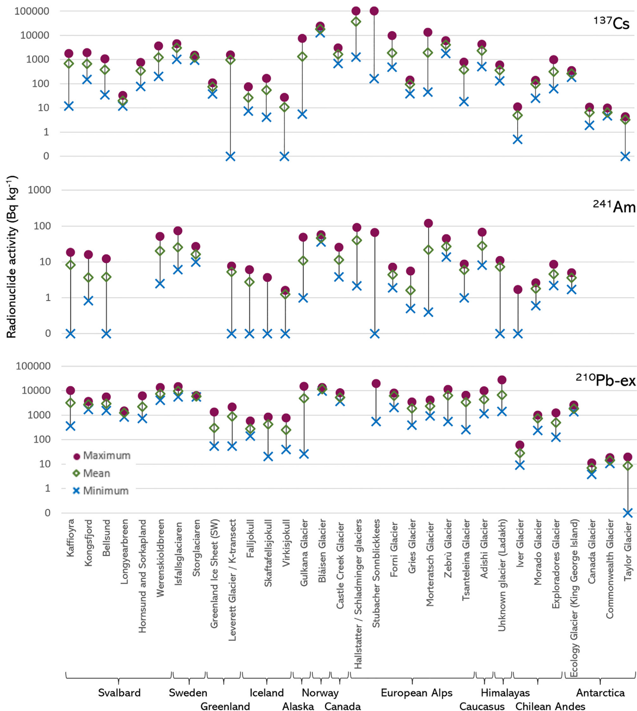
Fig. 2. The range and mean values of ^{137}\text{Cs} , ^{241}\text{Am} , and ^{210}\text{Pb-ex} activities recorded in cryoconite samples from across the global cryosphere - see Table A1 for data. Note that logarithmic scales and different scale ranges are used due to the large variability in activity values. Data are presented in latitudinal order from north to south.
