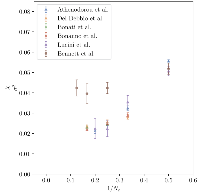
Fig. 1. Topological susceptibility \chi , in units of the string tension \sigma , in the continuum limit, for various groups SU(N_c) and Sp(N_c) , and as a function of the parameter 1/N_c . The measurements reported here are labelled by the collaboration that published them, and are also summarised in Table 1.
