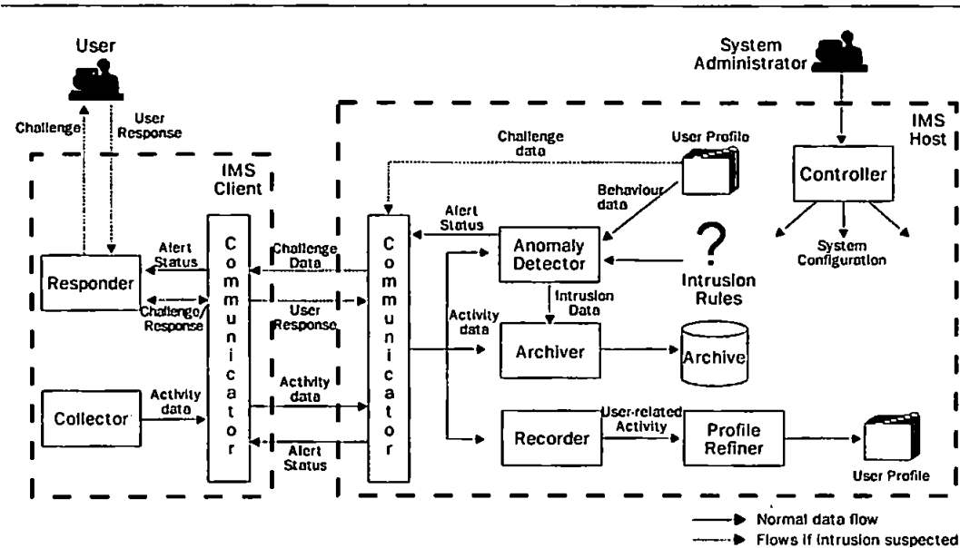
Figure 1 IMS architecture
