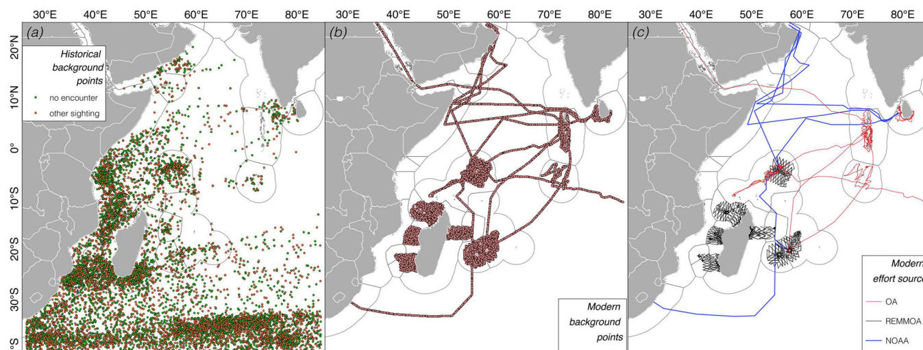
FIGURE 2 Background points for (a) historical and (b) modern Maxent models of whale sightings. Historical background points refer to position of whaling vessel days on which no whales were sighted (no encounter) and for sightings other than sperm whales (other sighting) (data from Census of Marine Life [Smith et al., 2012]). Scientific survey effort (c) associated with modern records (OA, Ocean Alliance [de Vos et al., 2012; Wise et al., 2009]; REMMOA, Census of marine mammals and other pelagic megafauna by aerial survey [Mannocci et al., 2013, 2015]; NOAA, National Oceanic and Atmospheric Administration [Balance & Pitman 1996; Ballance et al., 1998, 2001]). See Appendices S3 and S5 for references.
