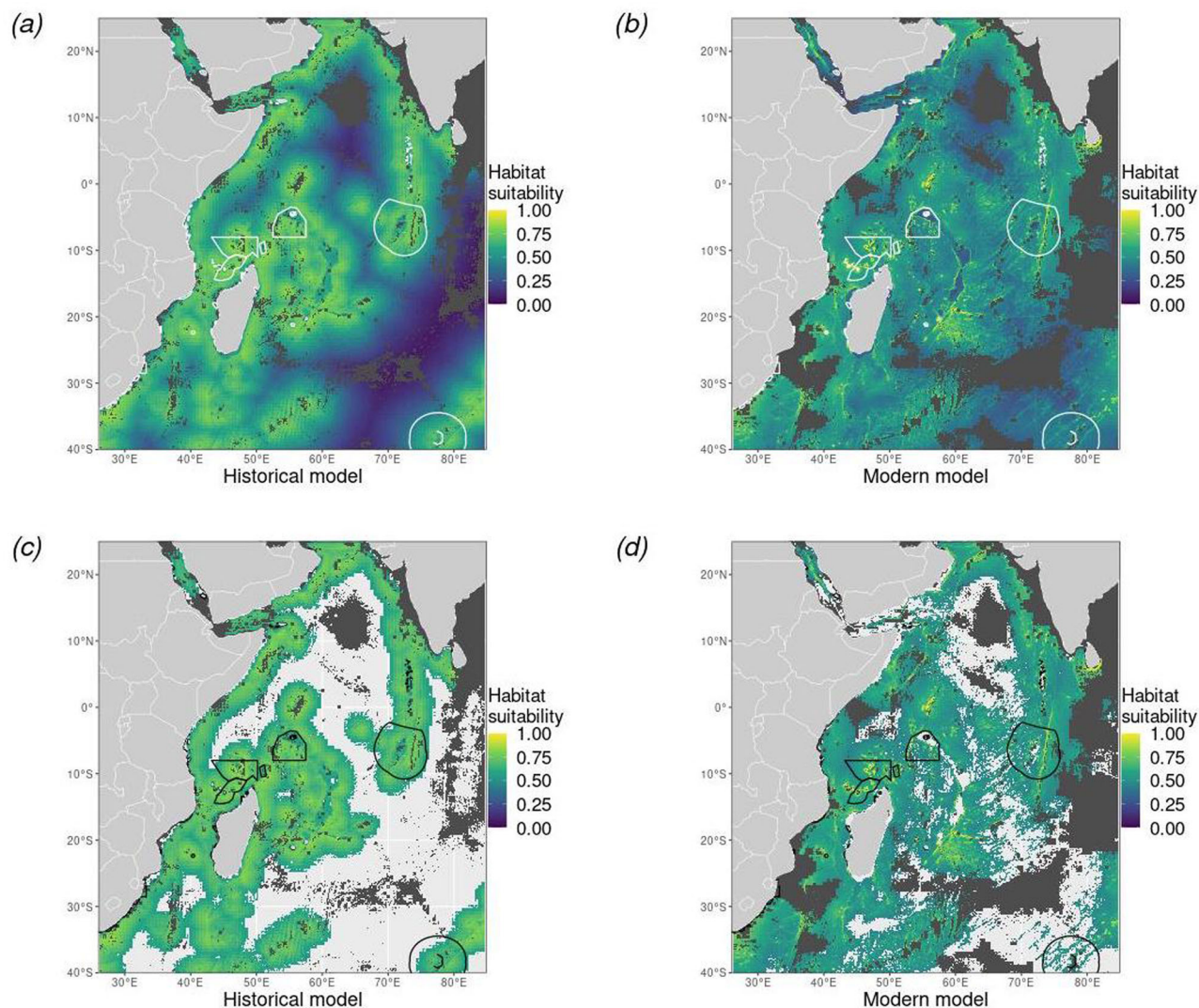
FIGURE 5 Sperm whale relative habitat suitability predictions for (a) historical and (b) modern models with MPA locations overlaid (IUCN-UNEP, 2021) and locations of high predicted relative habitat suitability (above the threshold set by maximizing the sum of sensitivity and specificity following the recommendations of Liu et al. [2013]) for (c) historical and (d) modern models (gray, areas of extrapolated environmental space where predictions should be considered unreliable).
