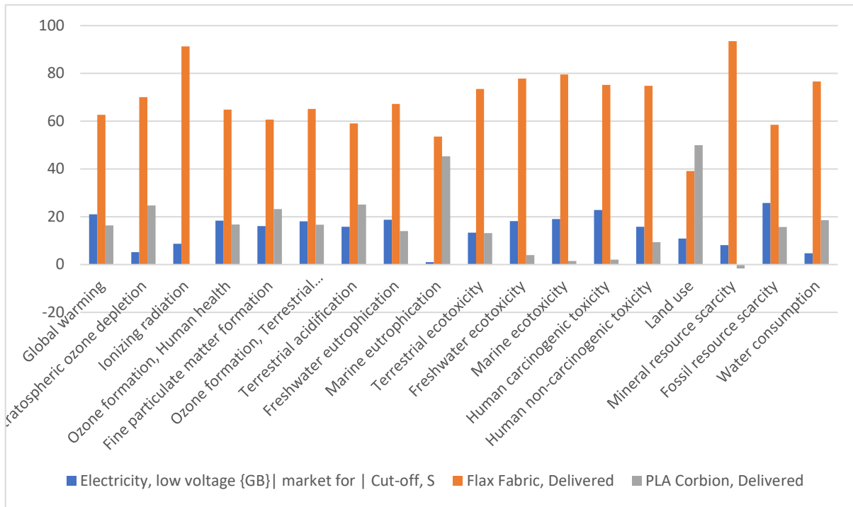
Figure 0.12: Relative Contribution of Flax PLA, FVf 0.6 Composite
