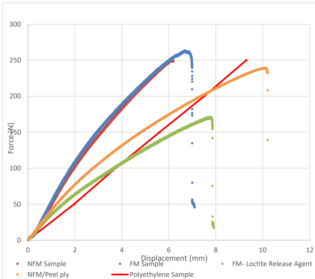
Figure F9: Force displacement curves for the flax/epoxy composites
