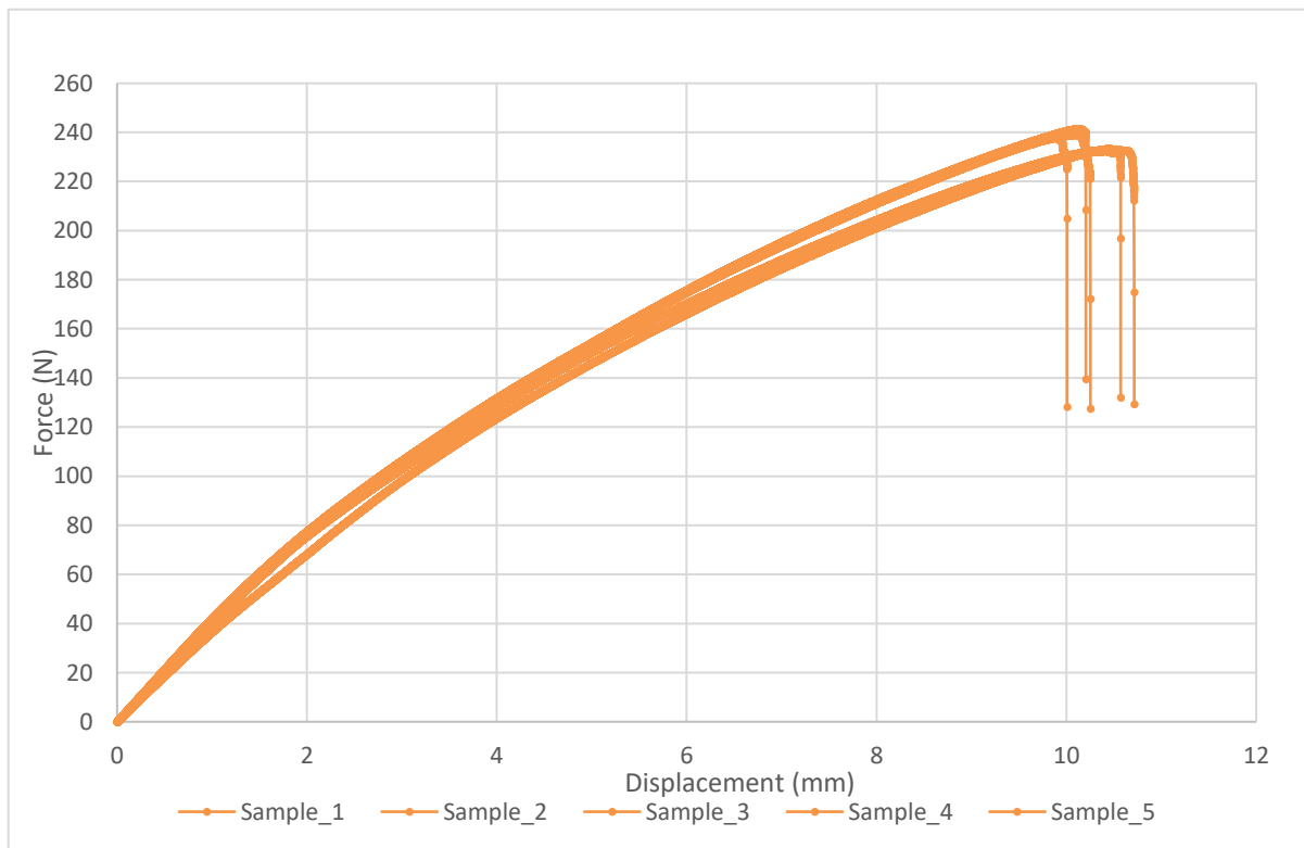
Figure F8: Flax/Epoxy NFM/PP Samples Force Displacement Graph
